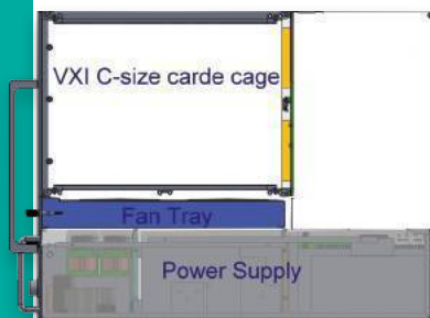
Schematic View 10U VXI6025 chassis
