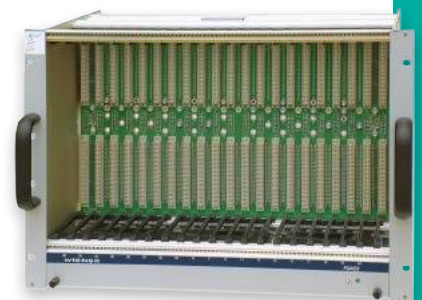
6U VME NIX-I Crate
