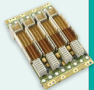
3U CompactPCI-Serial backplane
