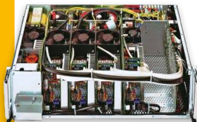
PL508 inside
