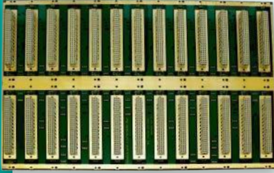
13 slot 6U VXI bus (C-size)
