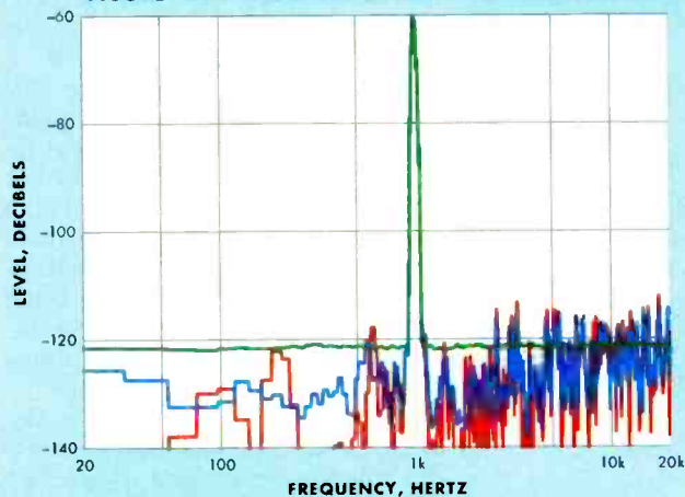
FIGURE 1: DITHERED VS. UNDITHERED TEST SIGNALS
