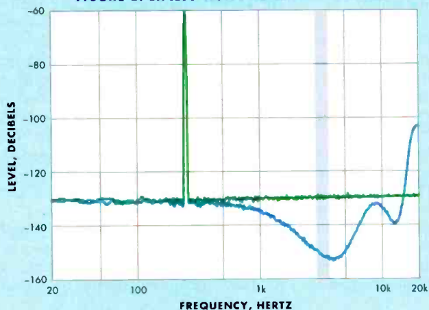
FIGURE 2: EXCESS-NOISE REFERENCE SPECTRA
