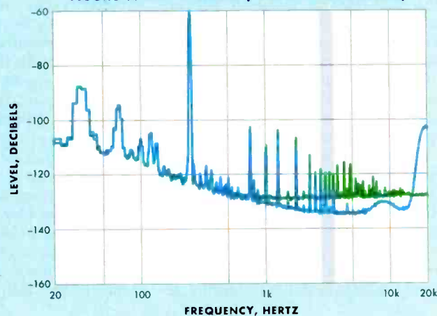
FIGURE 3: EXCESS NOISE (ANALOG DAT OUTPUT)
