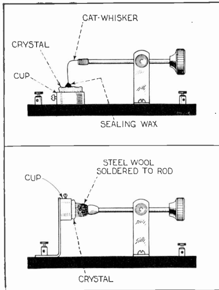
Upper: A drop of wax will hold the cat-whisker on a sensitive spot. Lower: Steel wool makes an excellent substitute for a cat-whisker.
