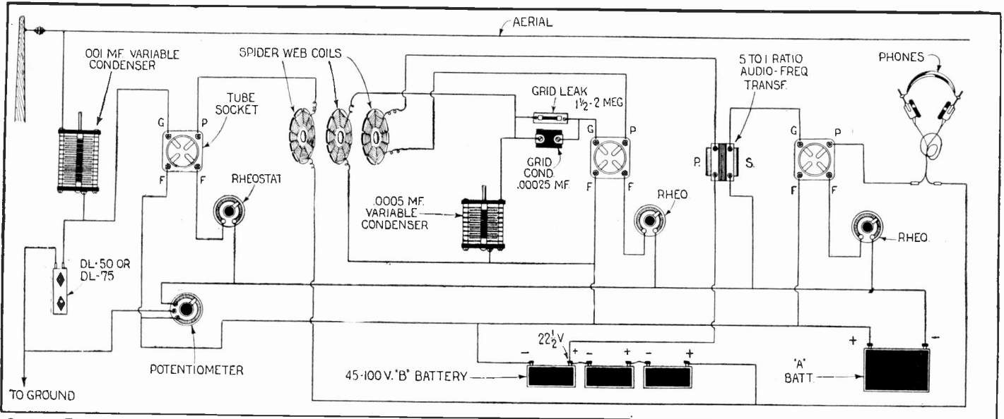
Q. 201. The circuit diagram of a radio receiving set employing one stage of tuned radio frequency amplification, a vacuum tube detector and one stage of audio frequency amplification, appears above. The tickler coil pro-
