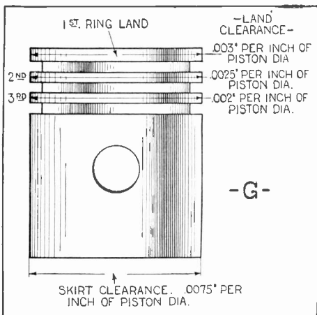
Here is shown a good rule for piston clearance. The piston should be placed in the cylinder and tried, for if it is too tight scoring will result.
