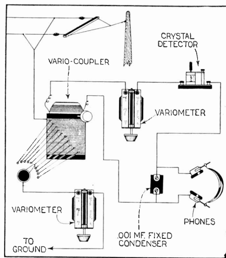
Q. 203. A selective and efficient hook-up using a crystal detector is shown above.
