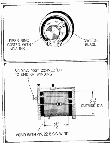
Q. 197. The top illustration shows the construction details of a variable grid leak. Q. 198. The lower diagram gives all the necessary data for a two-slide tuner, for use on the lower wave-lengths.
