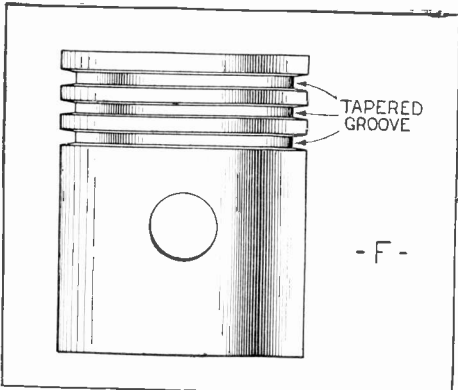
Before installing new rings in a piston examine it for groove taper. If the groove resembles the one above it should be re-turned.
