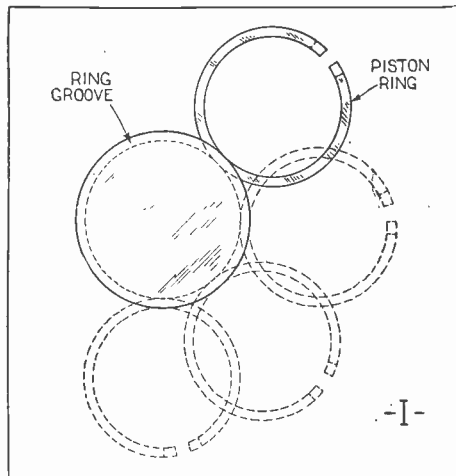
In fitting new rings into pistons roll them around the groove to see that they fit on all sides. If the ring is tight reduce it with emery paper.
