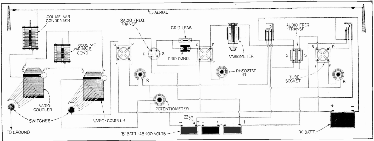
Q. 196. The selective tuner which was illustrated in the February, 1923, issue of this magazine may be used in connection with one stage of radio frequency amplification, a vacuum tube detector, and one stage of audio frequency amplification, using the circuit illustrated above. This method of connecting the instruments will give extremely sharp tuning under all conditions and regeneration is accomplished by means of the variometer.
