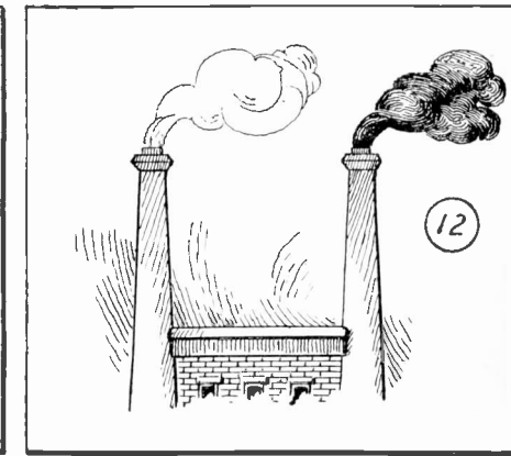
12 Black smoke from a chimney indicates incomplete combustion. No smoke, on the other hand, may indicate far too much air and a greater loss.
