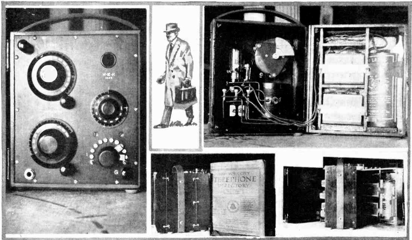
This set, called the "Single Six" receiver by the author, because the "A" battery is a single No. 6 dry cell, is illustrated in its completed form above at the left. In the lower center, the set is shown in comparison with a standard telephone directory, illustrating its compactness.
