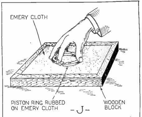
Here is shown a method of reducing a ring to fit a piston. On all rings it will be found that one side has been accurately ground. This side should be to the bottom of the groove. This will reduce leakage on the compression stroke. If the ring has to be reduced, do the reducing on the roughly finished side. Mark rings so they fit their own grooves.
