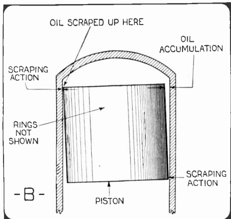
When a piston cocks in a cylinder it is caused by a warped or strained connecting rod. Such a piston pumps much oil as well as scores the cylinder wall.
