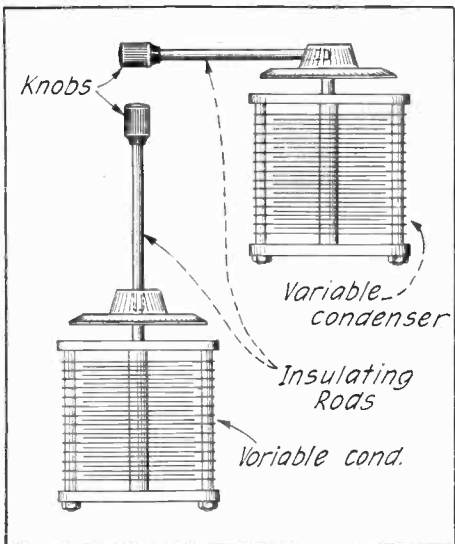
It is often desirable to tune condensers from a distance so the capacity of the body will not affect them. This may be done by drilling and tapping holes in the knobs of the condensers and attaching threaded rods as illustrated above. The condenser can then be tuned by means of the small knob. —L. J.
