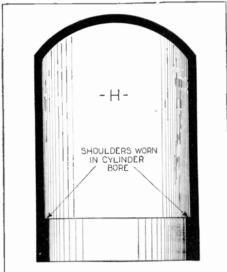
If a shoulder has been worn in the bottom of the cylinder as shown above, there is nothing to do but regrind the cylinder. This trouble also invariably causes a slight knock in the engine.
