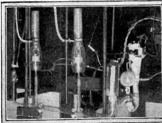
In manufacturing radio vacuum tubes, using mercury vacuum pumps the Western Electric Co. uses a liquid air trap to freeze and keep mercury vapors from returning to the tubes. (Above.) At the right is shown the liquid air "still" in operation.
