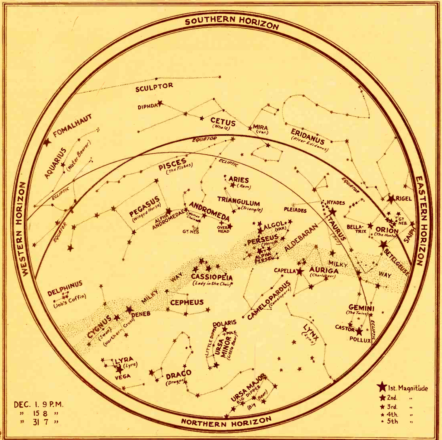
Above is the star map for the month of December. If the chart is held over the head with the "Northern Horizon," north, at nine P. M. December first or eight P. M. December fifteenth the location of the stars in the heavens will coincide with their position on the map.
