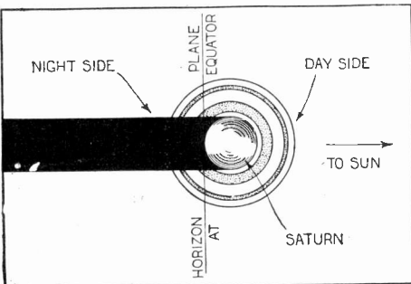
At the Equinoxes the planets shadow cuts a dark rectangle out of the rings leaving only a segment of them at each side of the horizon.
