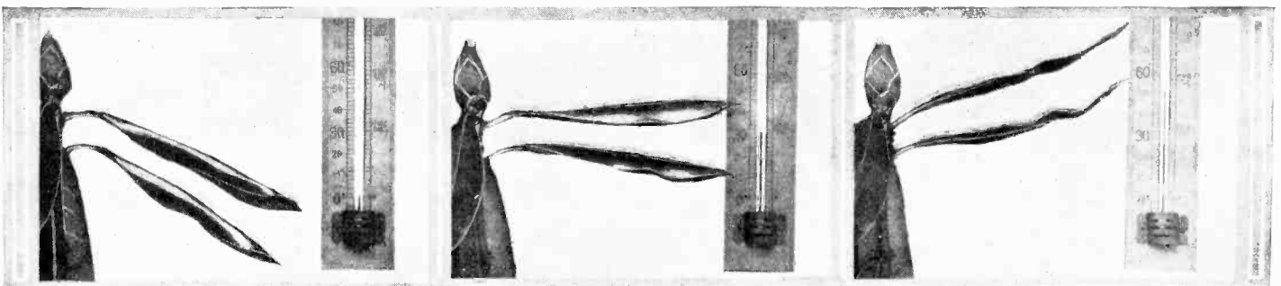
The Rhododendron gives clear indications of temperature. Its leaves form a natural thermometer. When the temperature is at about 50 deg. F. the leaves are held up. If the cold increases to freezing point the foliage becomes horizontal while at zero the leaves droop and roll inward.—S. Leonard Bastin.
