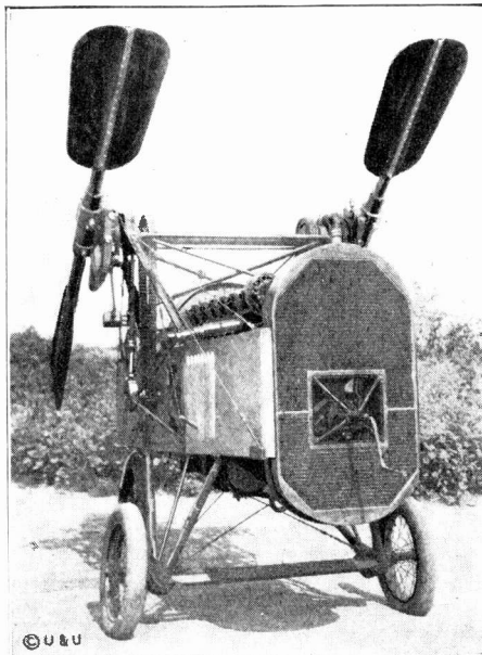
The inventor of this machine, E. R. Johnson, claims it will ascend, descend, move forward, backward, or remain stationary in the air. It will compete in the British helicopter contest.
