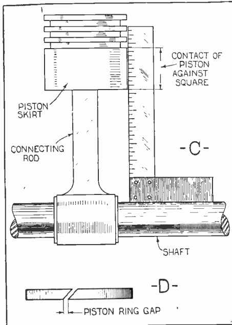
Above is shown a method of testing a piston for alignment. The connecting rod is bolted to a mandrel and the piston tested with a square as shown above. Both skirt and top of the piston should touch the square. To test the wear of a piston ring, place it in the cylinder and measure the gap. A gap should never be more than .002 to .003 inch for each inch of piston diameter.
