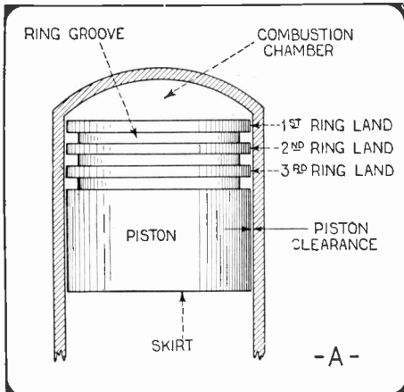
Here is shown an illustration of piston play. Also the sketch shows the correct names of the parts of a piston. All measurements should be made with micrometers.
