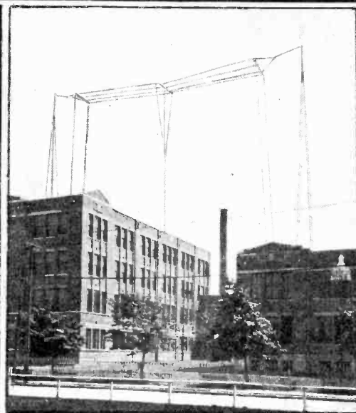
Monitoring Apparatus for Checking Up on the Programs. Announcements May Also Be Made from This Desk. Above, at Right: The Antenna System of WSAI Supported on Two Steel Towers 167 Feet Above the Street Level. The Active Antenna Length is 65 Feet with a Lead-in of 137 Feet.
