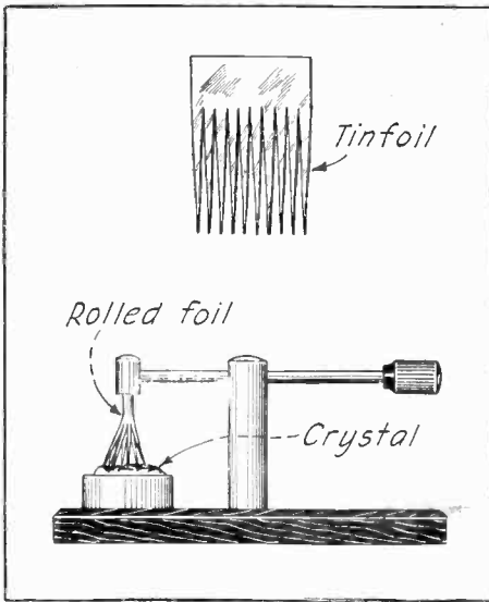
A strip of tin-foil cut as shown and rolled into a cylinder at the top makes an excellent cat whisker. —A. W.
