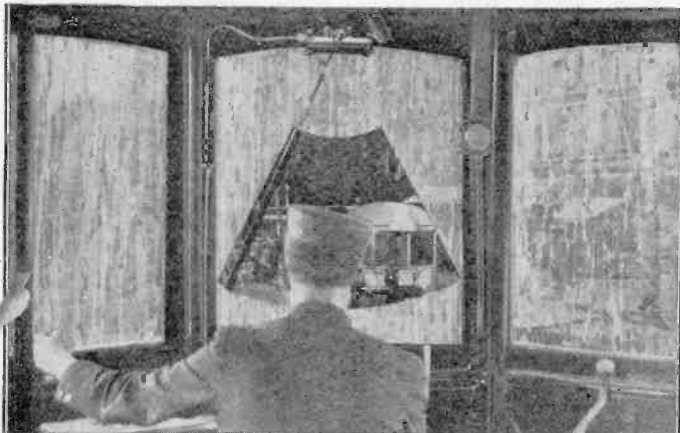
A Cleveland firm has just brought out a wind-shield wiper for use on trolley cars. It is made on the same principle to a similar device used on automobiles. The long arm with the rubber wiper attached is operated by a small piston and compressed air.
