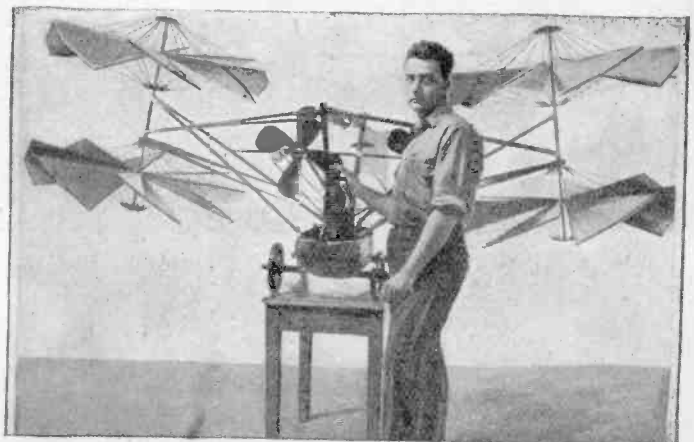
The general idea that the helicopter is a new development in aircraft is false as will be seen by the picture above which shows a model of one designed by Sir George Cayley in 1843. Photo shows Paul Garber of the U. S. National Museum, Washington, D. C., who built the model.
