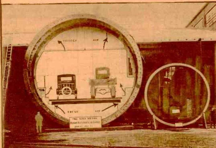
At the left is shown a cross-section of one of the finished segments of the steel tunnel. The system of ventilation can be plainly seen. To the right is shown a section of what was formerly the largest under-river railroad tunnel in the world. The pleasure car and truck indicates how fast and slow moving vehicles will be divided to prevent congestion.
