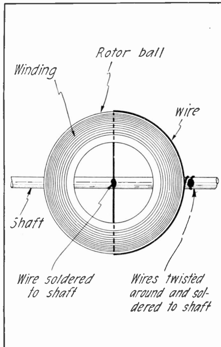
Drill two holes in opposite sides of the rotor ball, as shown. Pass a stiff wire through them around one-half the ball and solder to center and end of shaft. The rotor will be held rigid.
