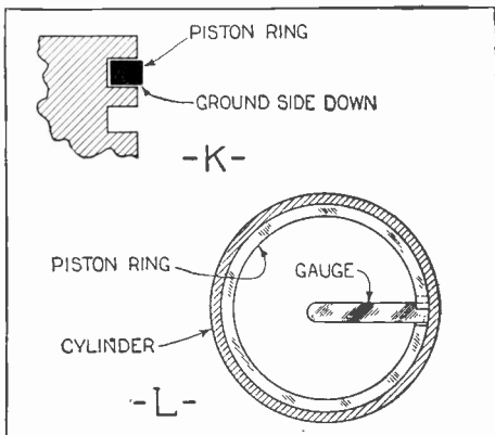
After placing a ring on a piston, test the gap for size. This is done with a feeler gauge. If the gap is too close the ends should be filed.
