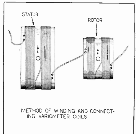
Q. 204. The rotor and stator of a variometer are always wound in the same direction and connected as shown above.
