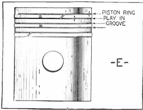
A ring loose in its groove is the cause of oil pumping and lack of compression. Even new engines sometimes show such trouble.
