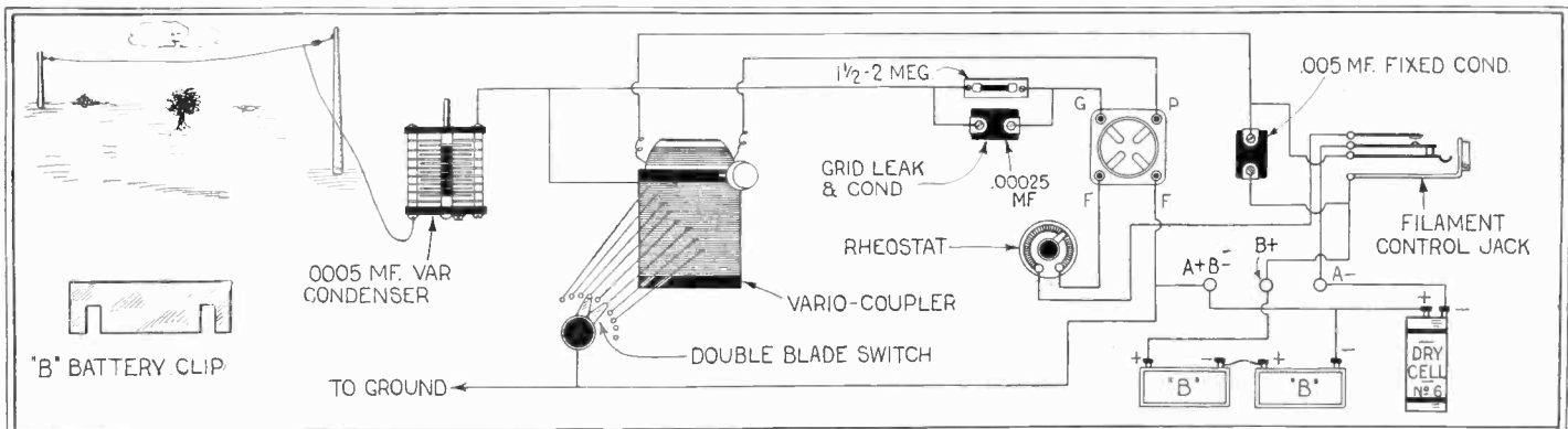
The circuit diagram of the "Single Six" receiving set is shown in simplified form above. Note the filament control jack, by the use of which the filaments will be extinguished upon removing the phone plug from the jack. This set will give fair selectivity and excellent volume under all conditions.
