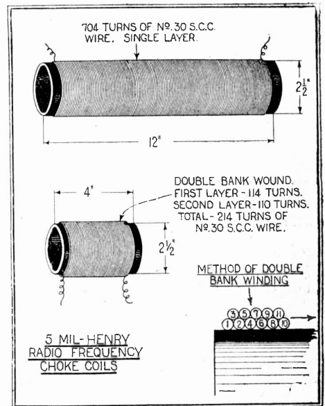
Q. 200. In various radio receiving and transmitting circuits, it is necessary to use radio frequency choke coils. Two methods of winding a 5 mil-henry choke coil are shown above, one using only a single layer of winding and the other two layers, bank wound.
