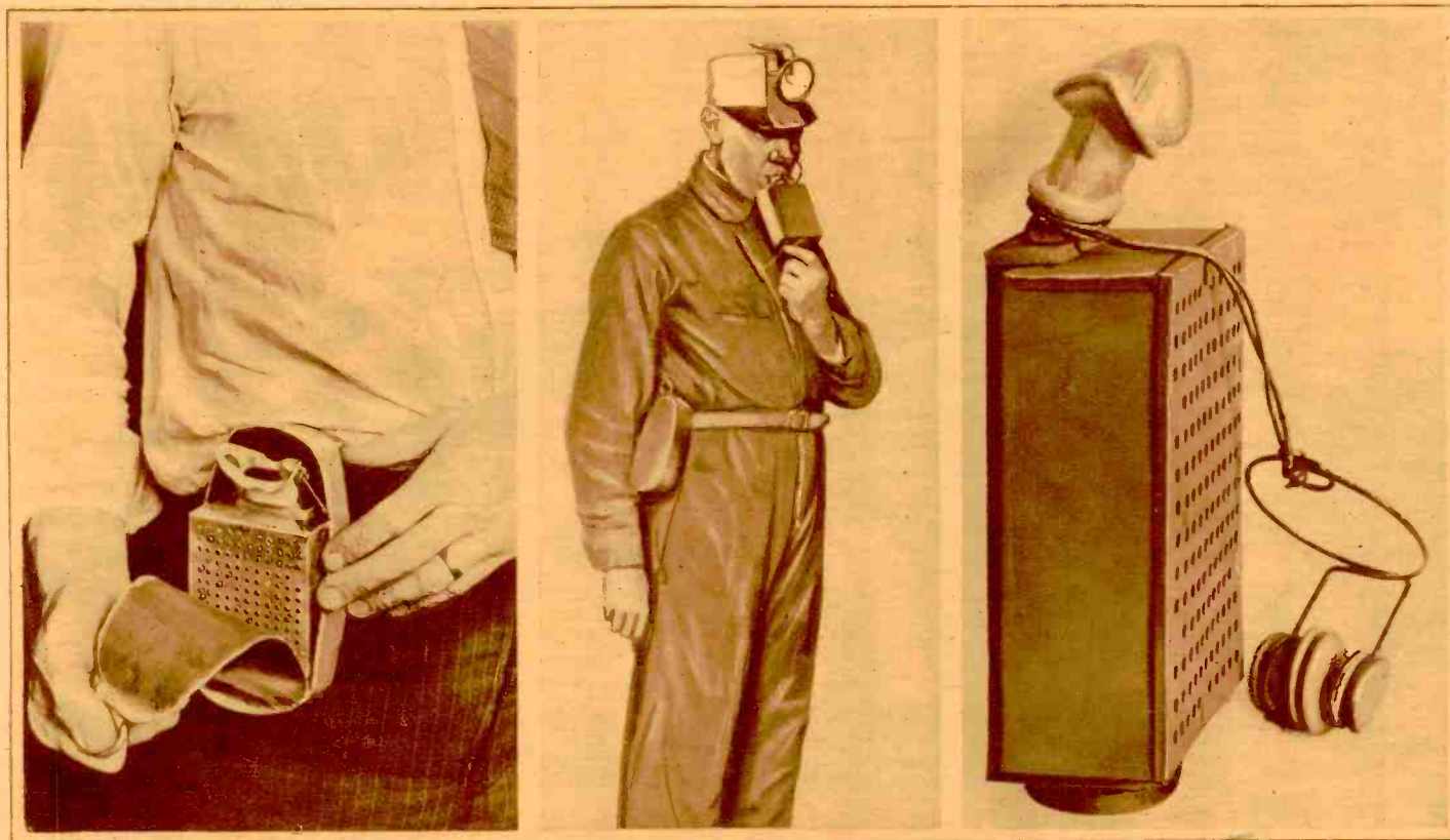
his teeth. The perforated box contains hopcalite which counteracts carbon monoxide, the most deadly of mine gases. The chemicals will give relief for seventy minutes, allowing miner time to reach safety.—John M. Schalek.
