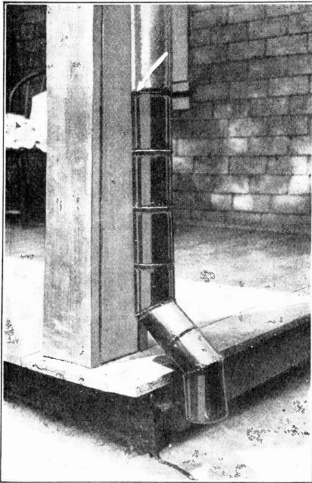
Remove the top and bottom of condensed milk cans and use to repair old drain pipes. They fit the 3-in. pipe. —J. H. Shalek.
