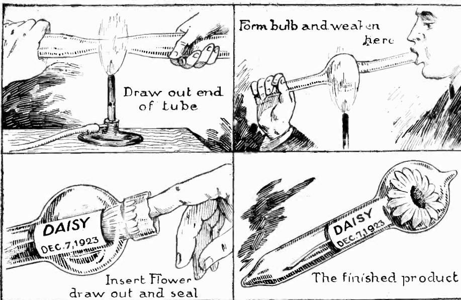
By placing a bloom in a sealed glass tube blown as shown above they may be preserved in their original state for two years. The paper with the name and date helps support the stem of the plant. If the tube is filled with an inert gas like nitrogen the flower will remain fresh much longer. After sealing the tube it should not be allowed to remain in the sun light on account of the deteriorating effects of the ultra-violet light. —H. O. Bernstrom.
