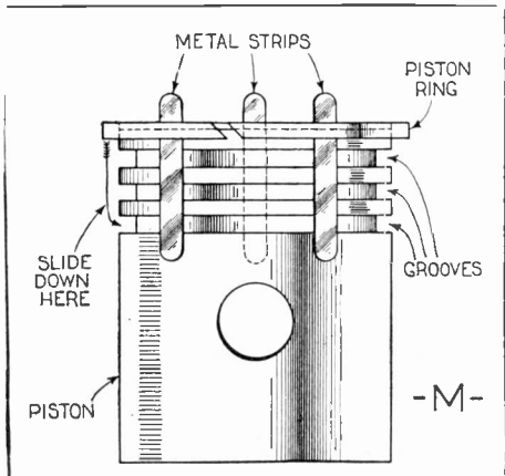
Here is given the method for placing the rings on the piston. Put on bottom ring first.
