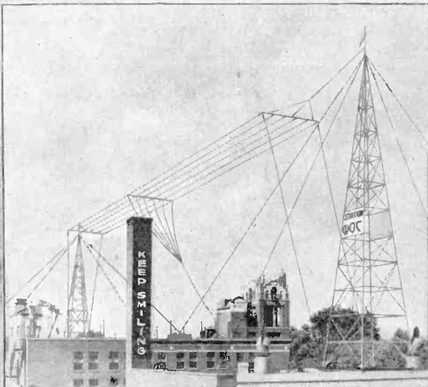
Above is shown the antenna system of WOC. The towers are placed atop one of the buildings of the school. Their total height is 130 feet above the street level. They are more than 300 feet above the level of the Mississippi River. On account of the severe winds that hit the city in the winter months special care had to be taken in the construction of the masts to make them proof against the gales. At night the towers are outlined by flood lights which make them visible for miles around the tri-cities. This station has a good distance record to its credit and has given great satisfaction in its operation. It was installed as a means of advertising the chiropractic system of healing.
