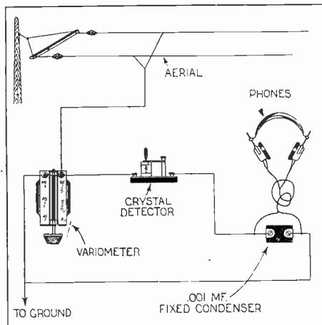
Q. 199. A crystal receiving set using only one tuning control may be connected as illustrated above. Selectivity is not very high, but the volume obtained is very good.
