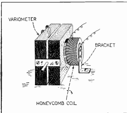
Q. 202. By placing a honeycomb coil in inductive relation to a variometer as shown above, regeneration by the feed-back principle will be obtained.
