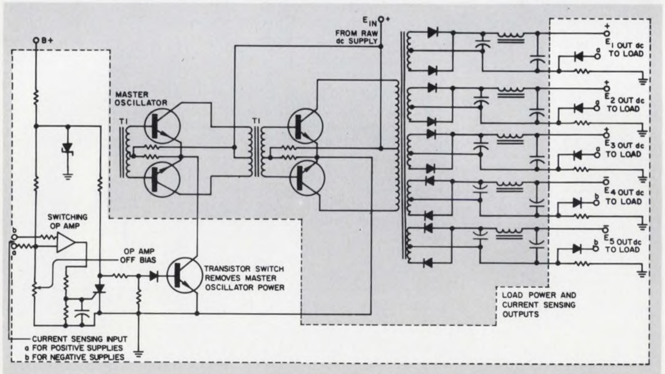
13. Multiple output line toggle reset using OR'd resistor sensing.
