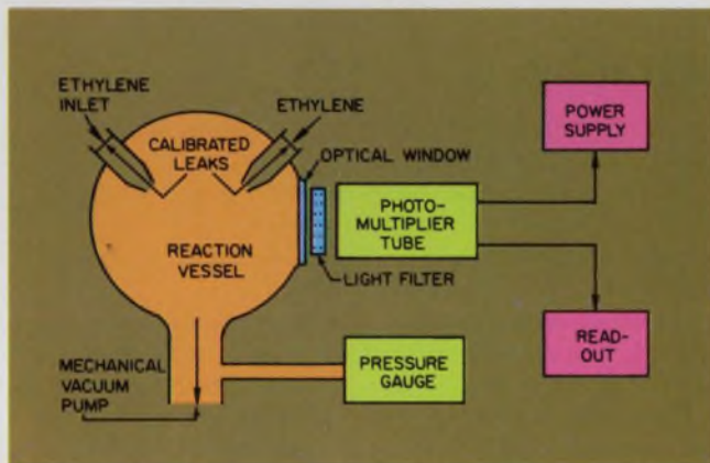
Fig. 2. Reaction of ozone with ethylene yields a chemiluminescent glow, the level of which is proportional to the concentration of ozone in the sample.
