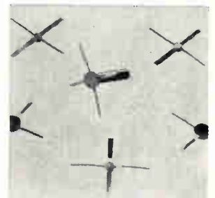
Low noise, high gain, npn epitaxial silicon microwave transistors come in three types. The input stage, model AT-101, typically provides 4 db noise figure and 10.5 db gain at 2 Ghz. The intermediate-stage AT-201 can deliver 10 dbm of linear output power at 2 Ghz. The output-stage AT-301S operates linearly at 17 dbm. Avantek, 2981 Copper Rd., Santa Clara, Calif. 95051 [439]
