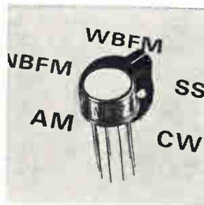
Multiple-mode, monolithic i-f strip LM373 is for a-m, f-m and ssb i-f applications as well as broad-band video amplification. It can serve nearly all radio users by incorporating those subsystem functions which may be changed with a few external connections from duties required of one mode to those of another. National Semiconductor Corp., San Ysidro Way, Santa Clara, Calif. [437]
