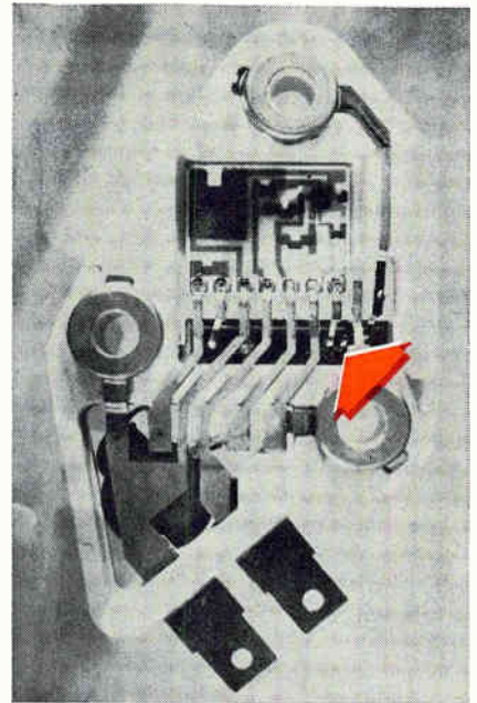
Under the hood. High-gain Darlington power amp and rectifier, on a special heat-sink bar in Motorola's auto voltage regulator, are indicated by arrow.
