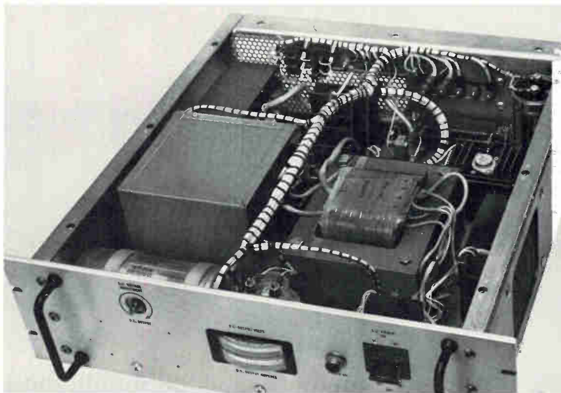
CR27.5 High-current, adjustable, 1% regulation, 28 V.D.C. output, 50-60 Hz unit. Withstands substantial overloads.
