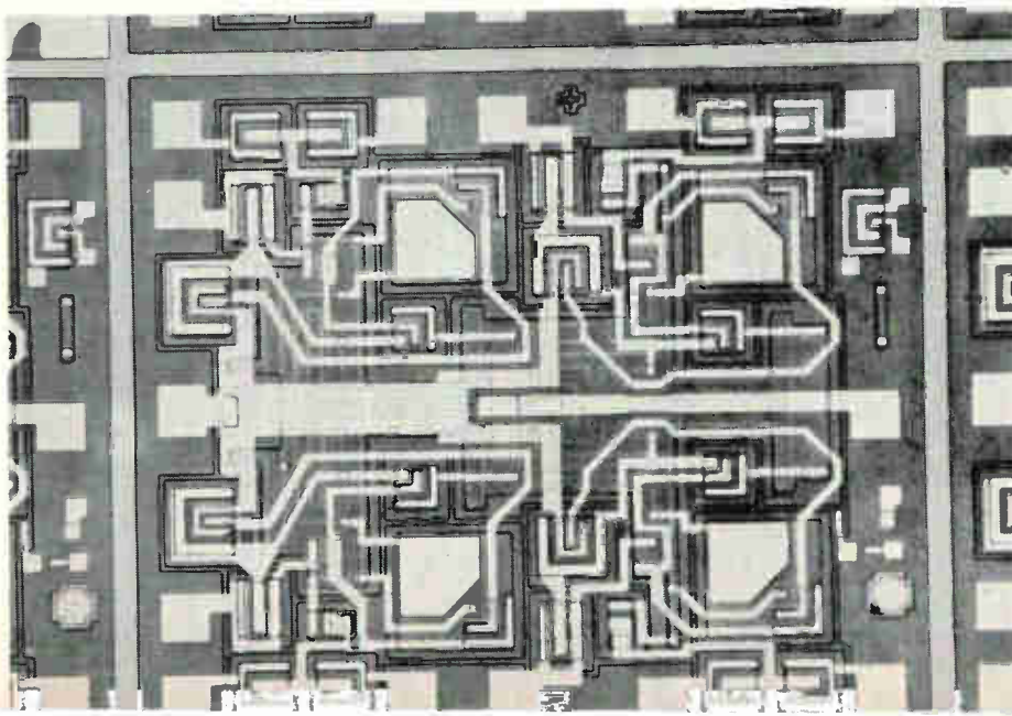
Big junctions. To maximize the Miller capacitance, the collector-base junctions have been made extremely large. This circuit is a quadruple dual-input gate, type 1.
