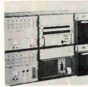
Compact data acquisition system series SY-128 accepts 400 channels of strain gage, temperature bulb, dc/dt transducer inputs. The system includes transducer excitation and calibration networks. All signal inputs are scanned and measured with the resulting data recorded simultaneously on a printer for quick assessment. B&F Instruments Inc., Cornwells Heights, Pa. 19020 [426]
