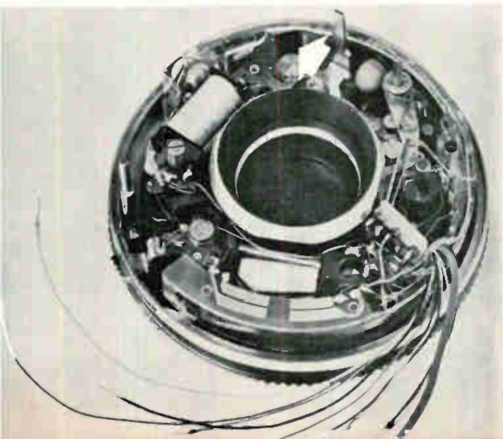
Concealed. IC for exposure-time control is mounted on a ring around the camera's lens. Addition of an identical IC would permit delayed shutter opening.
