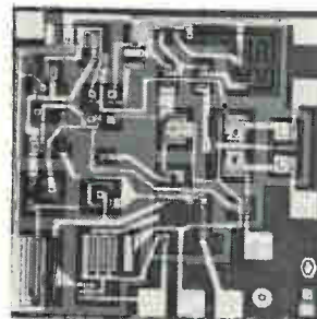
IC operational amplifier UC4101A has a guaranteed low offset current of 20 na maximum over a temperature range of -55^{\circ} to +125^{\circ} C. Design permits operation with \pm 5 to \pm 20 v power supplies. Typical applications include inverting and noninverting linear feedback amplifiers, and voltage follower stages. Union Carbide Semiconductor, 8888 Balboa Ave., San Diego, Calif. 92123. [442]
