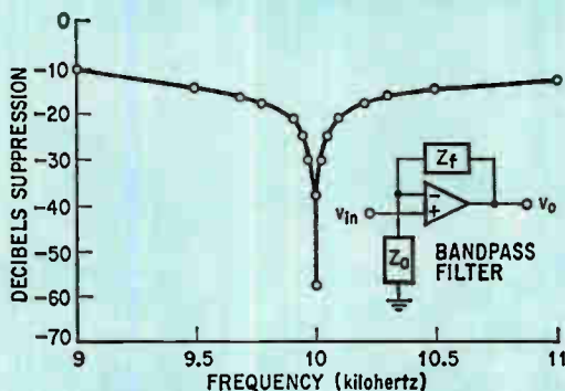
Sharp response. The notch filter can be placed in the feedback loop of a degenerative amplifier to produce a narrow bandpass filter.
