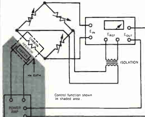
LOCK-IN AMPLIFIER USED AS BRIDGE OSCILLATOR/NUL DETECTOR
