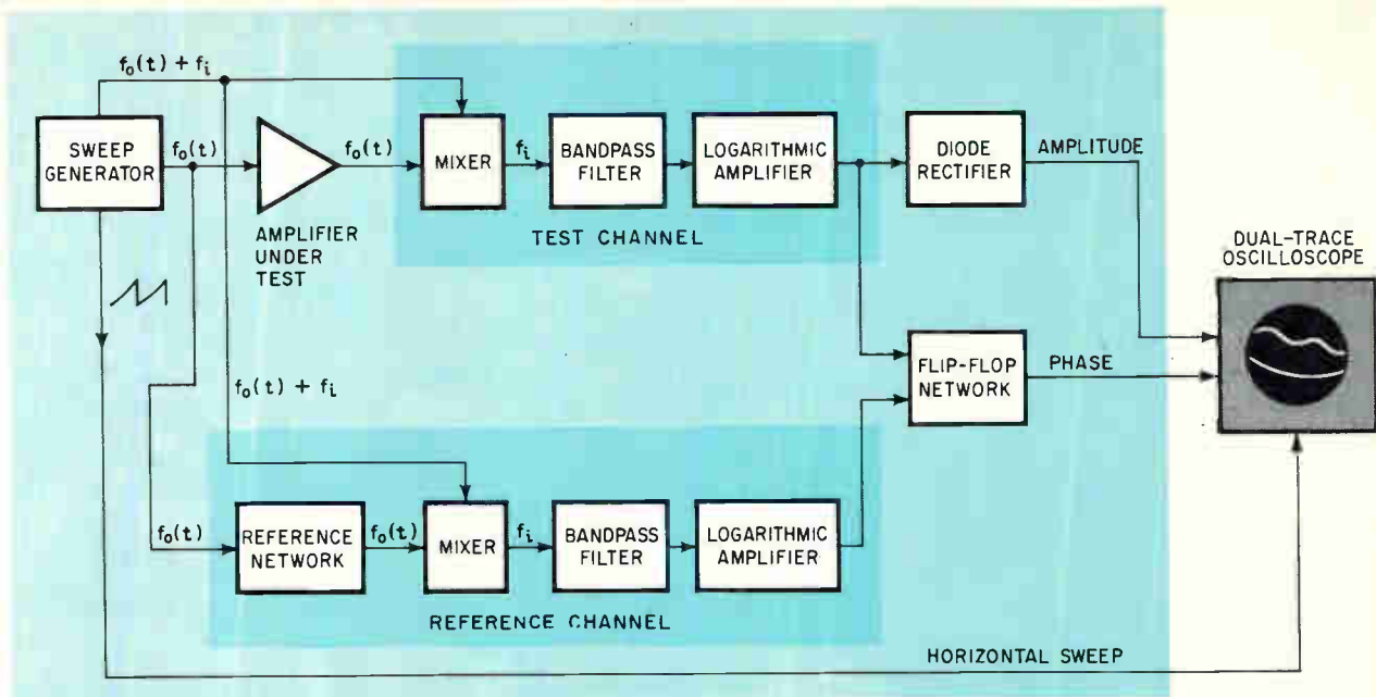
Gain and phase. The amplifier's input is the swept signal, f_o(t) . Its gain and phase are proportional to the rectifier's output and the flip-flop network's output, respectively. The scope plots both against f_o(t) .
