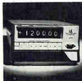
Five-digit voltmeter/multimeter model 370 features high accuracy (0.0025%) in a package 3 \frac{1}{2} in. high, half rack size. The unit can also measure a-c volts (to 100 khz), ohms (to a resolution of 1 milliohm) and ratio (0.99999:1), by simply adding plug-in modules. Price is $2,400; delivery, 60 days. Data Technology Corp., 1050 East Meadow Circle, Palo Alto, Calif. [367]
