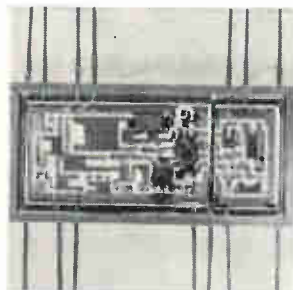
Film hybrid clock driver MS301 is a 20-Mhz device that can drive up to 15 SUHL II or equivalent-type flip-flops. It has multiple ground leads, internally connected bypass capacitors, and pin arrangement permitting convenient mounting near the flip flops to be driven. Size is 0.815 x 1.725 x 0.150 in. Sylvania Electric Products Inc., 100 First Ave., Waltham, Mass. [441]
