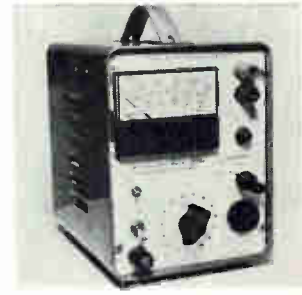
Multiple range, solid state, voltage breakdown tester, model 791, is suitable for testing both low and high voltage transistors, thyristors, diodes and rectifiers for zener breakdown levels. It has four voltage ranges: 0-50, 0-100, 0-1,000 and 0-5,000 volts. The high voltage output is continuously adjustable on every range. SVI Electronics, 48 Broadway, Albany, N.Y. [364]
