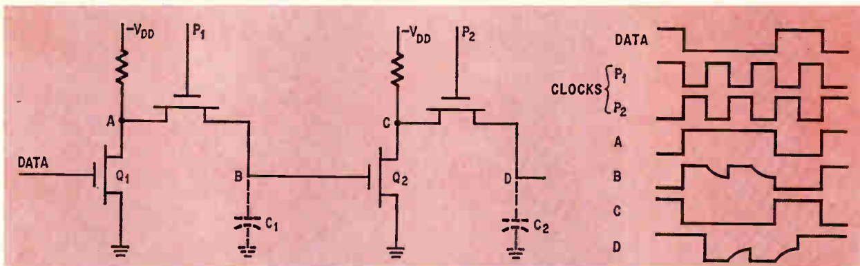
Dynamic. Gate capacitance of transistor Q_2 , shown here as C_1 , picks up the inverted data at A when P_1 is negative, retains it long enough for P_2 to transfer it to the gate capacitance of the next stage. Charging and discharging rates determine minimum and maximum frequencies of the circuit.
