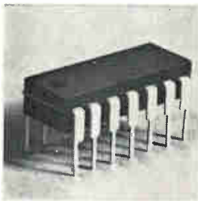
Monolithic IC TAD100 contains all the active components for a complete a-m radio receiver: oscillator, mixer, i-f amplifier, detector, agc, and audio preamp and driver stages. A-m sensitivity is 50 \mu v/meter for 100 mw audio output. Agc range is 65 db for an audio output change of 10 db. Total harmonic distortion is 2%. Amperex Electronic Corp., Slatersville, R.I. 02876 [436]
