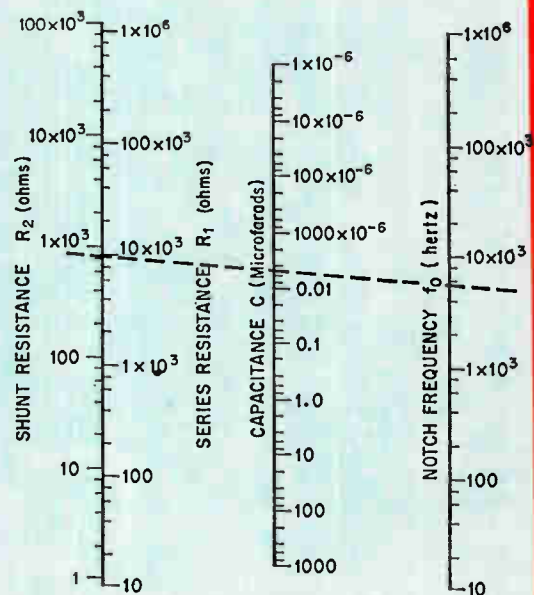
Quick and easy. A nomograph quickly and easily determines the values for all circuit components needed to design an RC notch filter.
