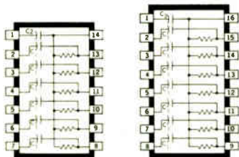
BYPASSED PULL-UP AND R-C COUPLING NETWORKS
