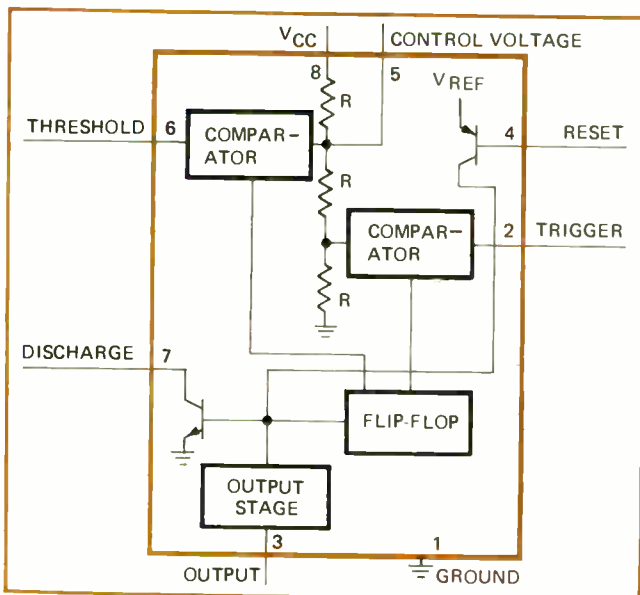
555-type timer. Internal resistive divider sets switching voltages for both of the circuit's comparators, which then toggle the flip-flop.
