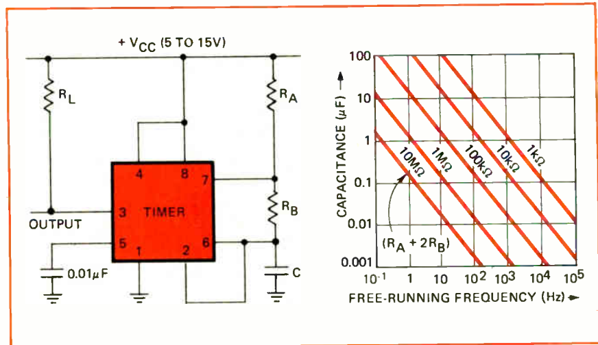
Astable hookup for the 555. With this simple connection, the timer operates in its free-run mode. The capacitor charges through resistor R_A and discharges through resistor R_B .
