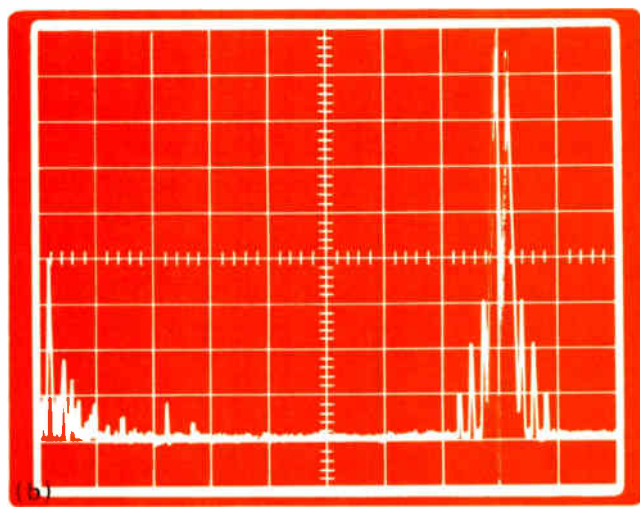
7. Sweep speeder. Trace made with a conventional sweep at optimum speed takes 100 seconds (a). Adaptive sweep, however, reduces dynamic range, eliminates noisy signal floor, and cuts sweep time to 10 seconds (b). The adaptive-sweep cutoff threshold is adjustable.
