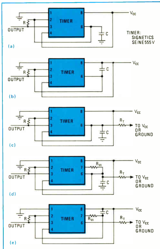
Choice of generators. Timer IC (a) generates symmetrical square-wave output. Slight output ringing can be eliminated with circuit (b). Output symmetry can be adjusted with external trimmer (c), or output pulse width made variable, as in circuits (d) and (e).
