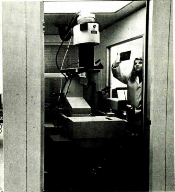
For the 1980's, GCA's DSW Wafer Stepper/Wafertrac, shown here interfaced, forms one of the most highly automated production systems for advanced device manufacture available today.
