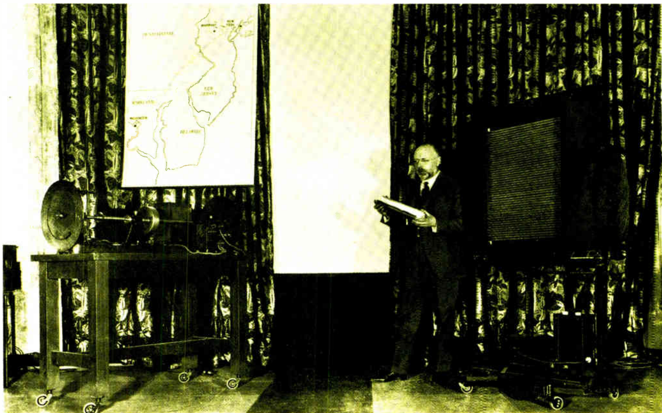
Demo. Bell Telephone Laboratories' Herbert Ives holds giant photoelectric cell that picked up signals at Bell's first public demonstration of TV on April 7, 1927. Screen (right) uses a meandering neon tube with electrodes placed so as to form a 2,500-element picture grid.
