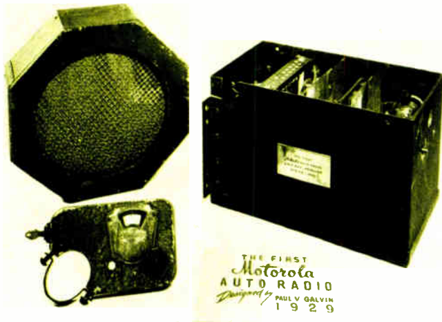
First car radio. Motorola (then Galvin Manufacturing) introduced it at the 1930 convention of the Radio Manufacturers' Association.
