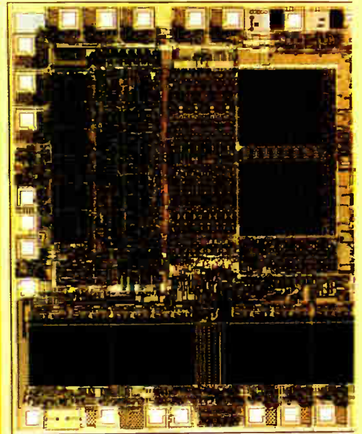
EF 6305 - 8-bit microcomputer IC for consumer applications.
