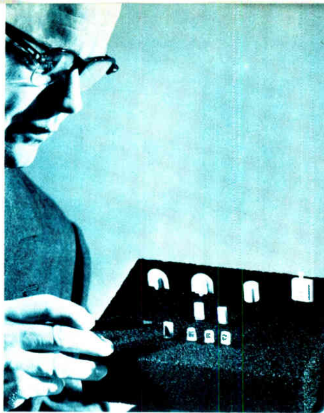
Shaping up. By 1952, germanium transistors had begun to take on standard shapes and pin configurations. The three rightmost transistors in the front row are point-contact devices; the rest—including the power transistors in the rear row—are junction types.
