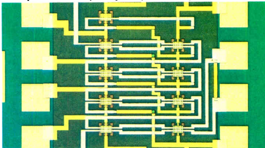
Experimental circuit of a 4bit parallel full adder using 9 DC-SQUID gates
