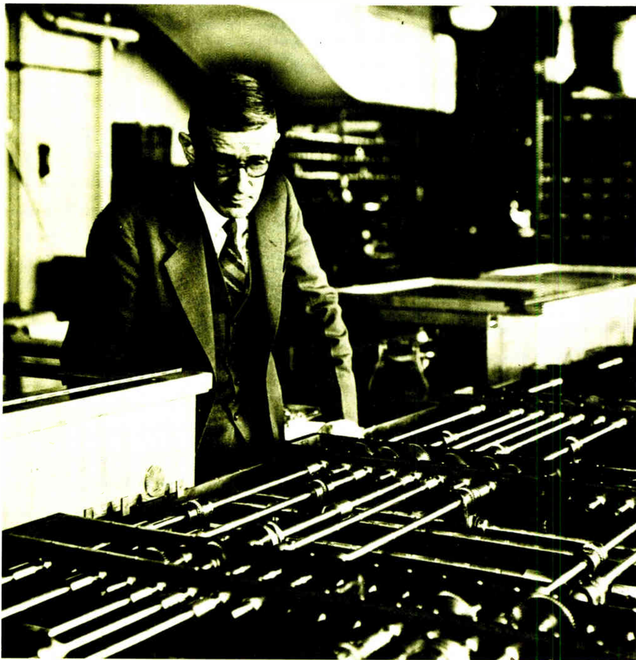
Analyzer. Vannevar Bush completed this differential analyzer in 1931 at the Massachusetts Institute of Technology. The analyzer was one of a series of Bush machines that were the precursors of modern analog computers. Their development stemmed from Bush's work on electric power transmission systems. He felt the need for machines that could perform analytical tasks too formidable for mathematicians alone.
