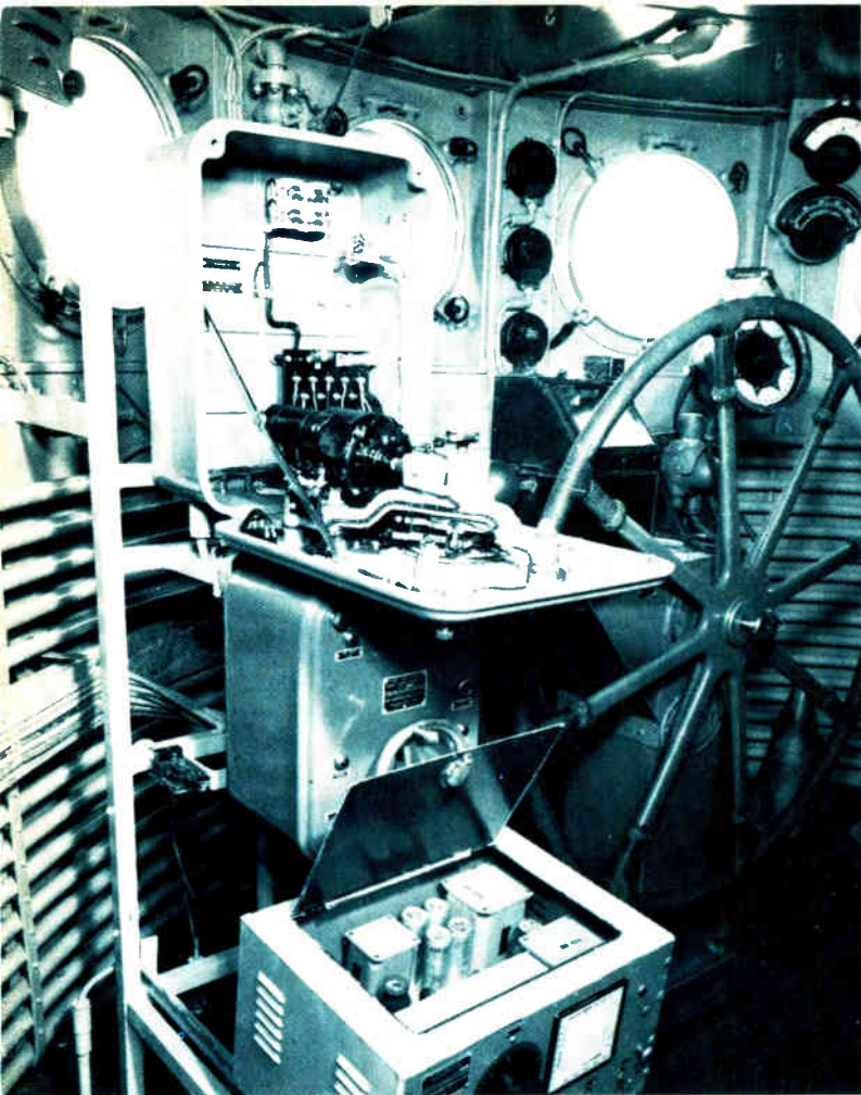
Antisub. In 1944, when this installation was photographed, sonar technology had enabled the Allies to greatly reduce the huge losses of shipping to German submarines. Such systems were capable of determining a submarine's depth and could track its movement.
