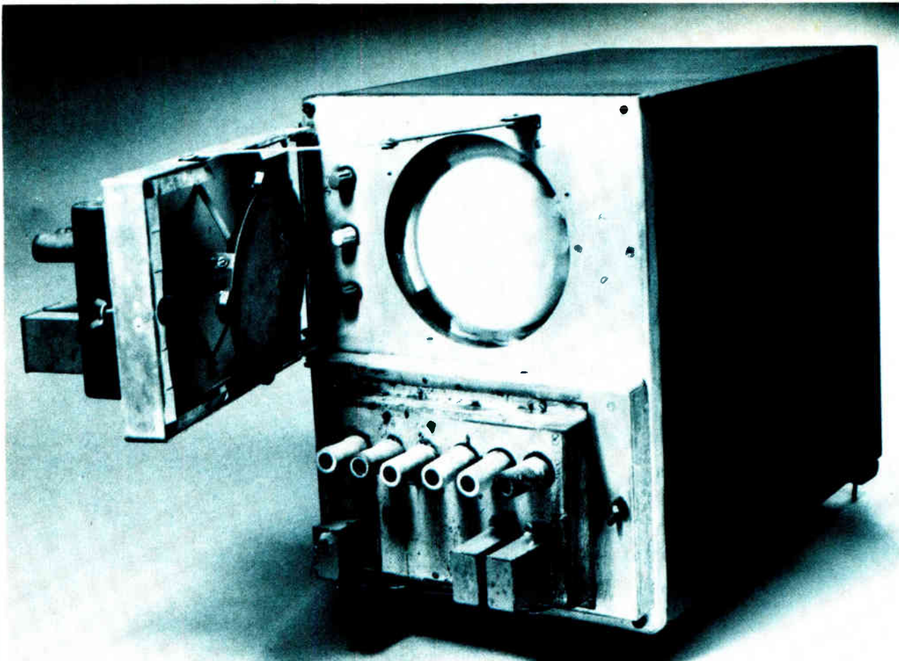
Breakthrough. The Williams tube, named for its inventor, F. C. Williams, was the first all-electronic memory, essentially a storage tube that utilized capacitive coupling at the tube face to sense data in the form of charges stored on the phosphor coating.
