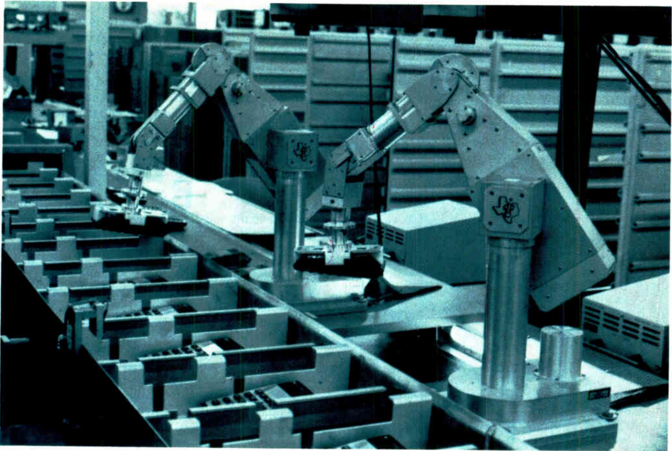
Pick and place. Robot arms made some progress during the decade in taking over boring and dangerous jobs. These at a Midland, Texas, plant of Texas Instruments transfer calculators from one conveyor belt to another. Overhead TV cameras help them search for "targets."
