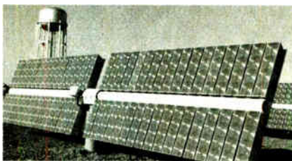
2 1/4" diameter concentrator cells from Applied Solar Energy are the heart of this point focus fresnel system
