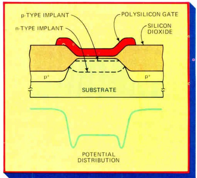
No capacitor. Present random-access memories use only one transistor per cell, but a capacitor is also present. Various approaches have been tried to drop that capacitor; this taper-isolated cell is one of them. The potential distribution traps charge.
