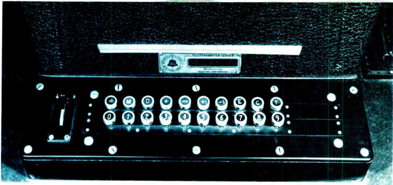
Early computer. This keyboard belonged to the first Bell Laboratories relay computer, which was put into operation in 1940 at the laboratories' old West Street facility in New York City. It was for this computer that binary-coded decimal notation was developed.
