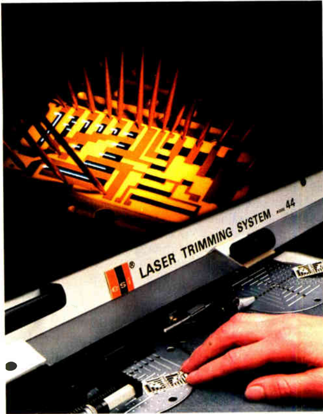
Trimmer. Computer-controlled laser trimmers boosted microcircuit yield by precisely removing excess thin- or thick-film resistive materials. A Q-switched YAG laser unit from trimmer pioneer Electro Scientific Industries is shown trimming a thick-film hybrid.
