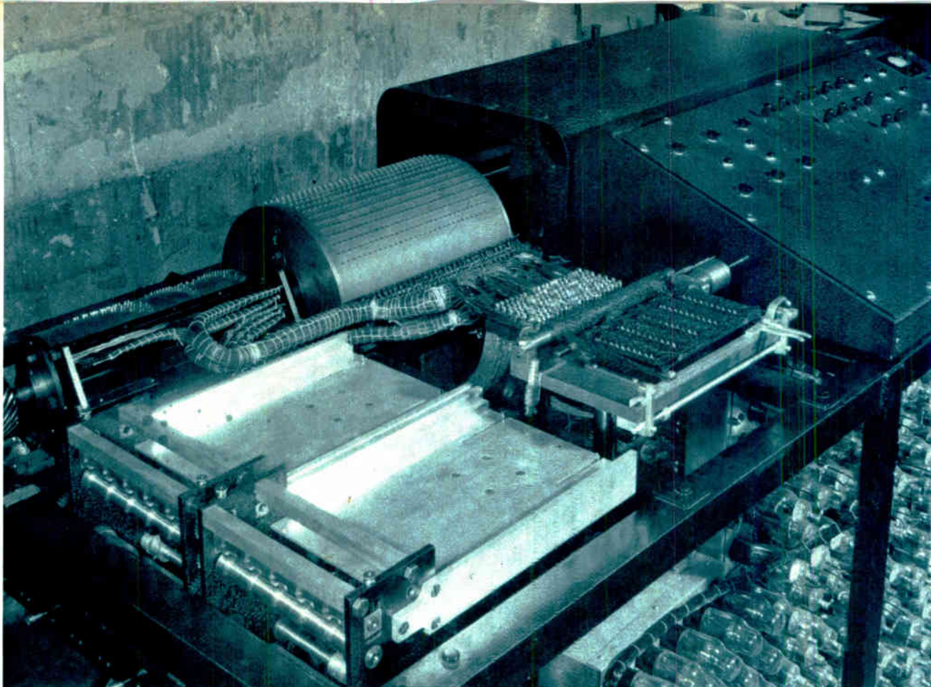
Precursor. This prototype digital computer, one of the earliest to use vacuum tubes as logic elements, was designed and built by John V. Atanasoff at Iowa State College for solving linear algebraic equations. He became involved in a patent dispute with Eckert and Mauchly.
