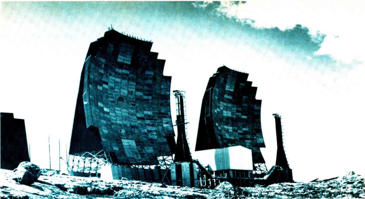
Missile seeker. This pair of antennas was part of the Ballistic Missile Early Warning System (BMEWS) built by Western Electric in Labrador. BMEWS could detect missiles 3,000 miles away at a height of 600 miles, giving about 20 minutes of warning.
