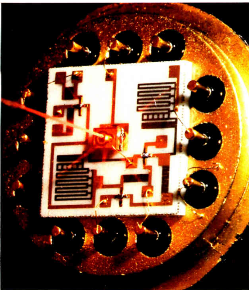
Talking lightly. Prototype for Bell System's FT 3 standard fiber-optical system used an avalanche photodetector diode as the receiving element in a thin-film preamplifier circuit in a TO-8 can. Invisible infrared laser will replace helium-neon laser light shown.
