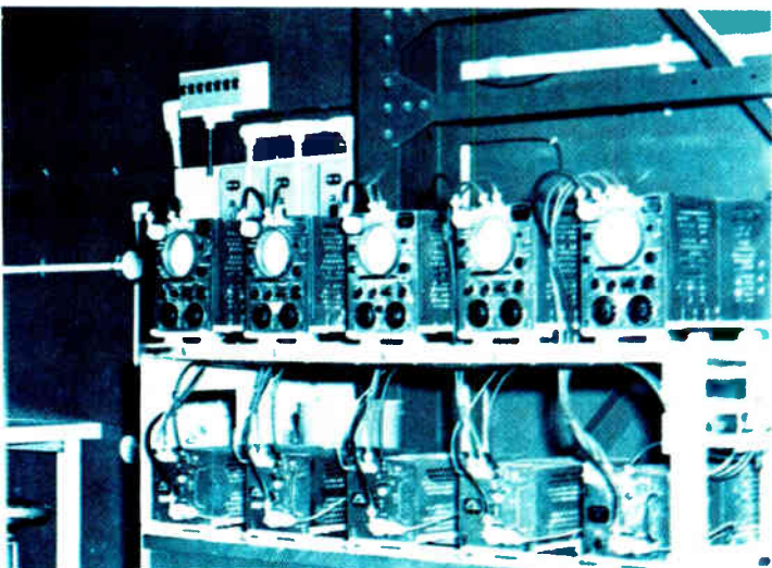
Navigation. Another contribution of the MIT Radiation Laboratory to the war effort was loran, a system by which vessels could determine their true position very accurately. This early installation (circa 1945) was at the Naval Air Station at Whidbey Island, Washington.
