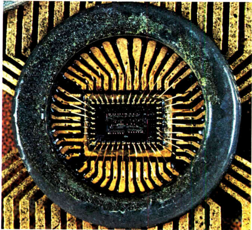
Round flatpack. The MOS integrated circuit's capacity for denser ICs than bipolar devices brought about this packaging scheme in 1965. The chip, a custom circuit for the military, integrated 968 components in the 44-pin package.
