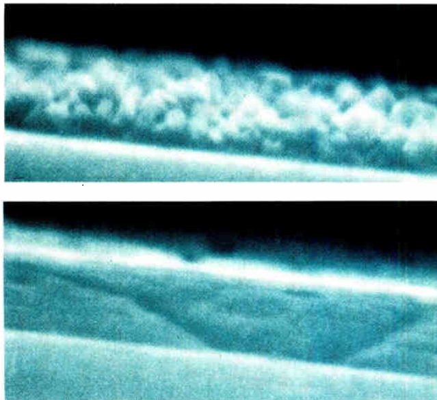
Soothe it. Is it possible to build three-dimensional ICs? Sure, and laser-annealed polysilicon may hold the key. In (a), polysilicon on silicon dioxide is shown before annealing; note the rough, pebbly texture. In (b), that polysilicon is annealed; it is much smoother.
