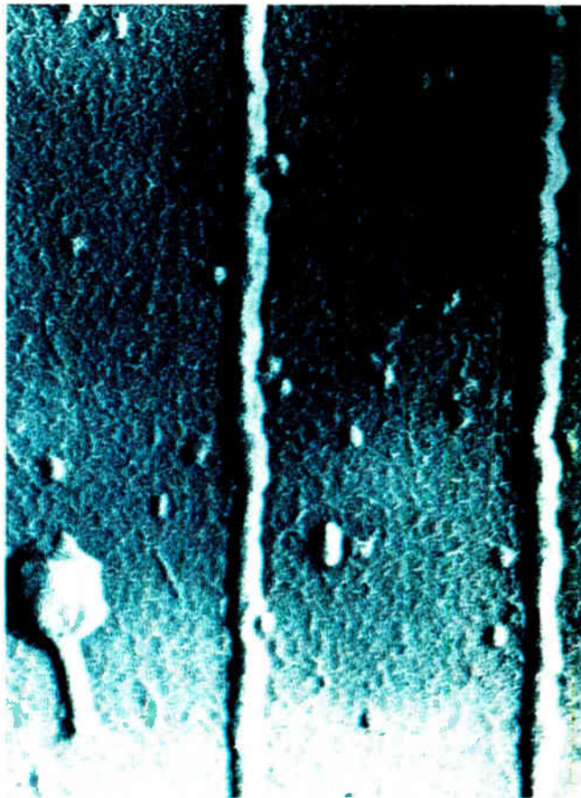
Slender. Researchers at MIT's Lincoln Laboratory used a polyimide mask shadowed with tungsten and X-ray lithography to resolve these 200-Å lines of PMMA photoresist on a silicon dioxide substrate. For comparison purposes, a T4 phage virus was placed on the sample.
