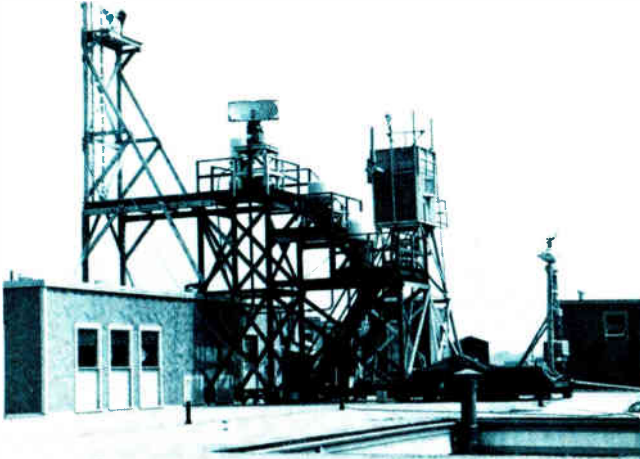
Rooftop radar. The MIT Radiation Laboratory was the scene of much of the experimental work that produced U. S. military radar. Shown here are experimental antennas atop the laboratory's Building 6 near Massachusetts Avenue in Cambridge.
