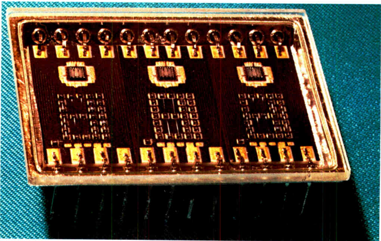
Indicator. Light-emitting diodes were being fashioned into rugged displays for industrial environments and the military. This numeric indicator from Hewlett-Packard uses gallium arsenide phosphide emitters in a 5-by-7-dot matrix. Each numeral contains its own decoder/driver.
