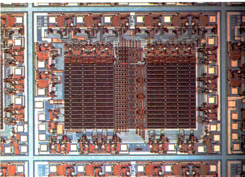
Erasable memory. The first erasable programmable read-only memory was developed by Intel in 1972. The 1702, a 2-K device, relied on charge stored on oxide-embedded floating gates, which could be discharged under exposure to ultraviolet light.
