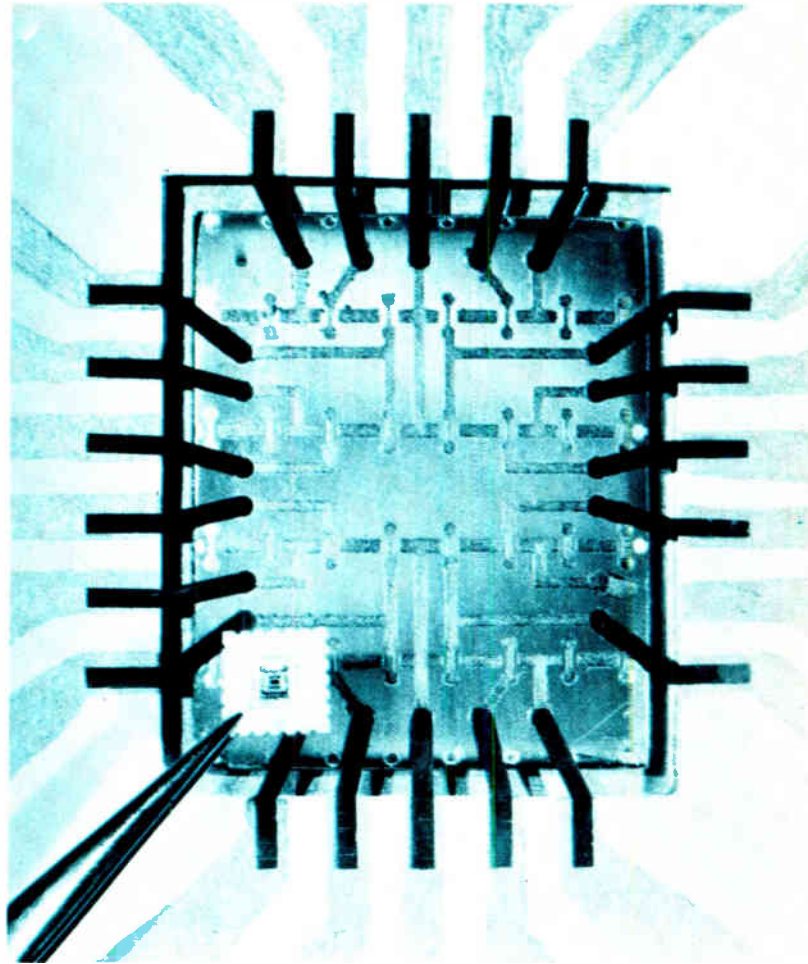
Early MOS. The close-up of the ceramic-packaged metal-oxide-semiconductor chip (held by tweezers) is actually a mockup, but it shows the details of the metal interconnecting 16 MOS transistors in this logic circuit from RCA. The year was 1963.
