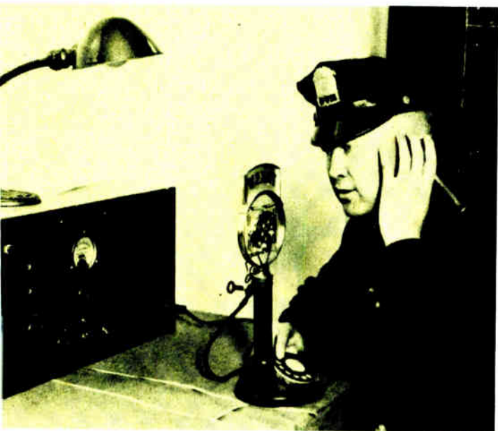
10-4. Not Broderick Crawford, but Patrolman H. H. Moon of the New Rochelle, N. Y., police uses radio to communicate with police cars direct from headquarters. The dial serves to connect the police system with telephone lines for local and long-distance hookups.
