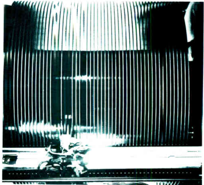
Juke-box memory. Considered revolutionary when introduced was this disk-storage unit designed for the IBM 305 and 650 Ramac machines. It comprised 50 magnetically coated spinning disks. Each disk had 100 data tracks, each storing 10,000 characters.
