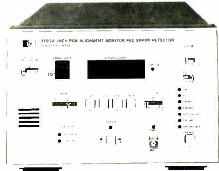
The easy-to-use 3783A 30 Ch PCM Alignment Monitor and Error Detector has a strip chart recorder output to let you make hard copies of the measurement results.
