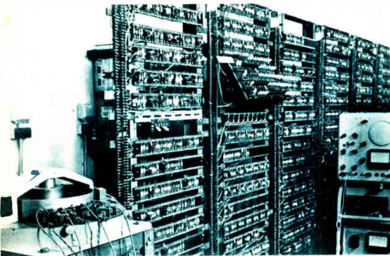
Transistors arrive. Another first for the British was this experimental computer assembled at Manchester University, with germanium point-contact transistors. Using a magnetic drum as main store, it was slow but probably the first stored-program transistor computer.
