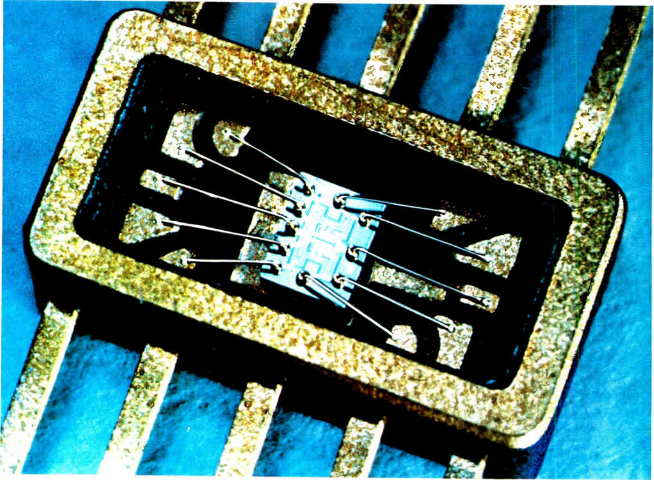
Apollo chip. One of the early bipolar integrated circuits, this chip—a three-input NOR gate using resistor-transistor logic (RTL)—was built by Philco-Ford for MIT Lincoln Labs. It emphasized reliability—a backup computer for an Apollo program launch was built entirely of these chips.
