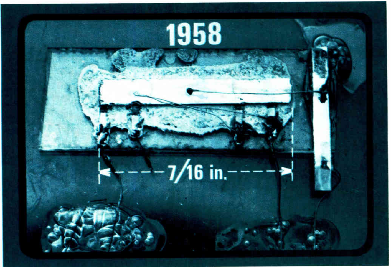
First integrated circuit. The first IC, developed at Texas Instruments Inc., proved an entire circuit could be built with silicon. The bars, actually sections from a wafer of mesa transistors, became breadboards in this oscillator using silicon as resistors, capacitors, and transistors.
