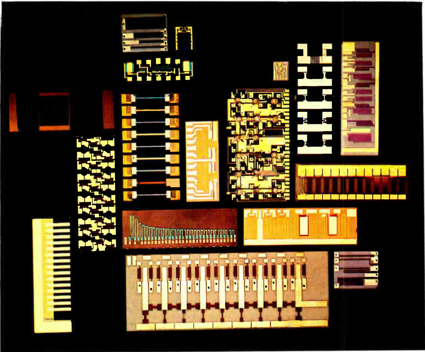
Shapes and sizes. Hybrid circuits in a striking variety of sizes, shapes, and colors were developed for the new miniature electronics. Different colors in these 1967 tantalum thin-film circuits from Bell Telephone Laboratories result from different thicknesses of tantalum oxide.
