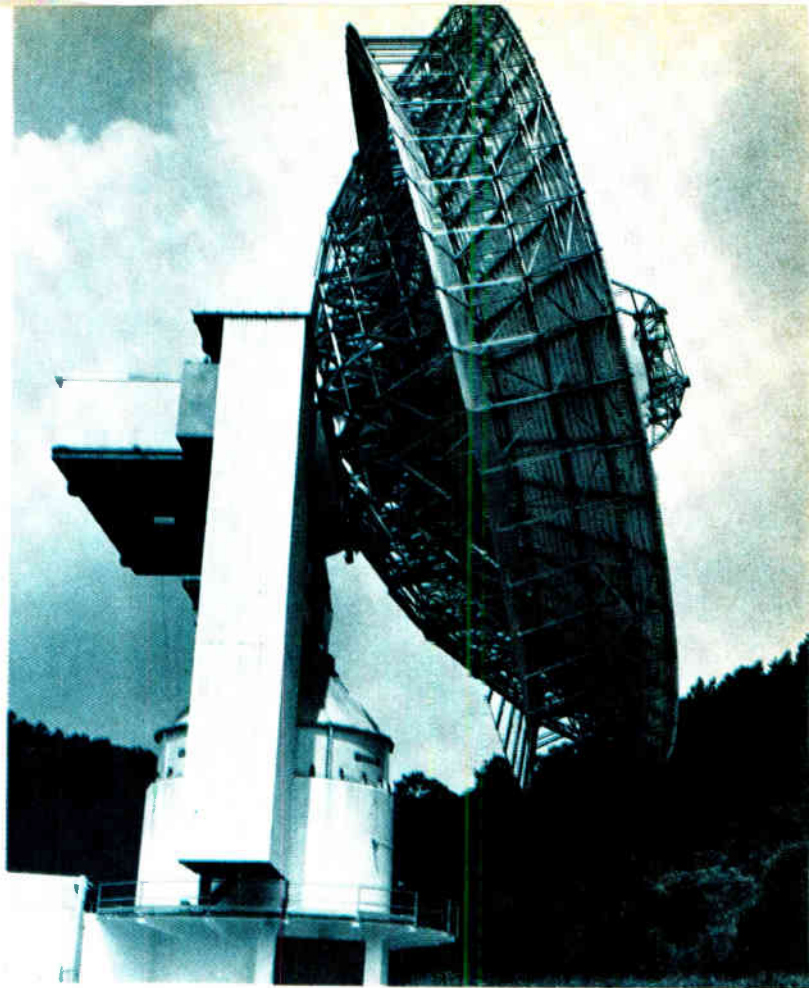
Towering. Earth stations, set up in the late sixties to communicate with the new satellites, were big. This one in Morgantown, W. Va., built by Philco-Ford's WDL division for Comsat Corp.'s Intelsat, has a 97-ft-diameter antenna, is 11 stories high, and weighs 470 tons.
