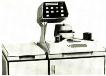
1967. First "hands off" wafer transport using patented air bearings was introduced.
