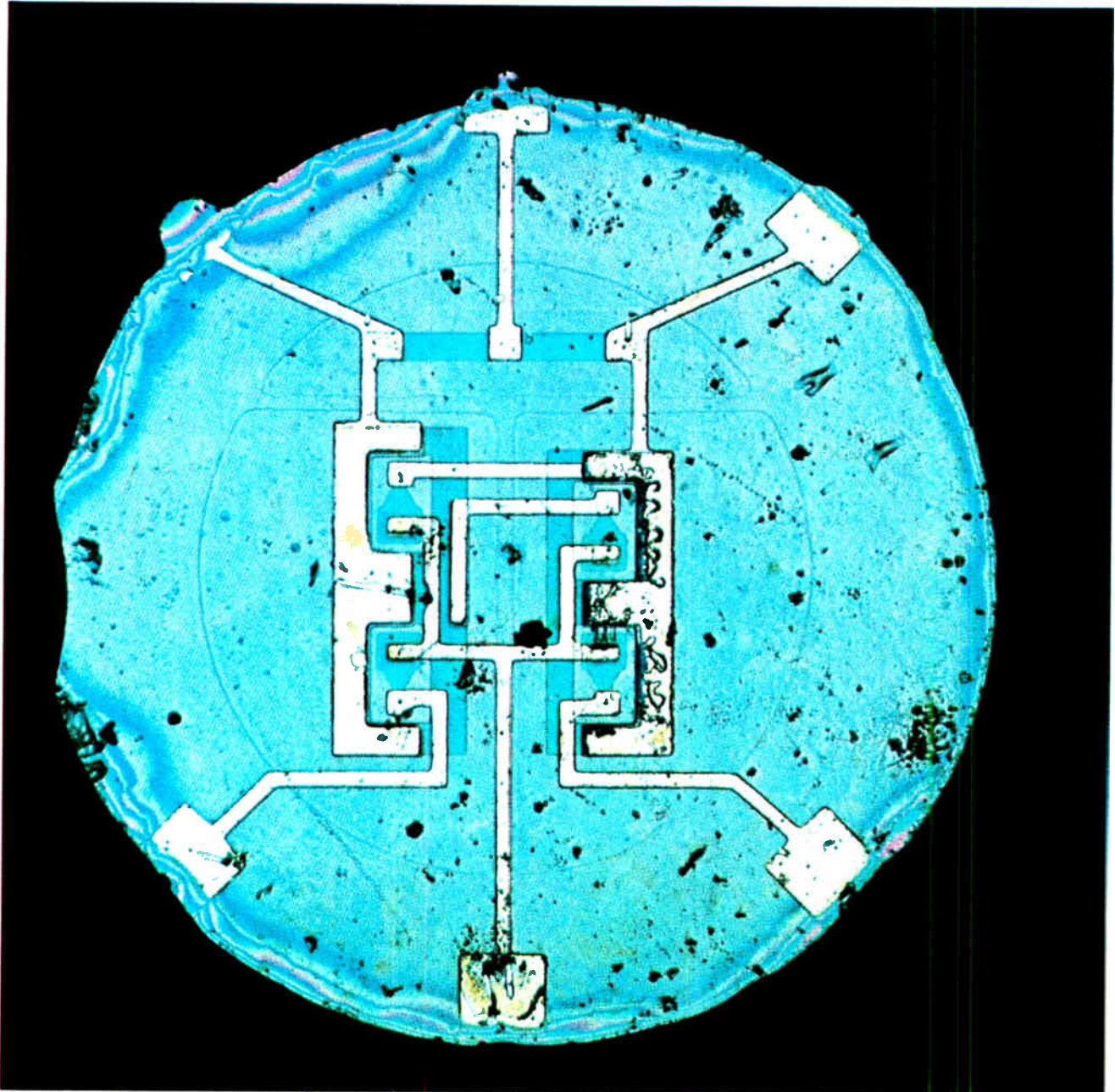
Flip-flop. The industry's first commercially available monolithic integrated circuit was this flip-flop from Fairchild Semiconductor, introduced in 1961. A member of the Micrologic family, the chip used resistor-transistor logic (RTL) and held four bipolar transistors and two resistors.
