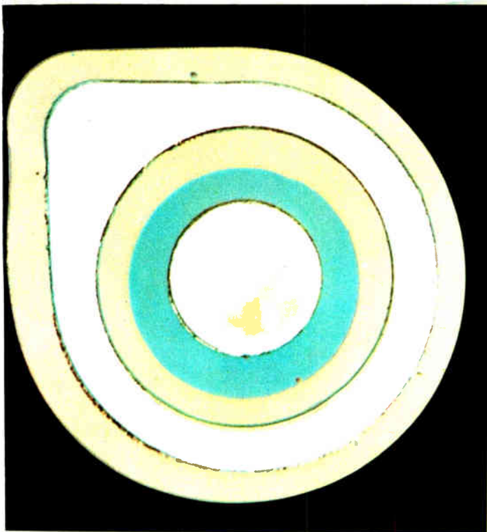
Planar. The transistor took on a new shape with Fairchild's planar process. So named because it was flat, the planar transistor diffused the emitter region (center) into the base region (tear shape), which itself was diffused into the collector substrate.
