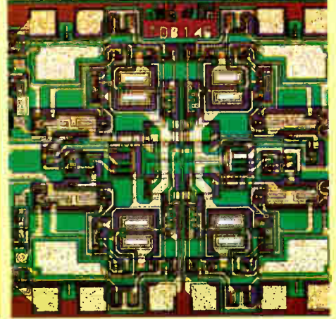
Quadruple op. amp. for active filters, telephone, ...
