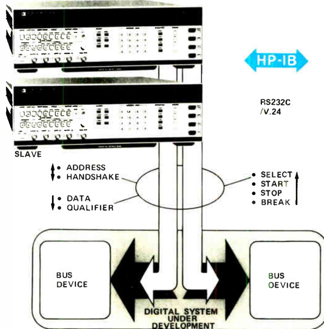
8170A LOGIC PATTERN GENERATOR - MASTER
