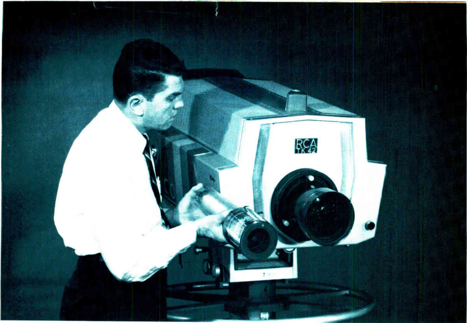
Camera. RCA's four-tube color TV camera, the TK-42, was introduced at the 1962 National Association of Broadcasters meeting. A 4½-inch-diameter image orthicon, shown, handled the monochrome channel. Color pickup was with 1-inch image orthicons.
