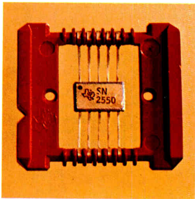
Flat pack. Handling tiny integrated circuits was a problem whose solution lay in the flat pack—a ceramic, plastic, or metal unit with flat-ribbon leads jutting from opposite sides. It was invented by Texas Instruments in 1962 and was soon an industry standard.
