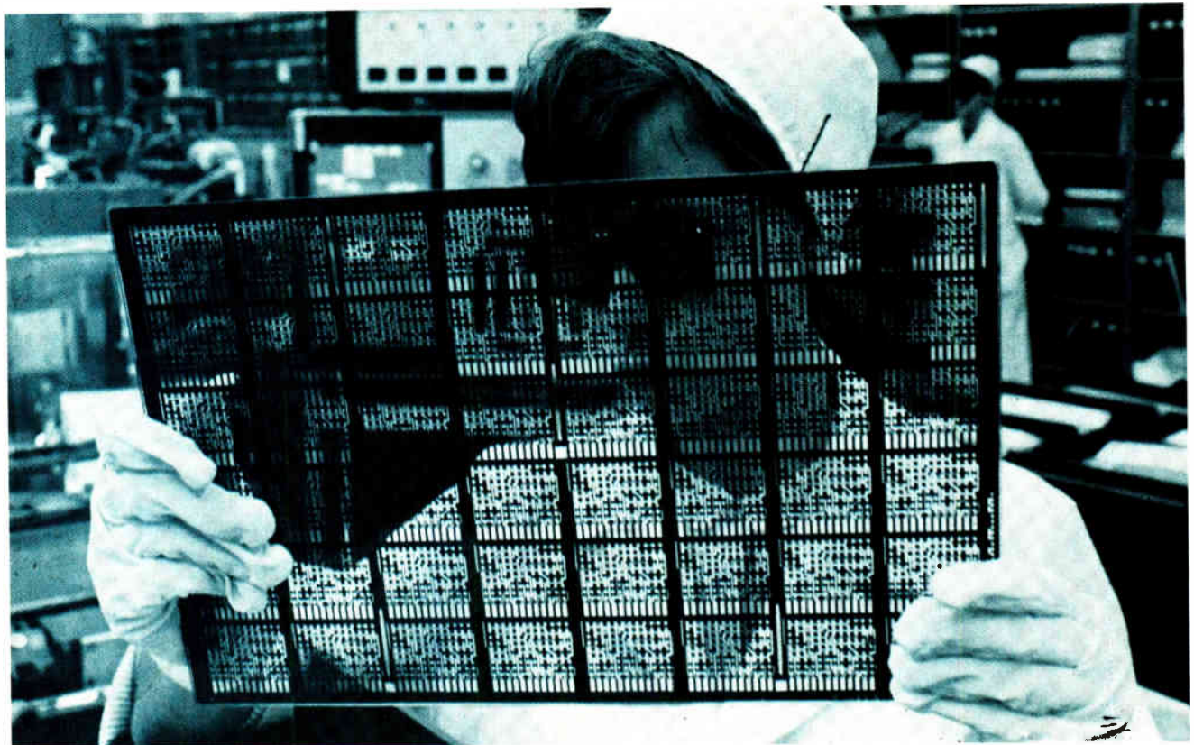
Master. Precision glass negative containing circuitry patterns for 48 etched printed-circuit cards for hybrid logic was fabricated for the System/360 line. Here it is inspected by a technician in a clean room before being inserted in an automatic photo-exposure machine.
