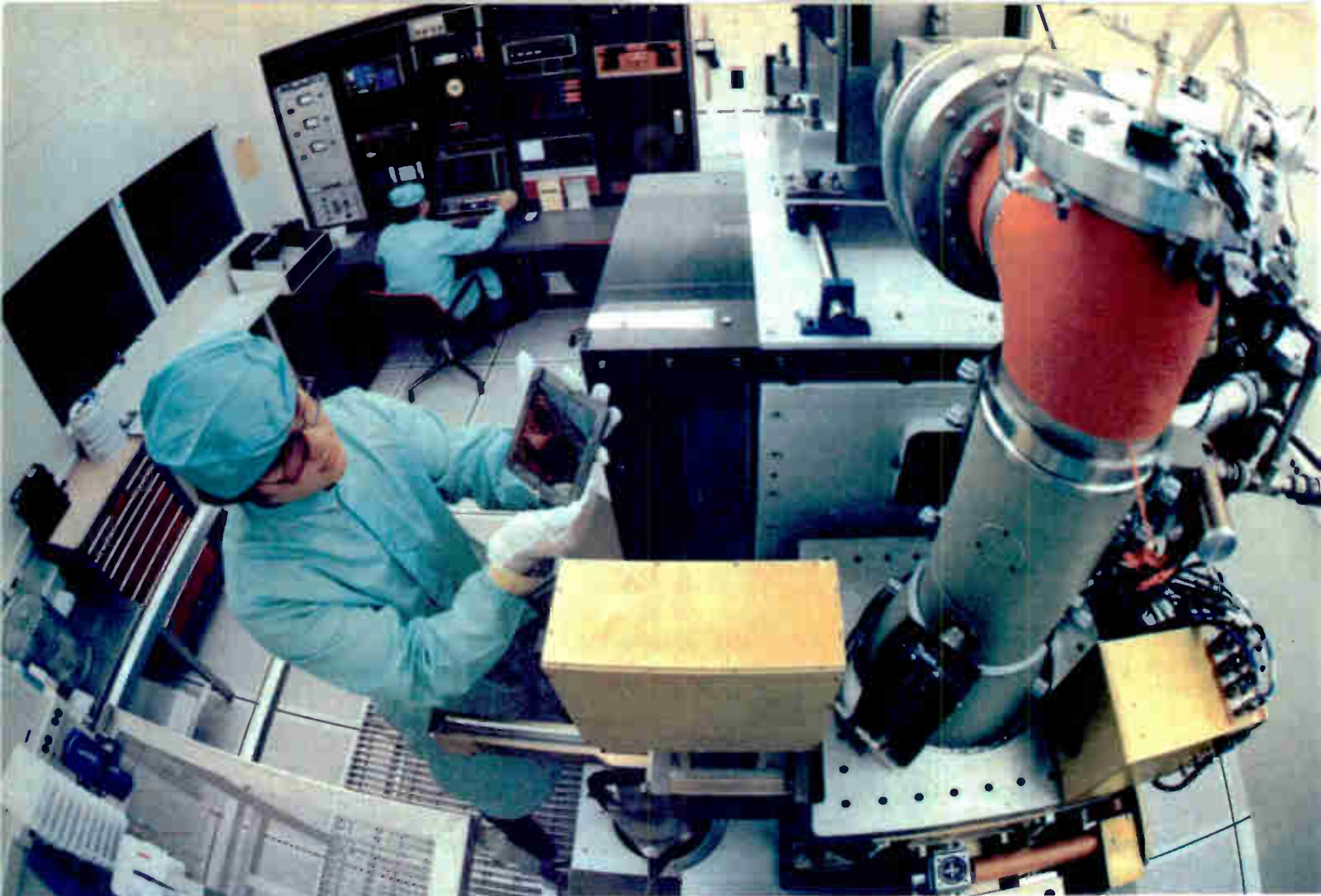
Electron-beam. An electron-beam exposure system, or EBES, was developed by Bell Laboratories and licensed to outside manufacturers. Here a technician holds a mask for LSI circuits before inserting it into such a machine at Western Electric's Allentown, Pa., works.
