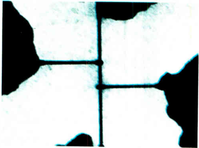
Even more slender. An experimental Josephson nanobridge developed by IBM switches without a junction. The lines in the circuit have widths and thicknesses of only 100 to 200 atomic diameters (30 to 40 nanometers). Electron beams exposed them.
