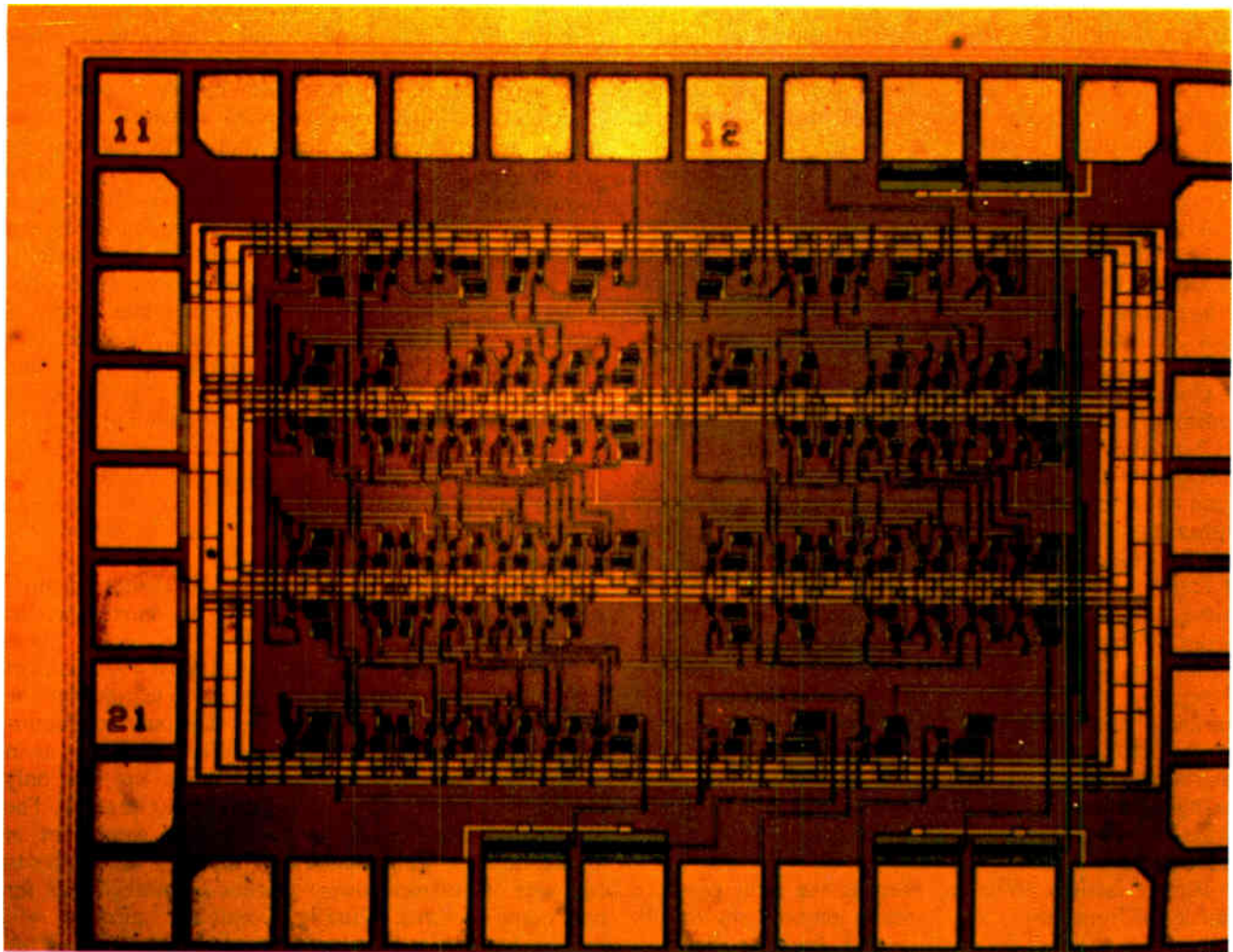
Gallium arsenide. To go beyond the speed of silicon, gallium arsenide with its enhanced mobility is one material to use. It has its own set of challenges, one of which is the inability to oxidize it for insulating layers. Still, circuits like this counter have been made.
