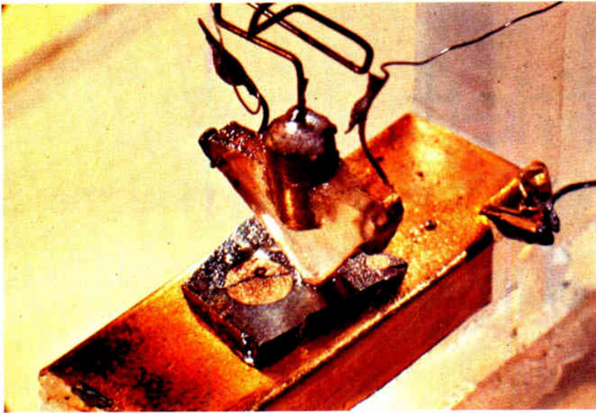
Solid amplifier. The first transistor placed two closely spaced contacts (the emitter and collector) on the surface of a germanium slab (the base). The V-shaped object is a plastic triangle round which gold foil was wrapped and slit at the apex with a razor; it was held on the slab by spring pressure.
