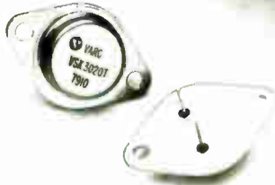
30A VSK30T Series: 20/30/40 V_{RRM} 0.64 V_F @ 15.0 A I_F
