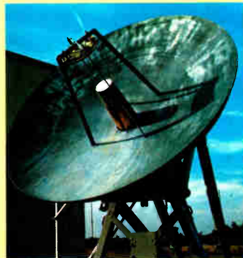
An 11-GHz, 3-meter diameter antenna, for communicating with France's first domestic satellite, TELECOM I, whose transmission capacity will be equivalent to 150 Mb/s.
