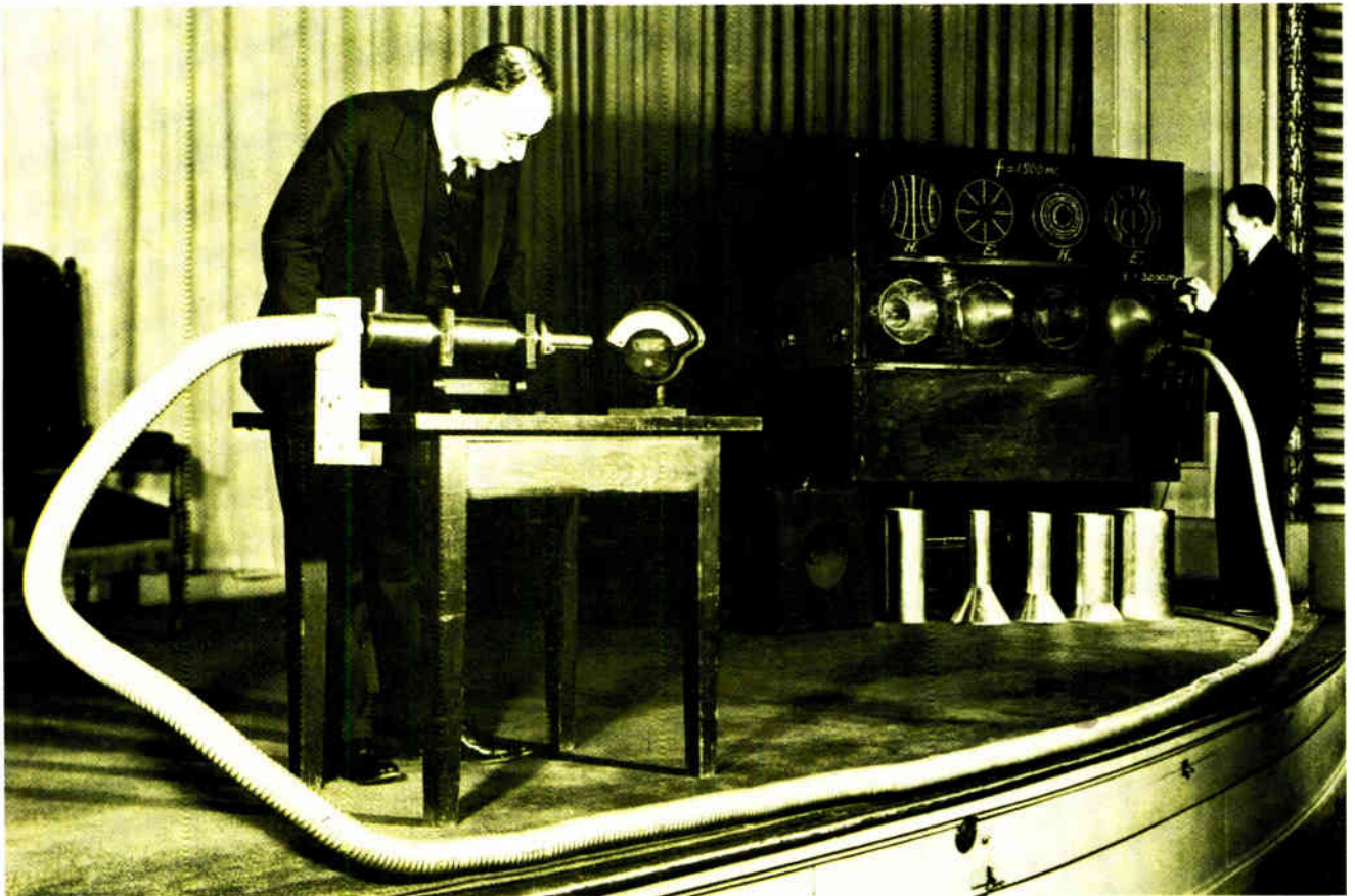
Guide. The work of Bell Telephone Laboratories' George Southworth represented a new way of thinking about radio waves. This photograph was taken at the first public demonstration of waveguide transmission before the Institute of Radio Engineers on Feb. 2, 1938.
