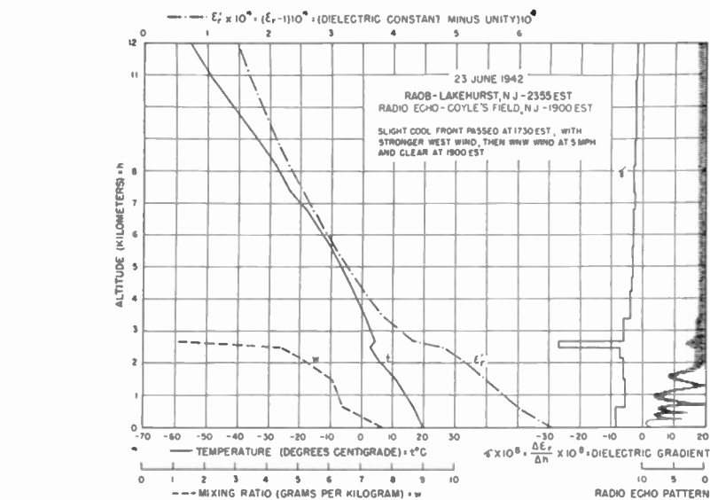
Fig. 1—RAOB and radio echo plots (June 23, 1942).
