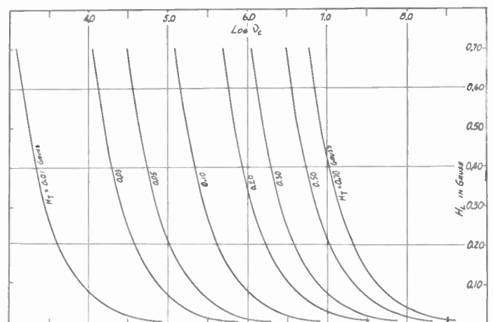
Fig. 3—Critical collisional frequency for various values of magnetic field.
