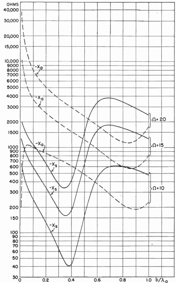
Fig. 15—Symmetrical and antisymmetrical reactances. β 0 h = π.
