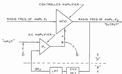
Fig. 1—A typical a.v.c. system.
