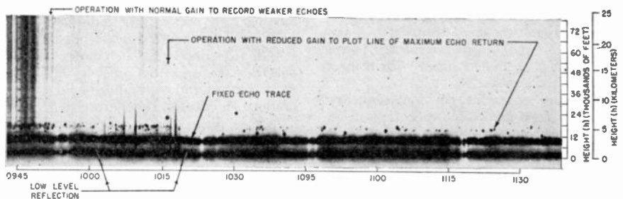
Fig. 3—Vertical beam radar sounding on 2800 Mc. on a perfectly clear day, modified AN/CPS-1 radar, Bedford Airfield, Mass., September 9, 1947, Eastern Standard Time. Weather, cloudless, visibility and ceiling unlimited; surface wind, S.E. 5 m.p.h.
