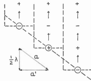
Fig. 7—Oblique array.
