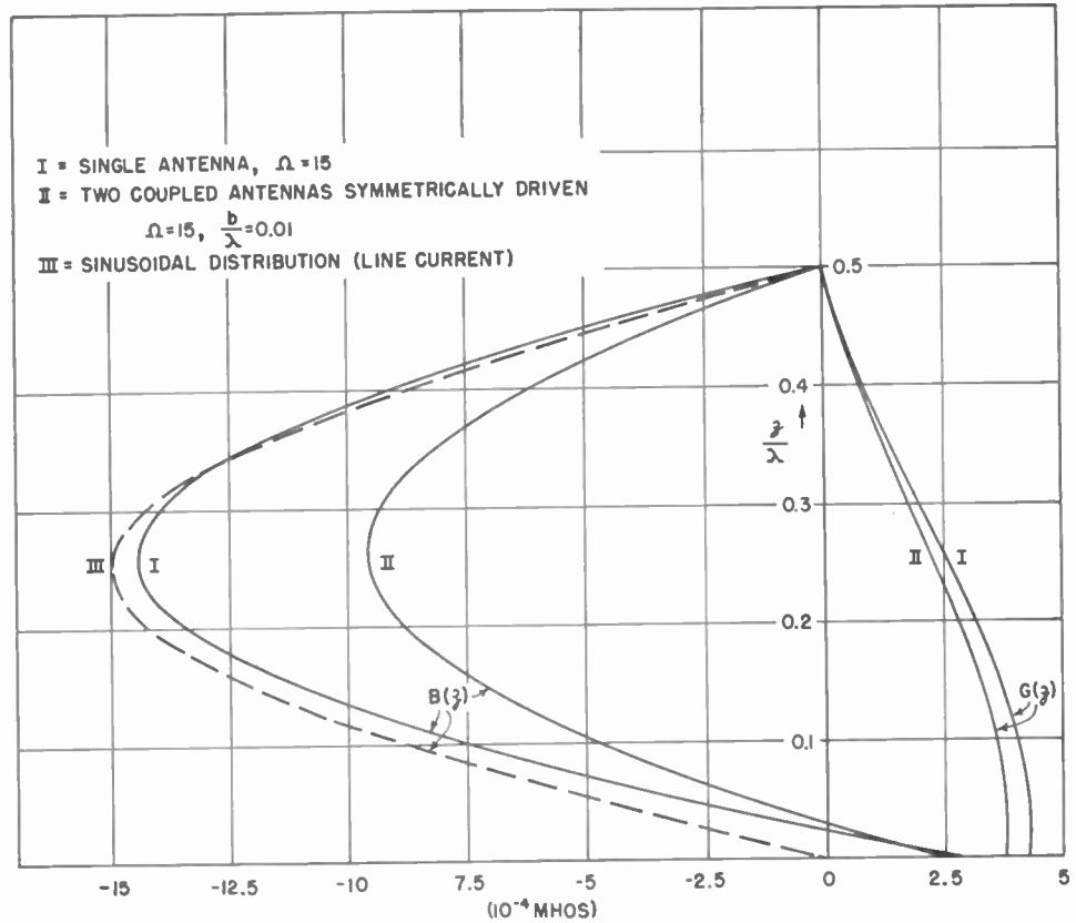
Fig. 11—First-order current distribution for h = \lambda/2 .
