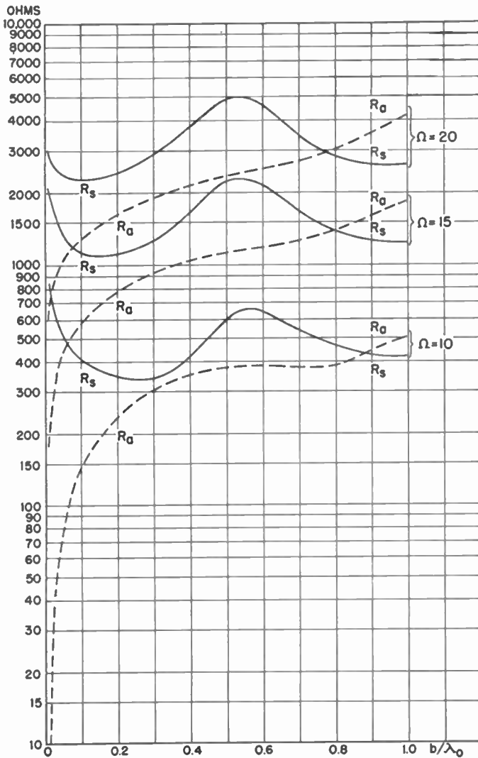
Fig. 14—Symmetrical and antisymmetrical resistances. β 0 h = π.
