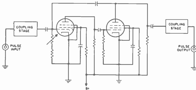
Fig. 4—Multivibrator used as protection against interference.
