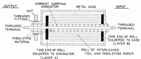
Fig. 1—Method of construction of the duct capacitor.
