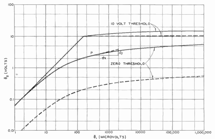
Fig. 7—A.v.c. regulation characteristics.
