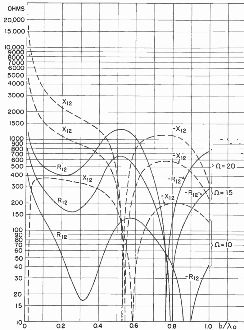
Fig. 18—Mutual impedance, \beta_0 h = \pi .
