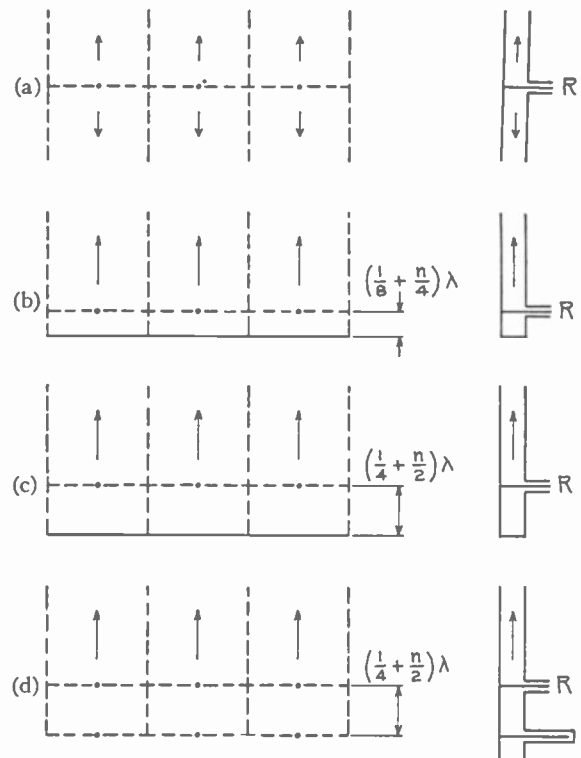
Fig. 3—The flat array with front and back radiation or reflection, and the equivalent transmission lines. (a) Front and back radiation. (b) Plane reflector for same resistance. (c) Plane reflector for double resistance. (d) Array reflector.
