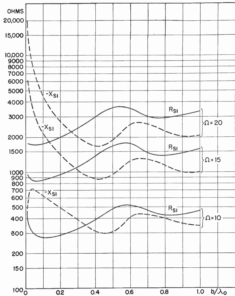
Fig. 17—Self-impedance, \beta_0 h = \pi .
