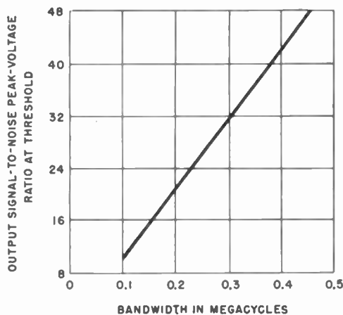
Fig. 7—Signal-to-noise ratio plotted against bandwidth for thermal agitation noise and signal-pulse displacement of \pm 8 \mu\text{s} .
