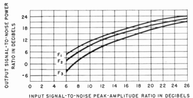
Fig. 8—Output signal-to-noise power ratio plotted against input signal-to-noise peak-amplitude ratio for 3- \mu\text{s} . noise pulse having repetition frequencies of F_1=250 , F_2=500 , and F_3=1000 . No protection.
