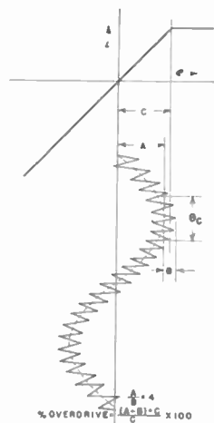
Fig. 6—Single-ended, sharp-cutoff characteristic with a two-frequency input signal.
