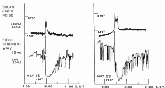
Fig. 2—Solar noise bursts and sudden ionospheric disturbances.
