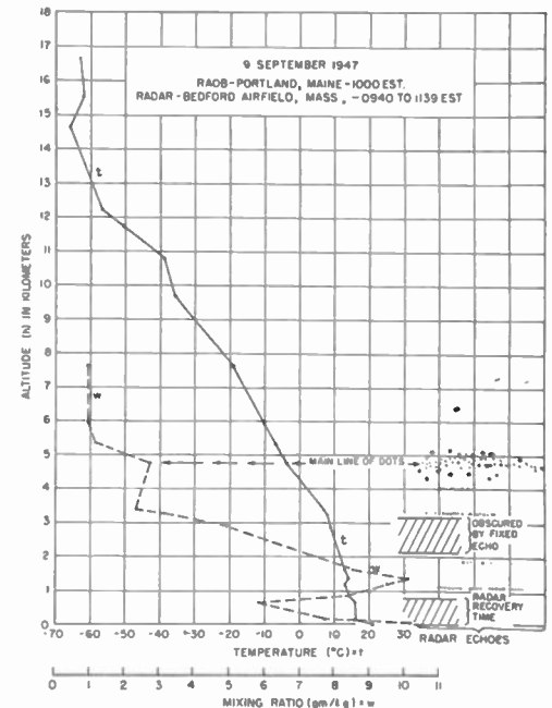
Fig. 4—RAOB and 2800-Mc. radar echo plots
