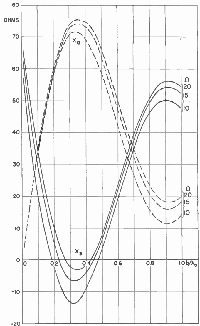
Fig. 13—Symmetrical and antisymmetrical reactances. \beta_0 h = \pi/2 .
