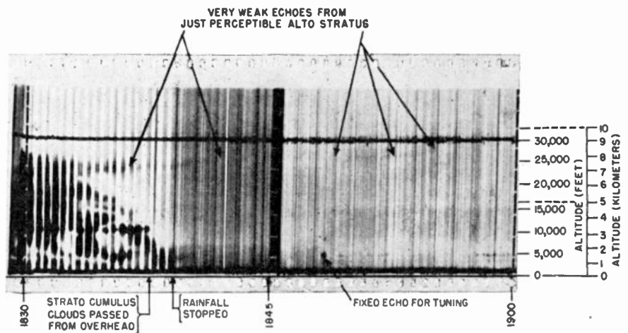
Fig. 2—Light frontal shower with large raindrops, vertical beam radar sounding on \lambda = 10 cm. with variable gain sweep, modified SCR-584 radar. East Lexington, Mass. July 31, 1947, Eastern Standard Time.
