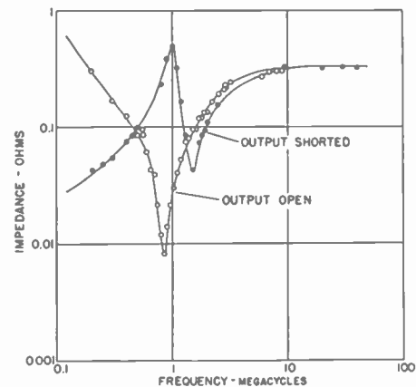
Fig. 8—Input-impedance characteristics of the 2.5- \mu fd. duct capacitor illustrated in Fig. 3.
