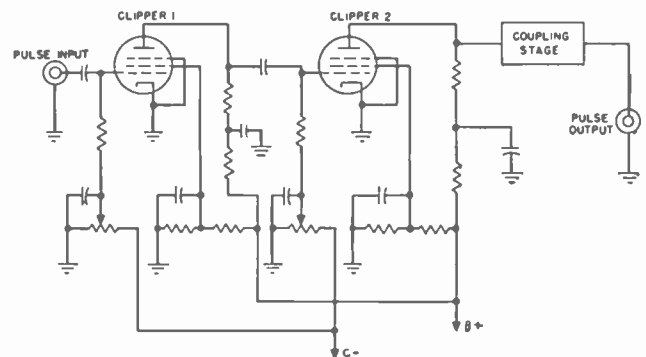
Fig. 3—Double-gate limiter used as protection against interference.
