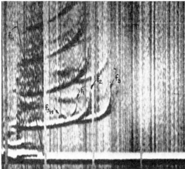
Fig. 1—Experimental evidence of magnetoionic multiple refraction.
