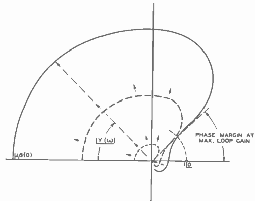
Fig. 3—Nyquist diagram of a stable a.v.c. system.
