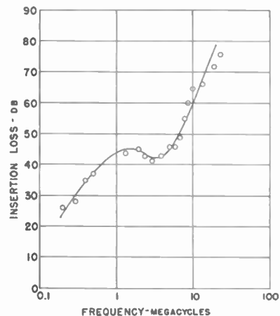
Fig. 5—Typical insertion-loss characteristic of a 2.5- \mu fd. duct capacitor as measured in the standard 20-ohm circuit.
