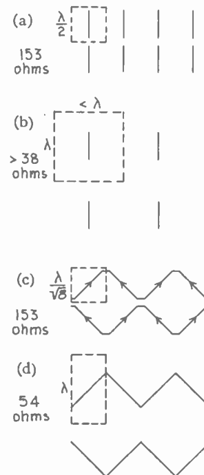
Fig. 5—Arrays of half-wave dipoles in image relations, with reflector. (a) Vertical antennas, normal spacing. (b) Same, maximum spacing. (c) Diagonal antennas, normal spacing. (d) Same, maximum spacing.
