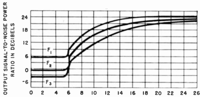
Fig. 9—Conditions similar to Fig. 8, but with double-gate limiter.
