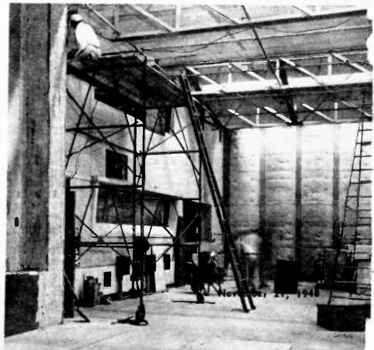
▶ A PARTIAL VIEW OF NBC'S TELEVISION STUDIO F in Hollywood shows workman on scaffolding installing wiring. The construction work was finished November 1, and KNBC expects to be telecasting commercially on Channel 4 by January 1, 1949. (NBC photo.)
