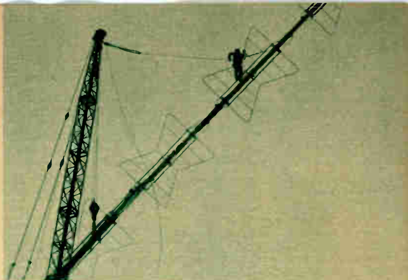
2. TWO DAYS LATER. WORKMAN HANGS precariously on one of the five "bat-wing" sets. KNXT tower is built to stand stress of 110-mile wind with one inch of ice on the tower and 130-mile wind without. Weave in wind is maximum fourteen inches.
