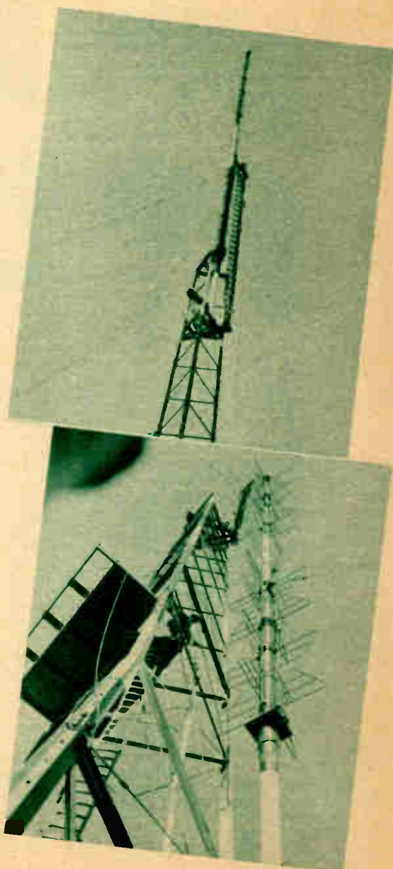
2. TWO DAYS LATER. WORKMAN HANGS precariously on one of the five "bat-wing" sets. KNXT tower is built to stand stress of 110-mile wind with one inch of ice on the tower and 130-mile wind without. Weave in wind is maximum fourteen inches.
