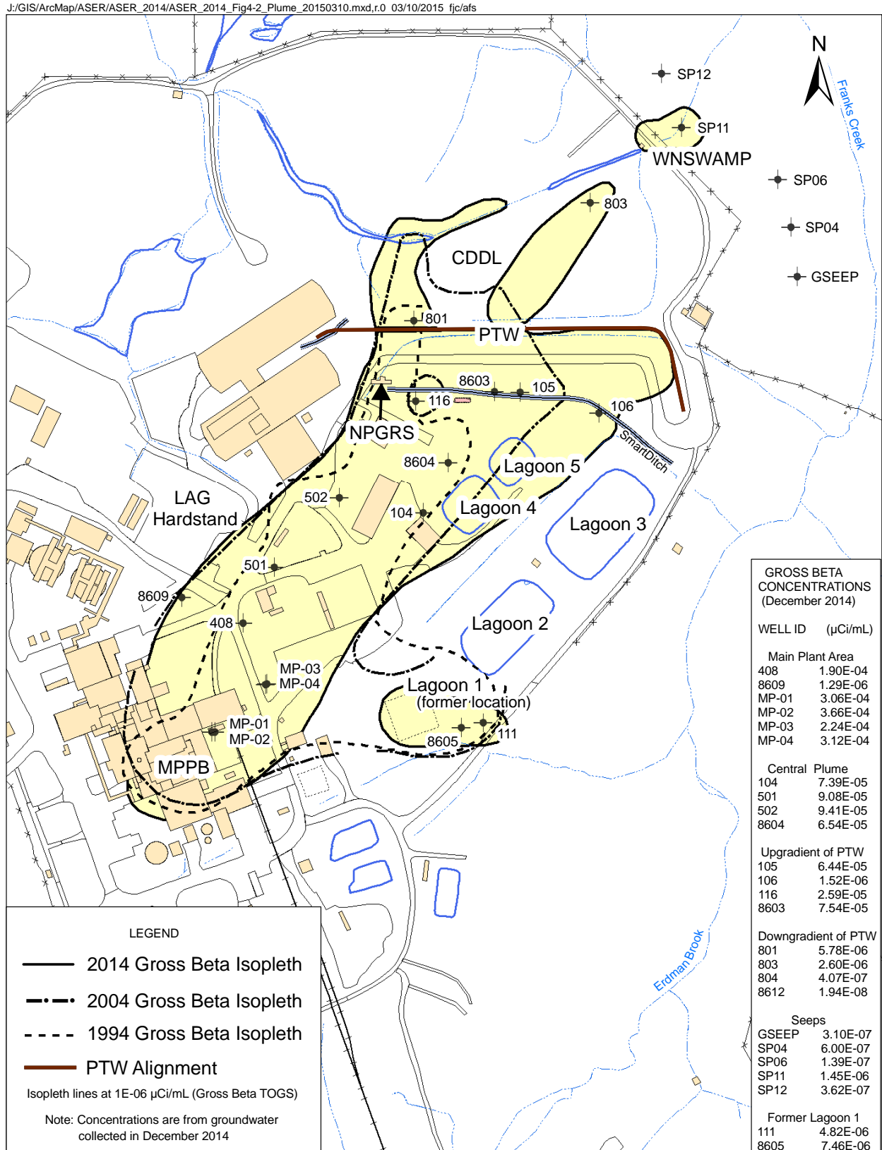
FIGURE 4-2 North Plateau Strontium-90 Plume Plotted by Beta Data: 1994, 2004, 2014
