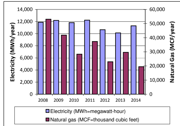
FIGURE 1-1 Energy Use
