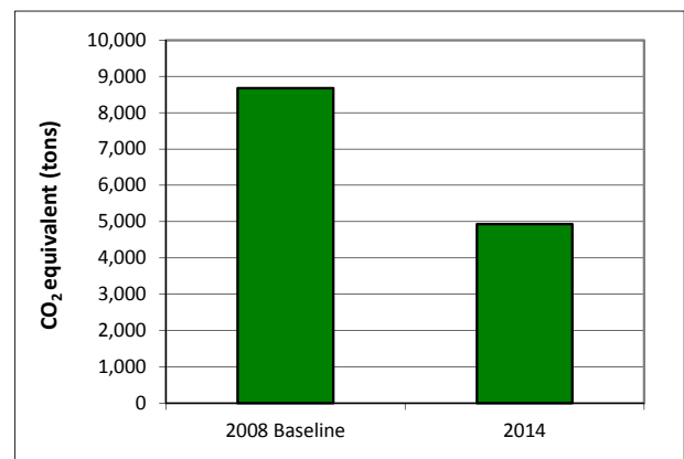
FIGURE 1-2 GHG Emissions
