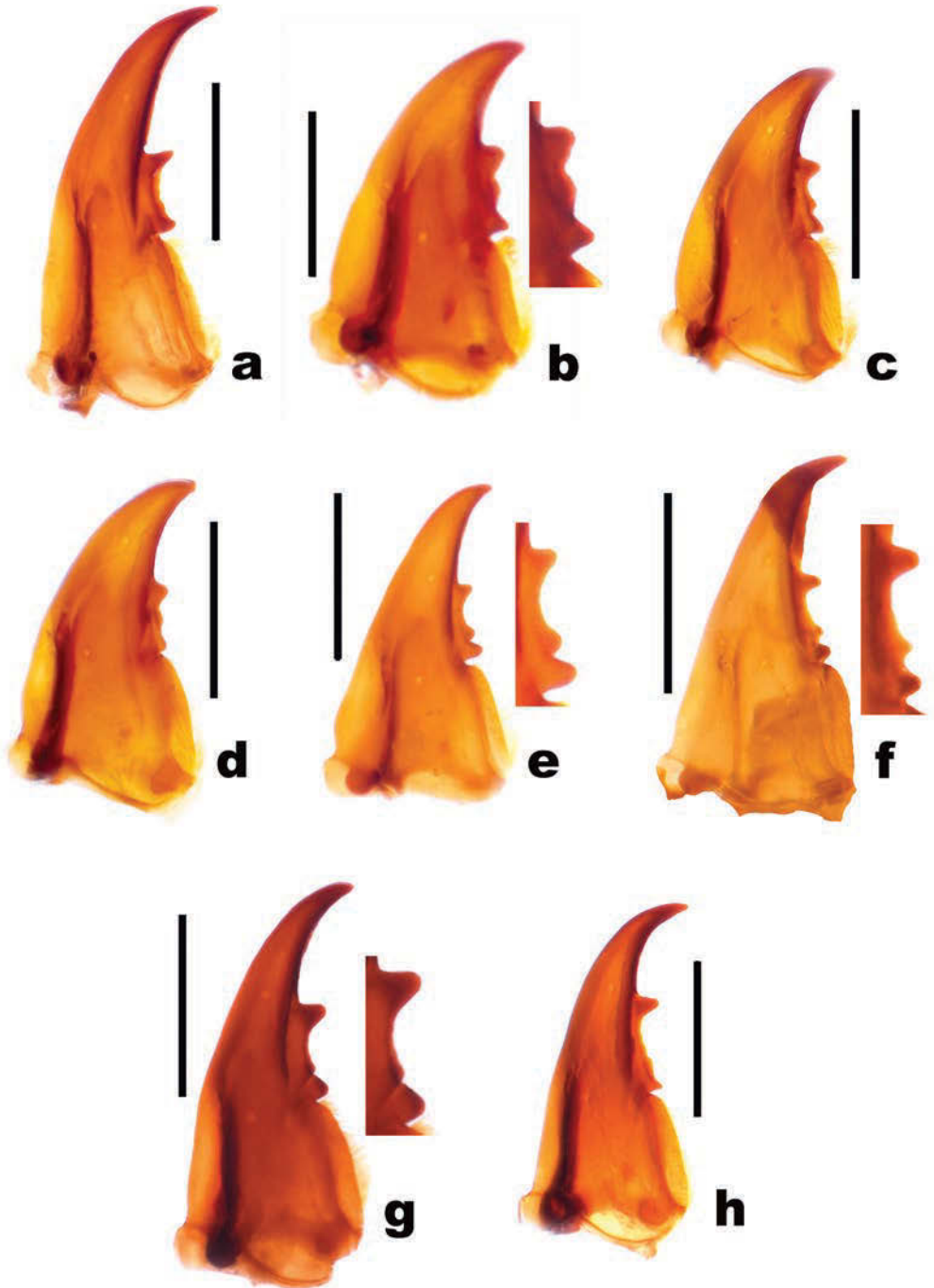
FIGURE 16. Trechine right mandibles, ventral aspect. a. Agonotrechus xiaoheishan sp. nov. b. Trechus indicus Putzeys with dentition enlarged. c. Trechus gongshanensis sp. nov. d. Trechus shibalicus sp. nov. e. Pseudepaphius gonggaicus Deuve with dentition enlarged (China, Sichuan Province, Moxi Township, NE slope of Gongga Shan). f. Trechepaphiopsis uniporosa sp. nov. with dentition enlarged. g. Epaphiotrechus fortipesoides sp. nov. with dentition enlarged. h. Trechepaphiama gaoligong sp. nov. Scale lines = 0.5 mm.
