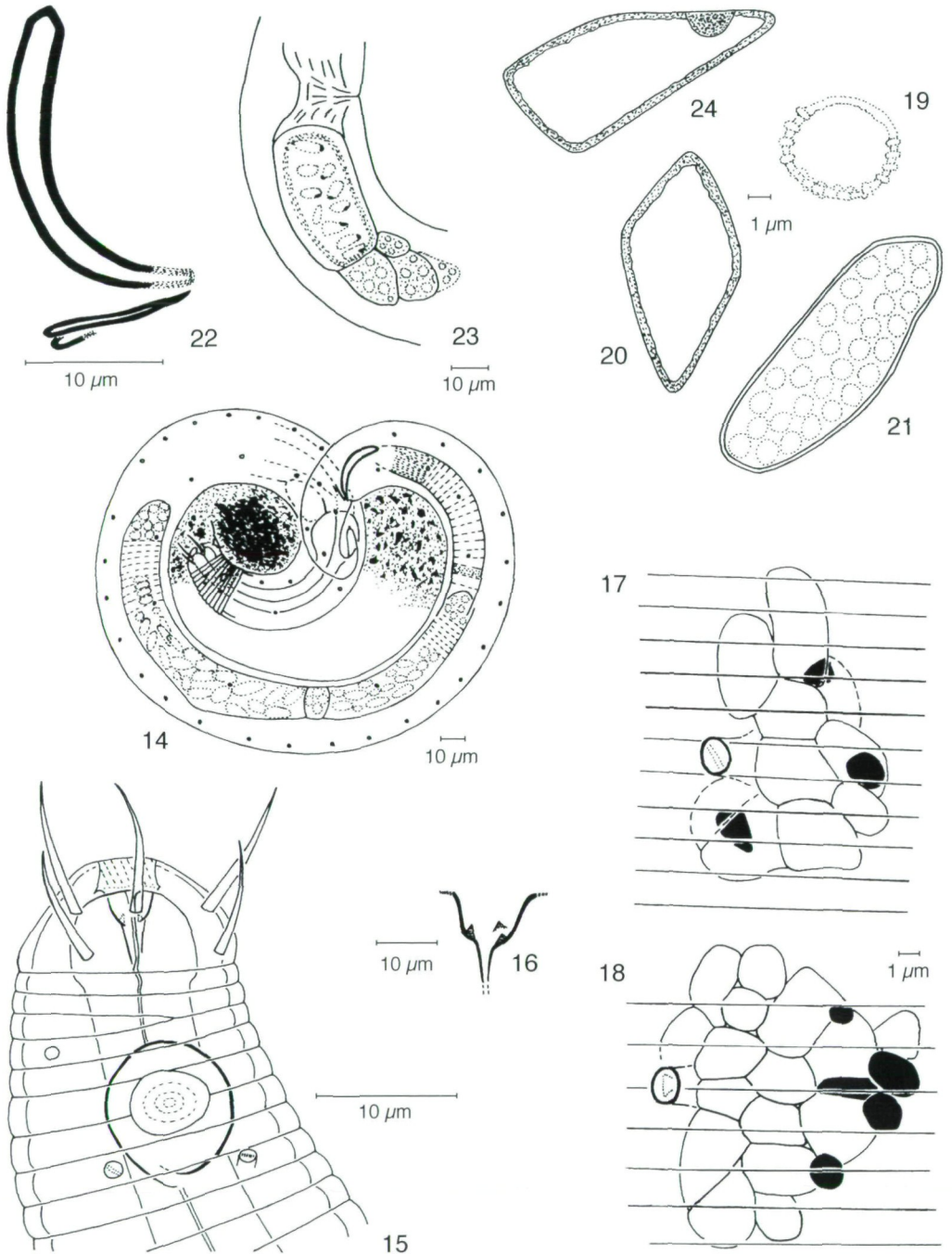
Figs. 14-24: Microlaimus discolensis sp.n.. Habitus (14) and head (15) of ♂; buccal cavity of ♀ 2 (16); epidermal gland and pore of ♂ 1 (17) and ♀ 1 (18); sperm cells of young (19, ♂ 1 ), medium (20, ♂ 2 ), and old (21, ♂ 1 ) developing stage; copulatory apparatus of ♂ 1 (22); vulvar region of ♀ 1 (23); sperm cell inside the reproductive organs of ♀ 1 (24).
