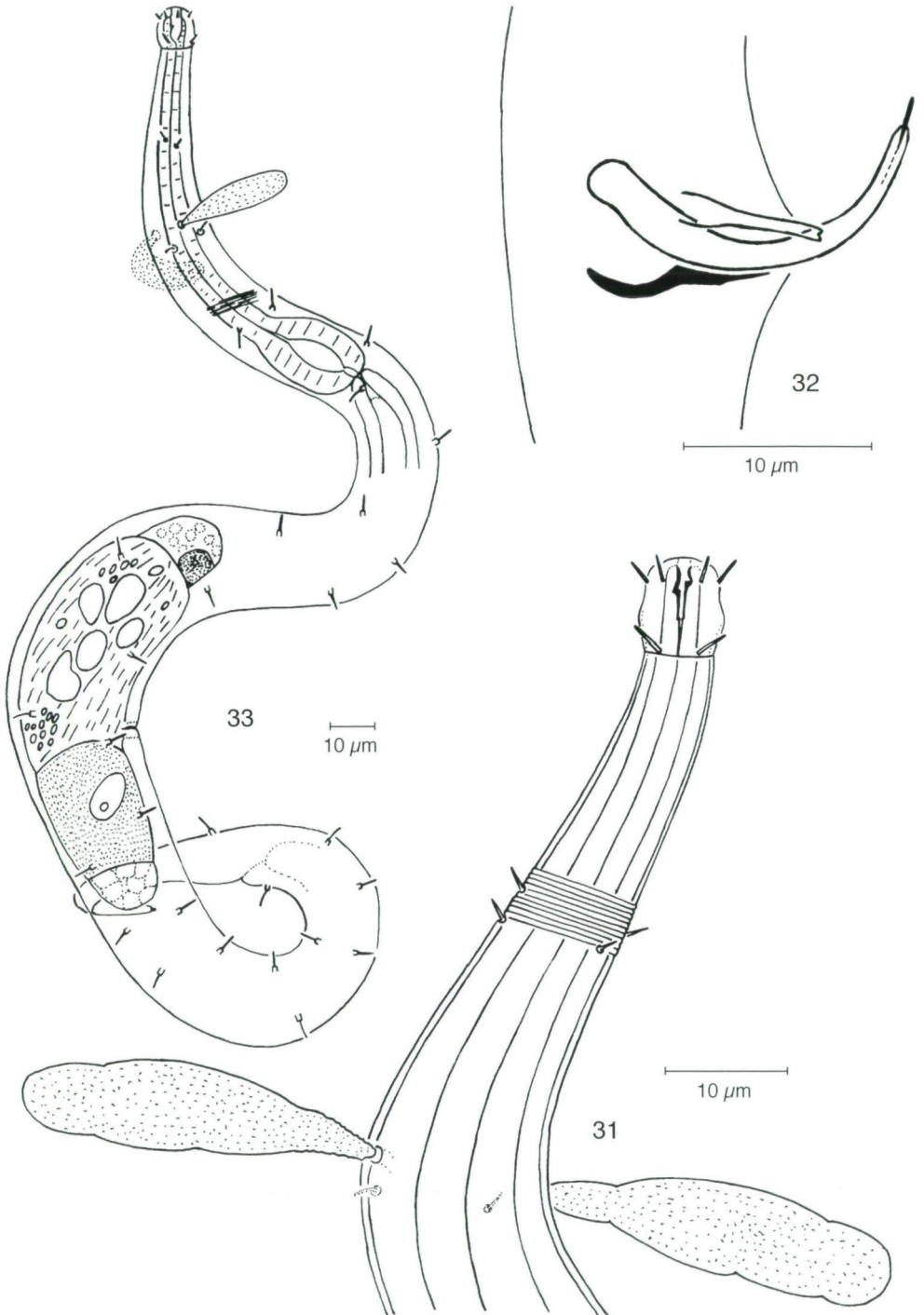
Figs. 31-33: Bathynox clavata gen.n. sp.n. Anterior body (31) and copulatory apparatus (32) of \sigma_1 ; habitus of \varphi_1 (33).
