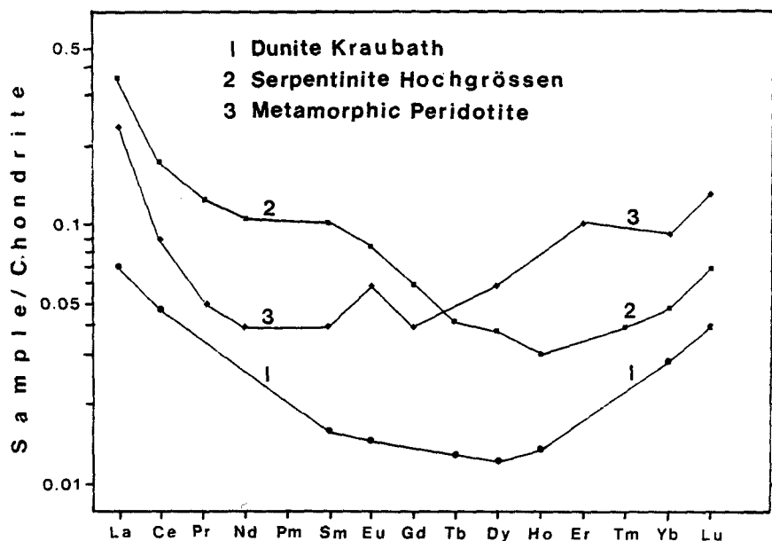
Fig. 7: Rare earths elements (REE) in Kraubath and Hochgrössen ultramafic rocks (from EL AGEED, SAAGER and STUMPFL, 1980). Note that, compared to Kraubath, average light REE abundances of Hochgrössen ultramafics are higher by a factor of 4. This suggests fractionation from an REE-enriched liquid and underlines the refractory nature of the Kraubath rocks.
