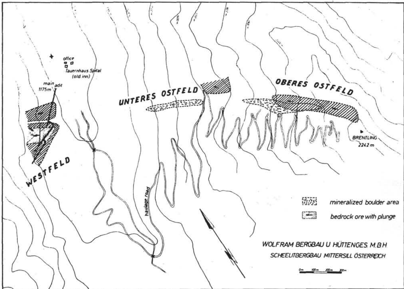
Fig. 14: Locality map, Mittersill Scheelite Mine. Difference of altitude is almost 1100 m over a horizontal distance of 2000 m. (Courtesy, Dr. R. Vaché, Wolfram Bergbau GmbH).
