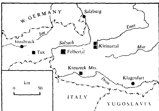
Fig. 12: Major scheelite occurrences in Austria (from STUMPFEL, 1977). Felbertal (Mittersill) is, at present, the only producing mine.
