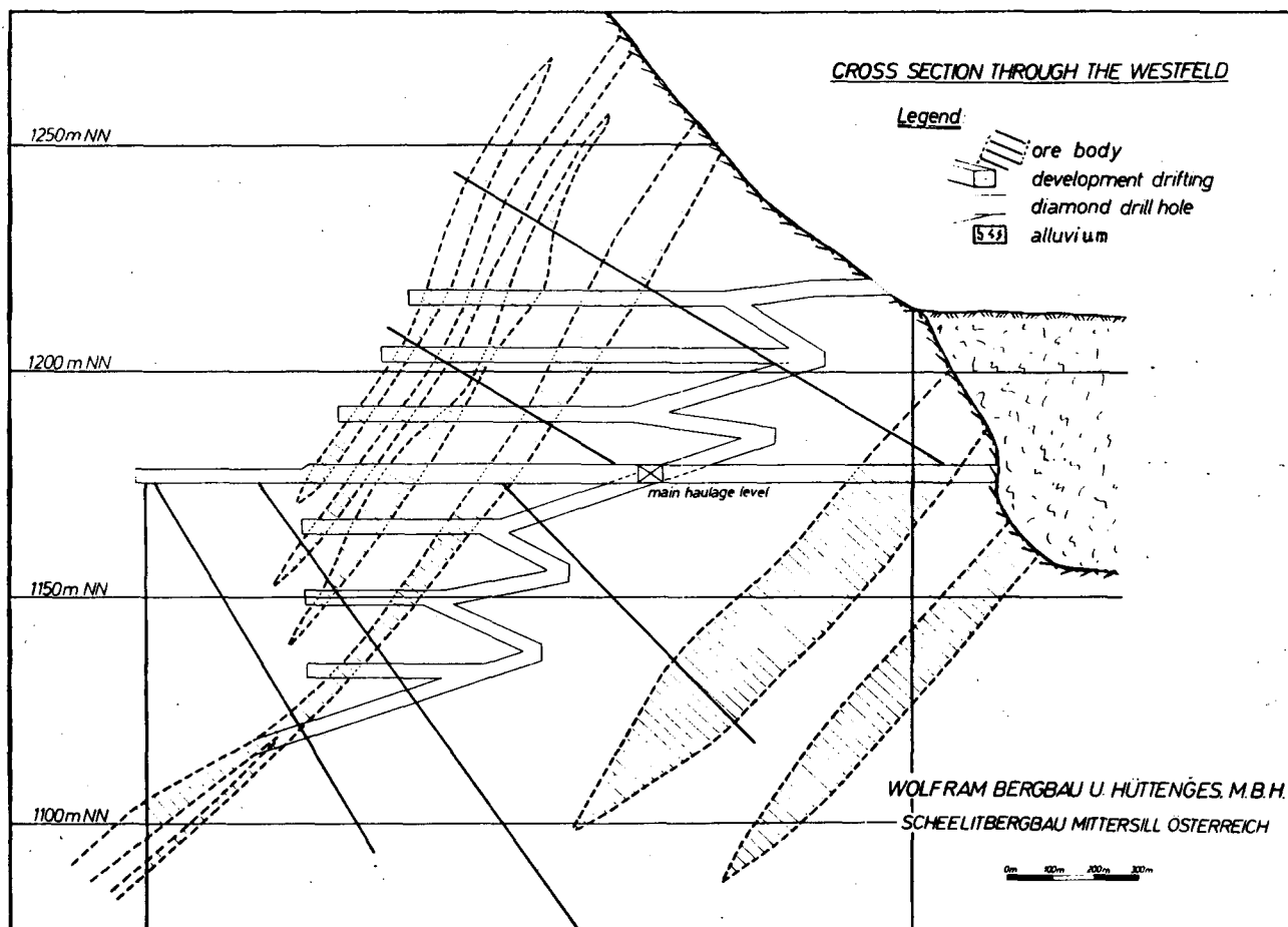
Fig. 15: Mittersill Scheelite Mine, section through the Westfeld (Courtesy, Dr. R. Vaché, Wolfram Bergbau GmbH).
