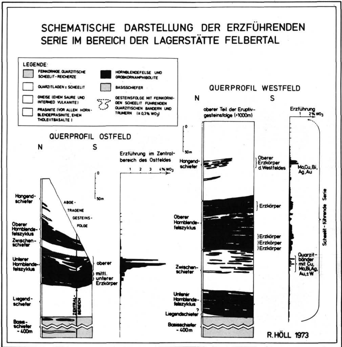
Fig. 16: Generalized stratigraphy of the Felbertal Scheelite Mine. After HÖLL, 1973.
