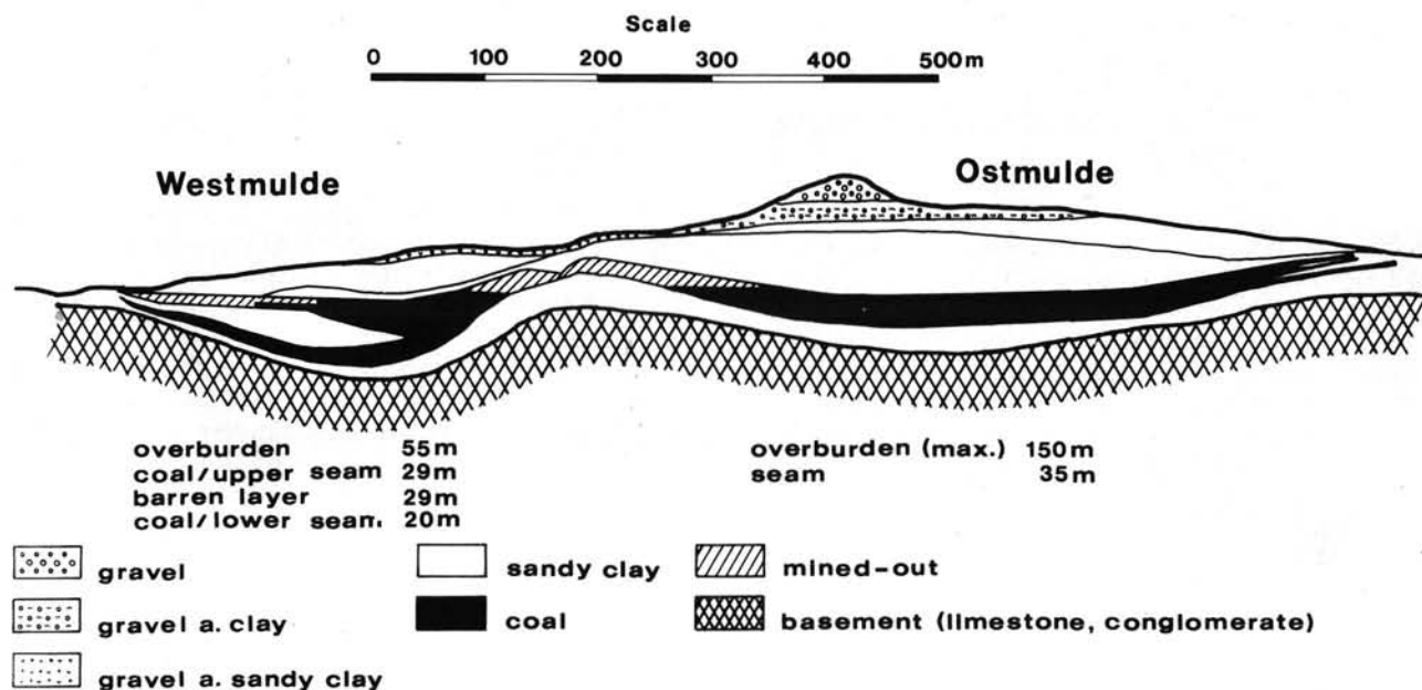
Fig. 3: Cross section of the lignite basin of Köflach—Voitsberg.
