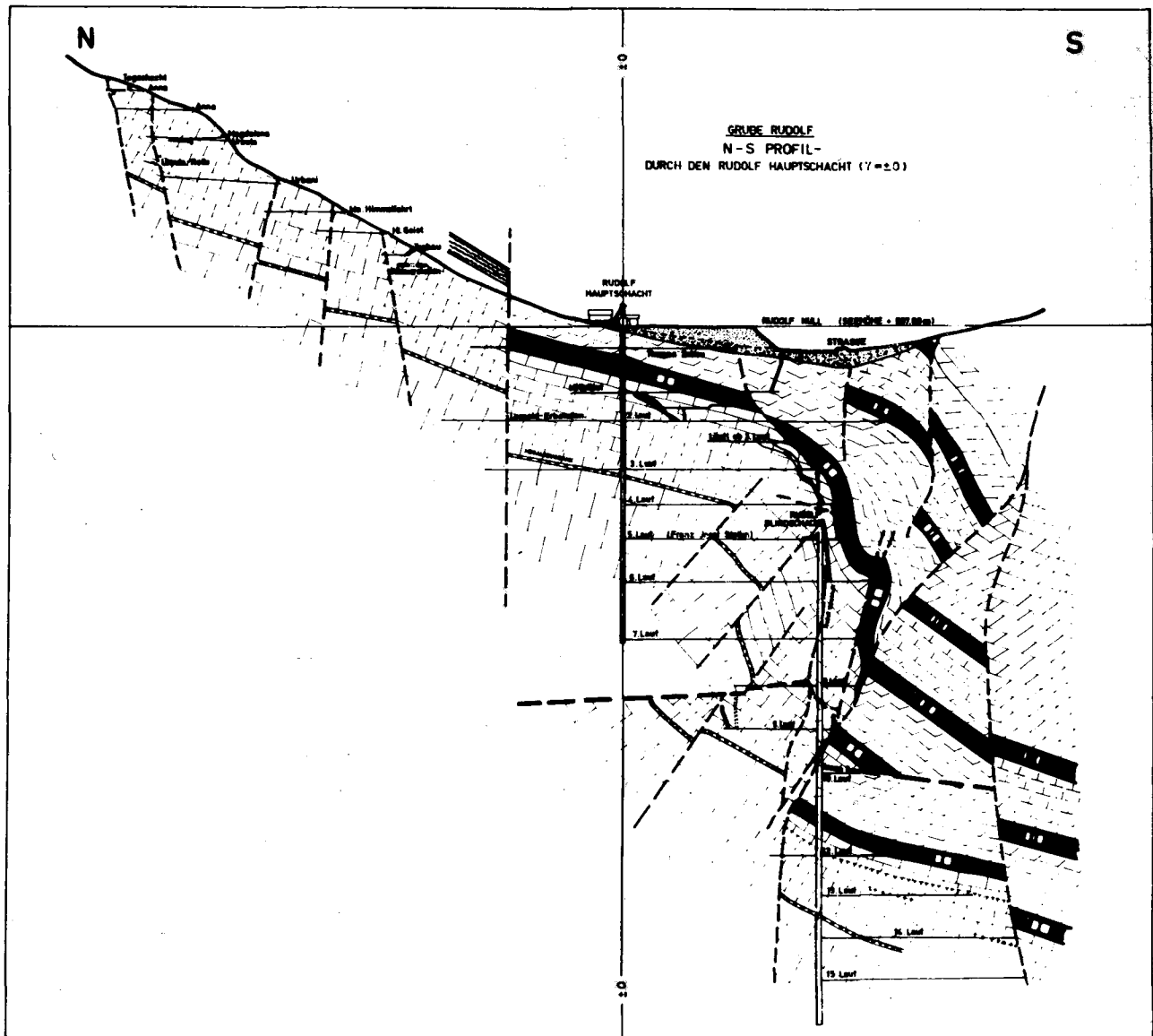
Fig. 11: Bleiberg Lead-Zinc Mine. Section through the workings of the Rudolf Shaft (after BOUVIER et al., 1972). Note the Megalodus Bank, an important stratigraphic marker. "Lauf" = level.
