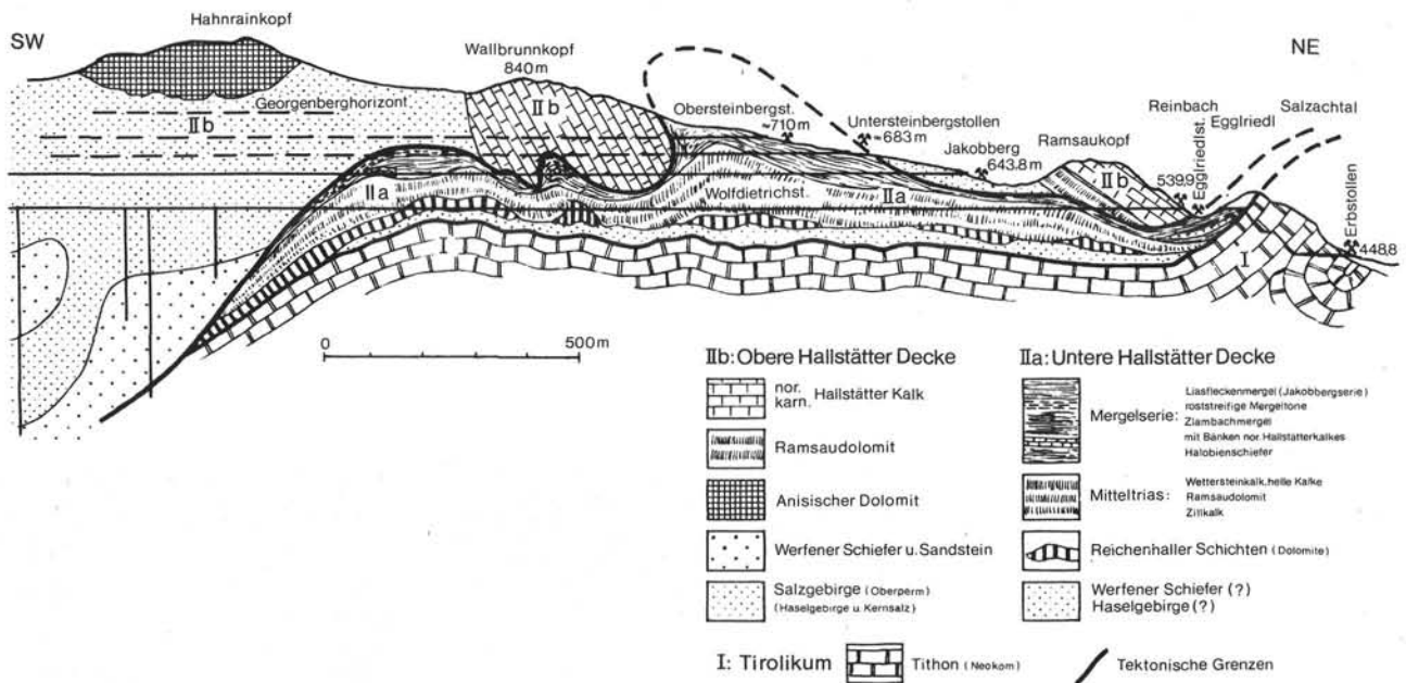
Fig. 17: Geological cross section through the Hallein Salt Deposit. After MEDWENITSCH, 1963.
