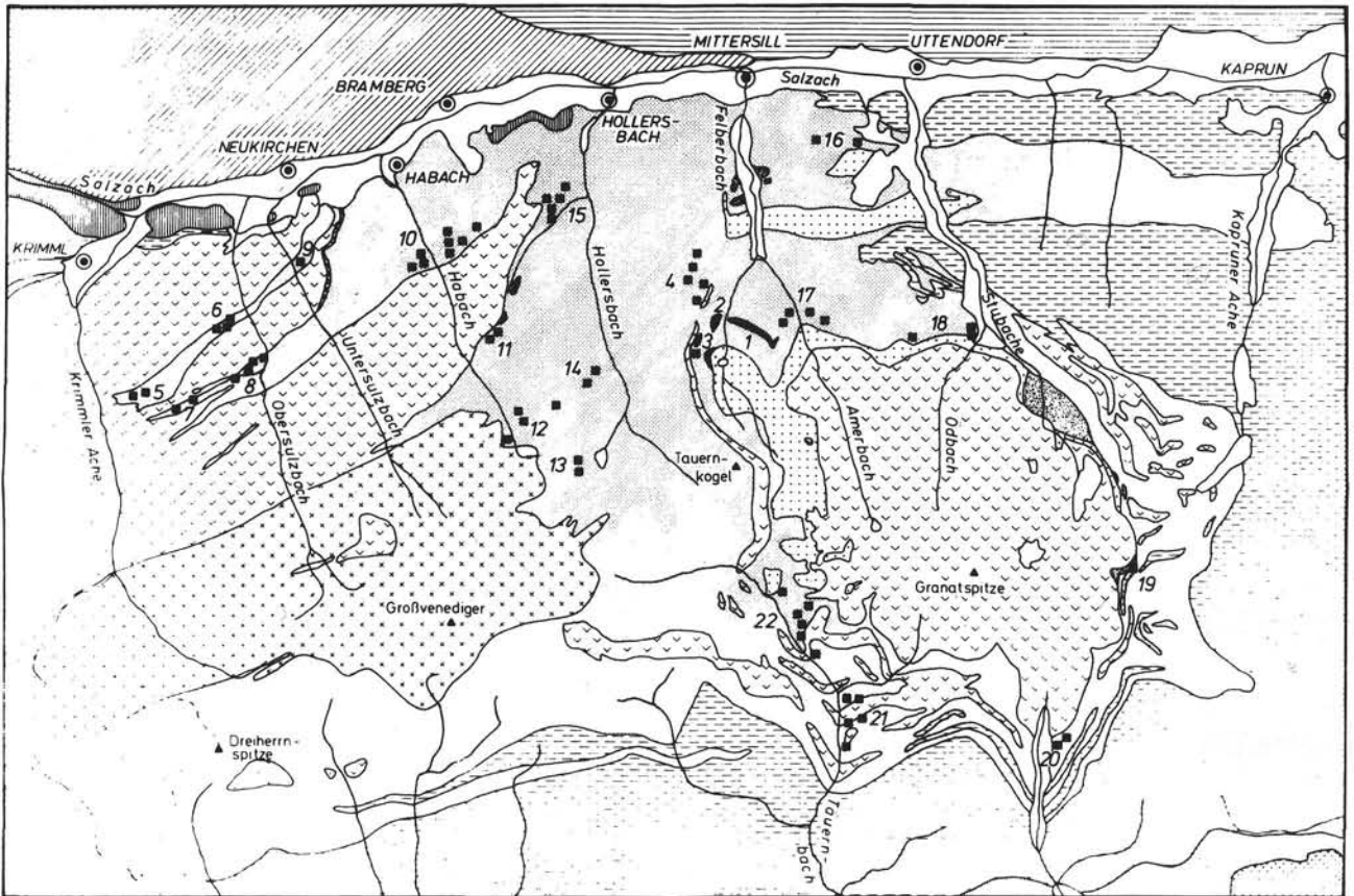
Fig. 13: Scheelite occurrences in the Hohe Tauern area (from HÖLL, 1975). Finely dotted = Habach Series within the Schist Cover; x = granitic and v = tonalitic Central Gneiss; coarsely dotted = basal amphibolites; horizontal stripes = Greywacke Zone, diagonal stripes = Quartz Phyllite Zone. "1" = Felbertal deposit, Ostfeld; "2" = Felbertal deposit, Westfeld. Other numbered occurrences are presently not of economic significance. Scale: width of map = 47 km.
