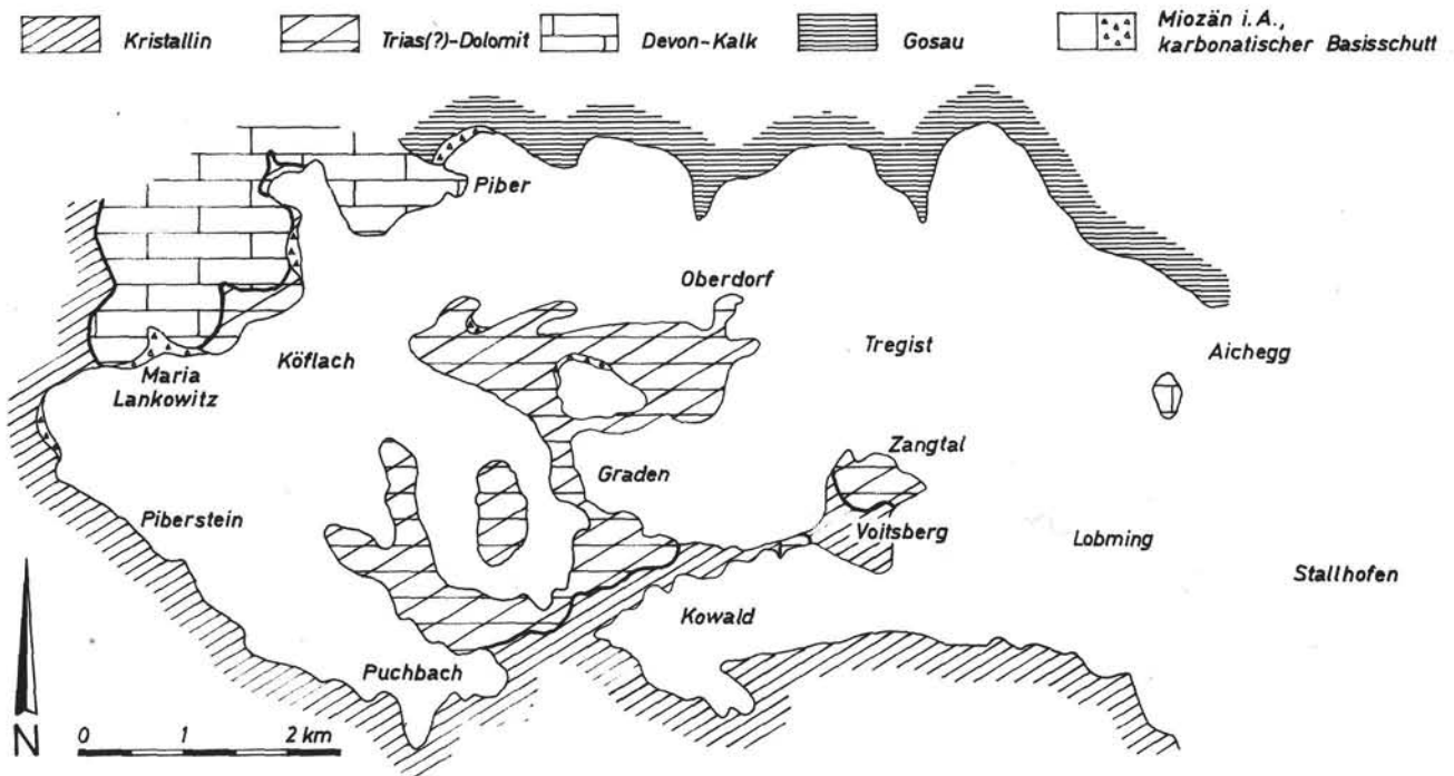
Fig. 1: Geological map of the lignite basin of Köflach—Voitsberg. After W. POHL, 1976.
