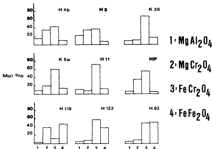
Fig. 6: Molecular proportions in chromites from the Kraubath (K 36, K 6 a) and Hochgrößen ultrabasic massifs (analysis numbers with prefix "H"), calculated from electron microprobe analyses (EL AGEED, 1979).
