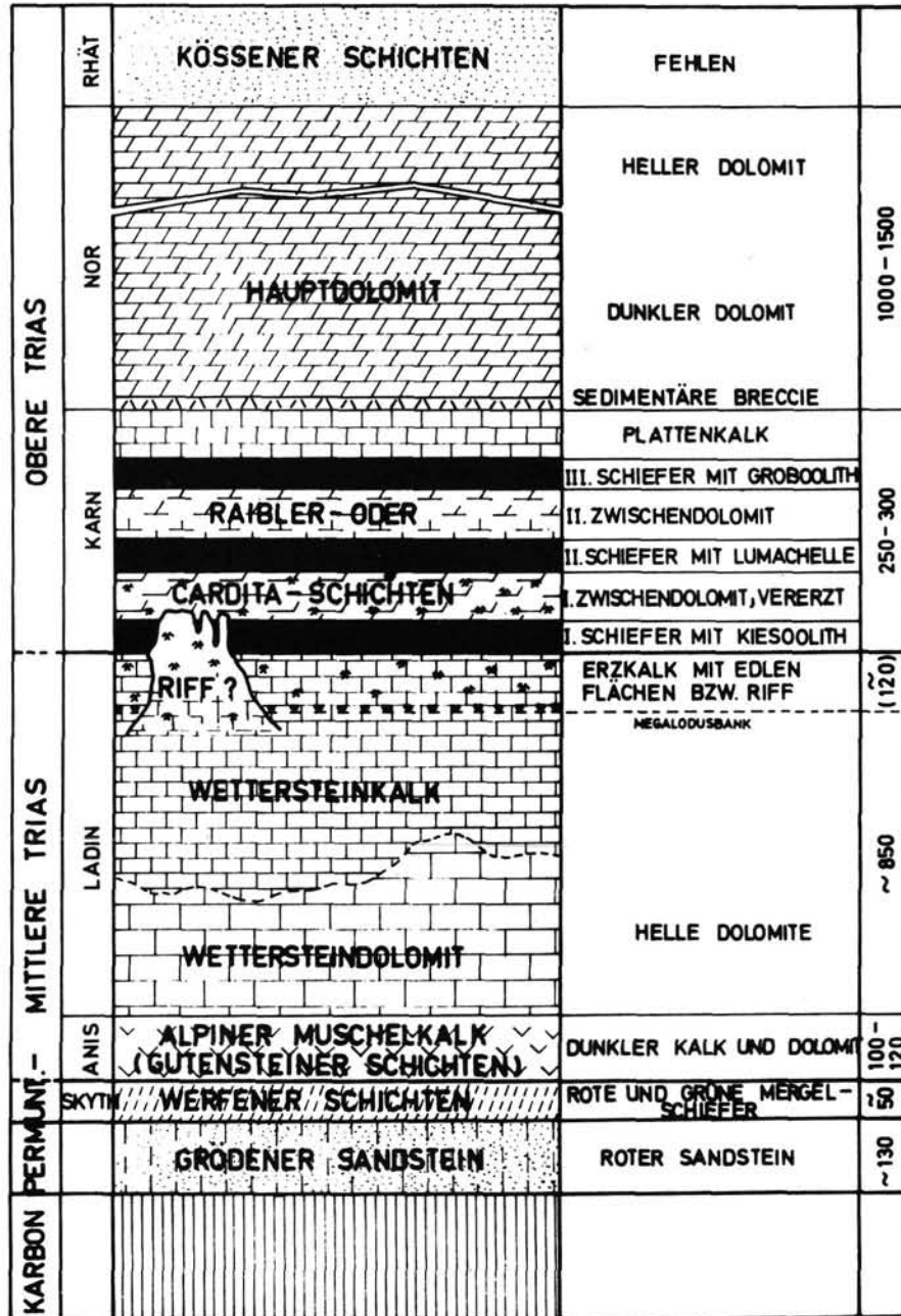
Fig. 9: Stratigraphy of the Triassic in the Bleiberg area (from M. BOUVIER et al., 1972). Crossed hammers indicate mineralized zones.
