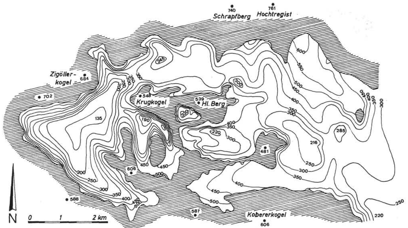
Fig. 2: Map of the pre-Tertiary relief of the lignite basin of Köflach—Voitsberg. After W. POHL, 1976.
