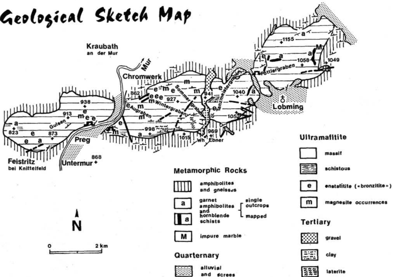
Fig. 5: Geological sketch map of the Kraubath ultramafic massif. After J. G. HADITSCH et al., 1980.
