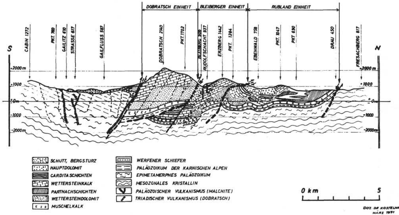
Fig. 10: North-South section from the Drau valley to the Gail valley, illustrating the general geology of the Bleiberg area (from M. BOUVIER et al., 1972). "Schutt, Bergsturz" = gravel, rock slide.
