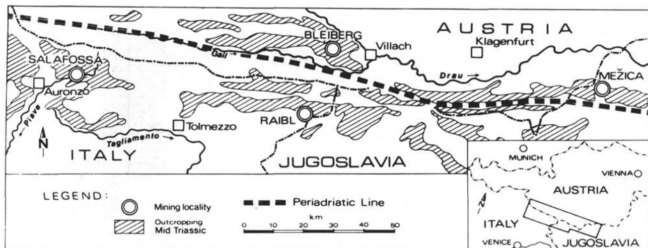
Fig. 8: Location map of the lead-zinc mines of Bleiberg, Méžica, Salafossa and Raibl. From L. BRIGO et al., 1977.
