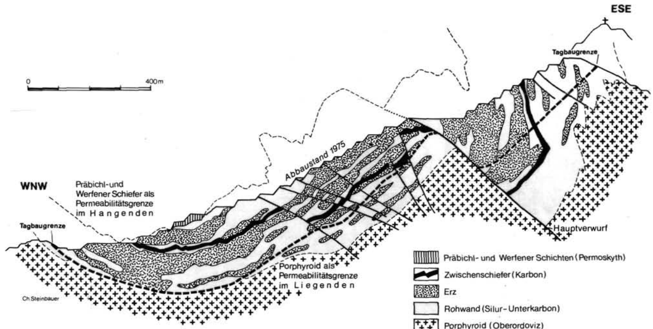
Fig. 4: Cross section through the Erzberg deposit. After Vöest-Alpine Corp.
