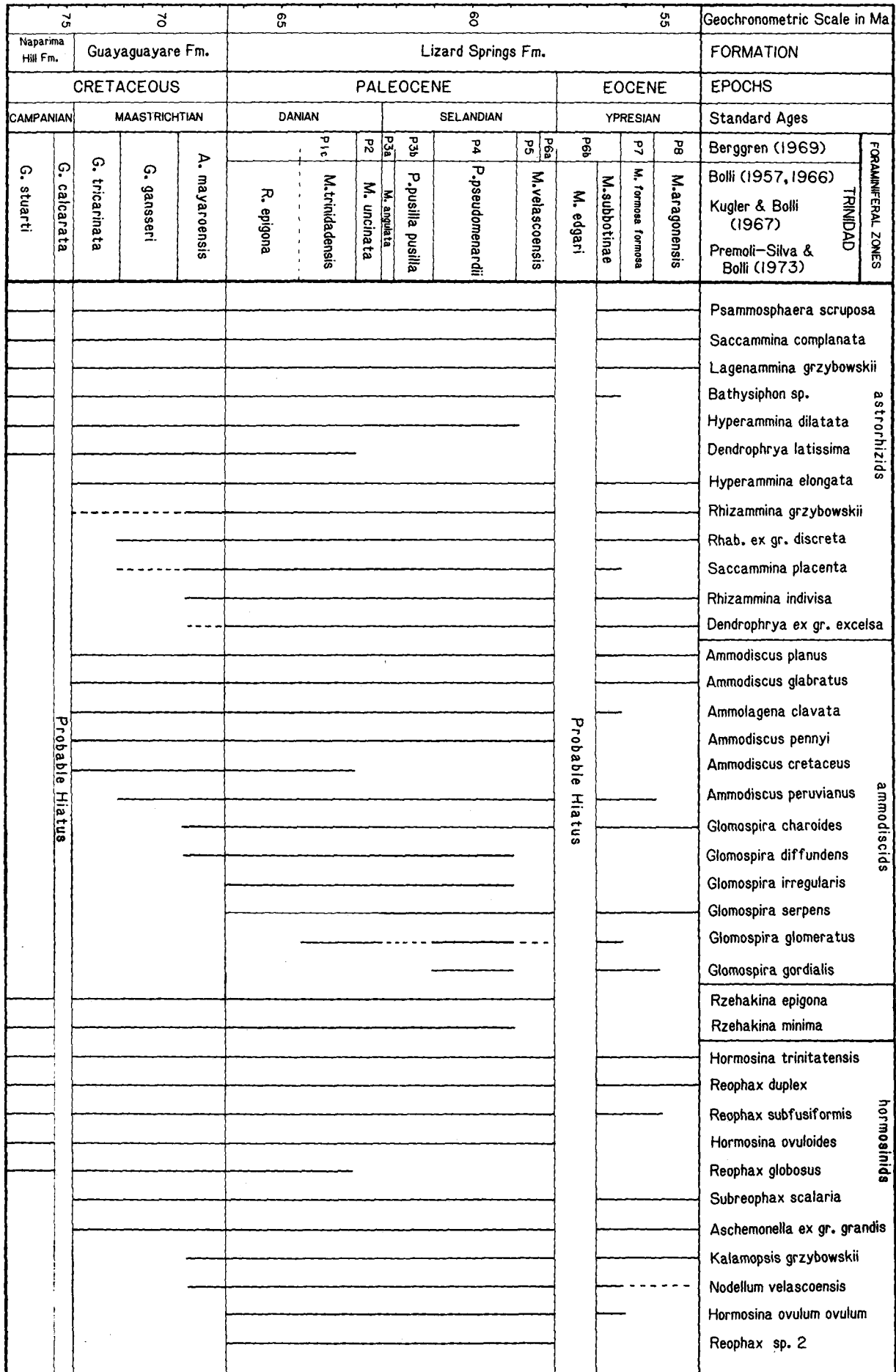
STRATIGRAPHIC RANGE CHART
