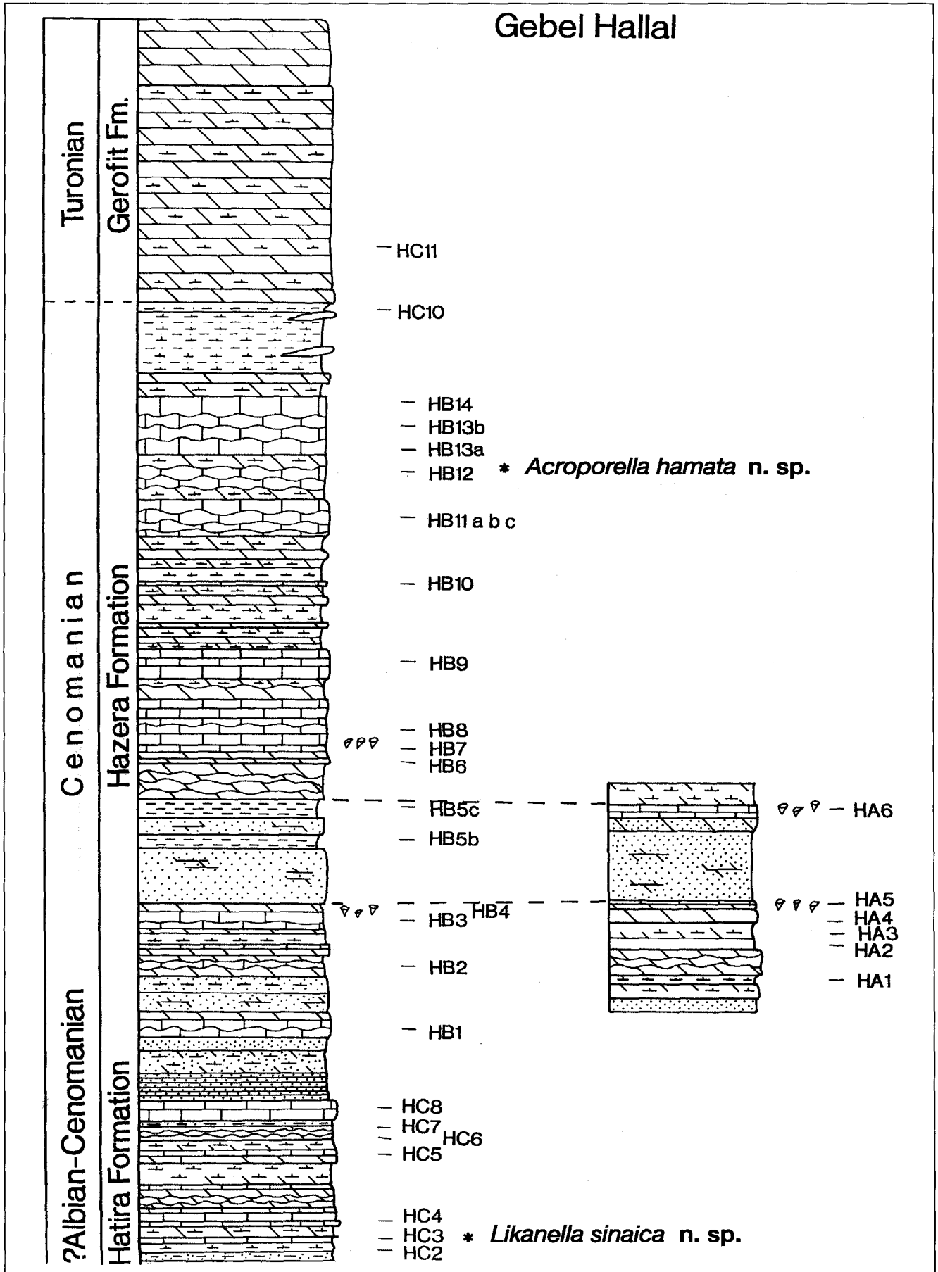
Text-Fig. 3. The Albian-Turonian succession of Gebel Hallal (northern Sinai; see Text-Fig.1). The column is drawn with respect to sample-horizons and occurrences of the new species Acroporella hamata n.sp. and Likanella sinaica n.sp.
