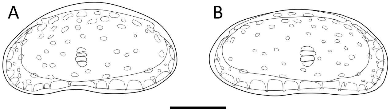
Figure 7. Redekia abyssalis sp. nov., male, holotype (SMF 57056). A RV, internal lateral view B LV, internal lateral view. Scale bar: 100 \mu m.
