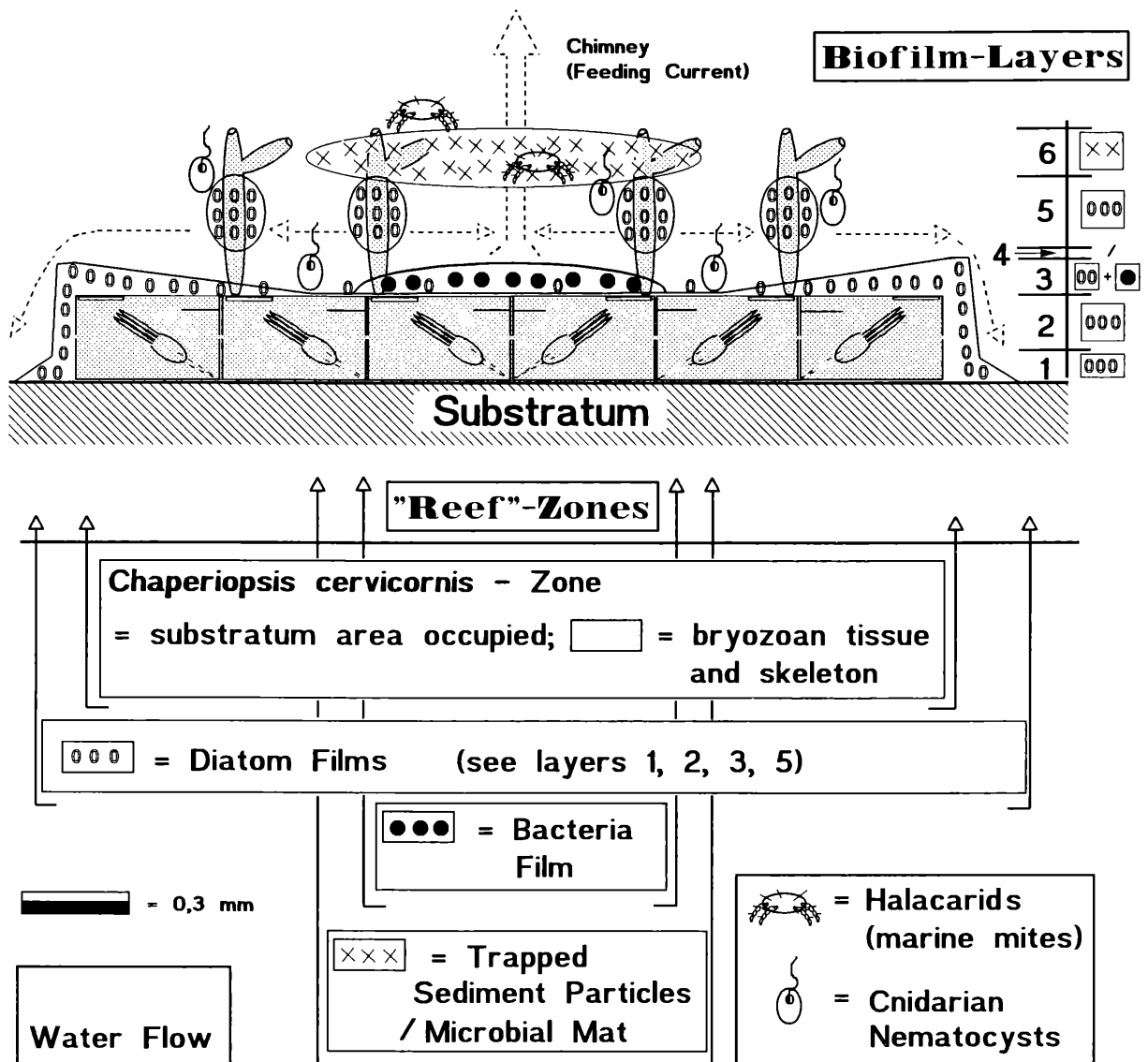
Figure 1: Layering and zonation in a bryozoan micro-reef, compiled from the specimen of Chaperiopsis cervicornis illustrated in Pl. 1 & 2. Each of the layers has a distinct epibiotic microbial community which can be described as follows:
