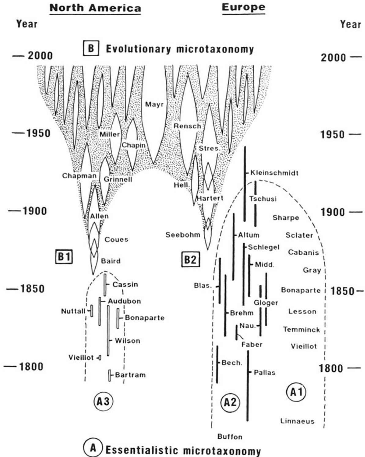
Fig. 33. Research traditions (“schools”) of systematic ornithology during the 19th and 20th centuries. A. Typological (essentialistic) microtaxonomy; A1. Linnaeus school, A2. Pallas-Schlegel school, A3. Wilson school; B. Evolutionary microtaxonomy; B1. Baird-Coues school, B2. Seebohm-Hartert school. The main publishing periods of major ornithologists are indicated symbolically. Most presently active representatives of evolutionary microtaxonomy are indicated anonymously. Bech. – Bechstein, Blas. – J.H. Blasius, Midd. – Middeldorff, Nau. – Naumann, Stres. – Stresemann. (From Haffer 1997a).
