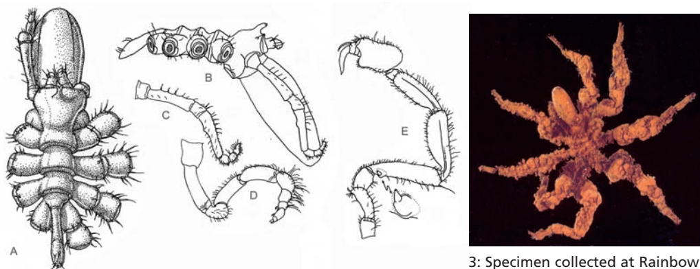
1: Holotype male. A: Trunk, dorsal view; B: Trunk, lateral view; C: Palp; D: Ovipiger; E: Third leg; from CHILD & SEGONZAC (1996).
