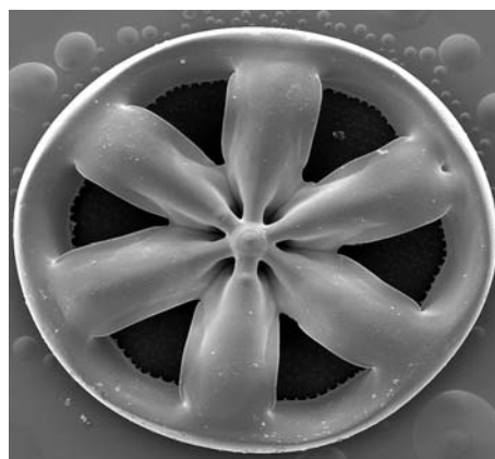
4: Wheel shaped spicules (SEM) © Ifremer.
