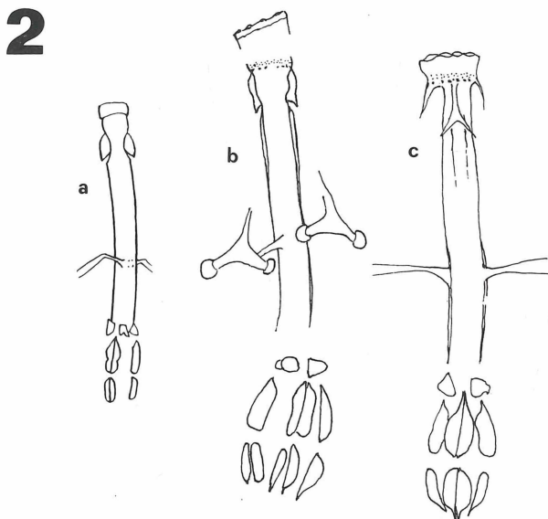
Fig. 2a-c. a - Hysibius , bucco-pharyngeal apparatus (lateral view); b, c - Acutuncus antarcticus (Richters, 1904), bucco-pharyngeal apparatus (b - lateral view, c - ventral view).
