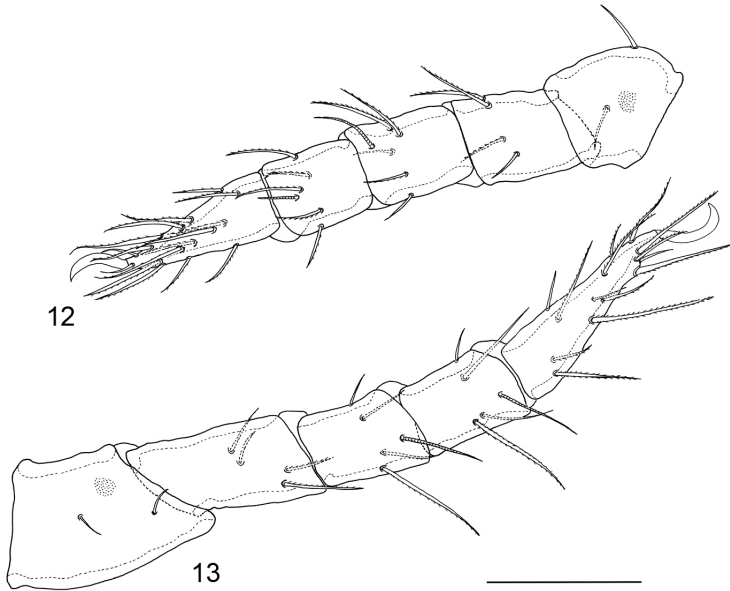
Figs 12-13: Perlohmannia (Perlohmannia) dissimilis (HEWITT) (adult). (12) leg 3; (13) leg 4. Scale bar: 100 \mu\text{m} .
