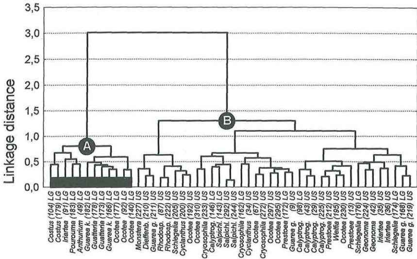
Fig. 6. Cluster dendrogram for two different microsite types, i.e. shady understorey vs. light gaps (design IV in Table 3). Dendrogram based on Sørensen's (1948) coefficient of community and Ward's clustering algorithm. For further explanation see text. US = shady understorey phorophyte, LG = light gap phorophyte.
