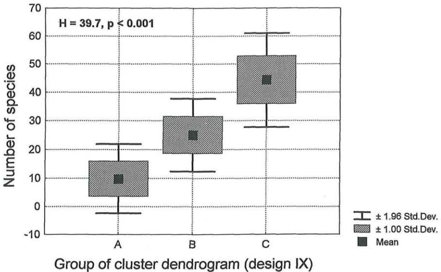
Fig. 12. Box and whisker diagram (Kruskal-Wallis H-test) showing the degree of overlap in foliicolous lichen diversity between the groups defined in the cluster dendrogram of Fig. 11.
