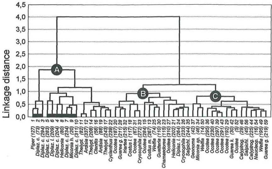
Fig. 11. Cluster dendrogram for phorophytes with continuously increasing foliicolous lichen diversity (design IX in Table 3). Dendrogram based on Sørensen's (1948) coefficient of community and Ward's clustering algorithm. For further explanation see text. The figures behind the phorophytes indicate the number of foliicolous lichen species present on each phorophyte.
