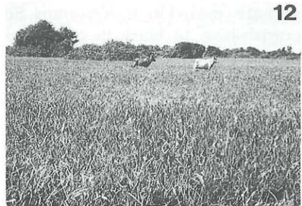
Figs. 7–12. Vegetation of the Pantanal region. – Fig. 7. General aspect of an earthmound savanna with small tussock grassland and (relatively grand) elevated earthmounds. – Fig. 8. Aerial view of an earthmound savanna with Licania -gallery forest in the background. – Fig. 9. Detailed view of an earthmound savanna: small tussock grassland with interspersed (relatively little) earthmounds. – Fig. 10. Same site after being burned, showing the gully and micromound structure of the grassland soil and termite mounds on top of the earthmounds. – Fig. 11. Tall tussock grassland of Andropogon hypogynus with tussocks of A. bicornis interspersed (dense whitish inflorescences). – Fig. 12. Inundated shortgrass floodplain with dominance of Pontederia cordata var. lancifolia .
