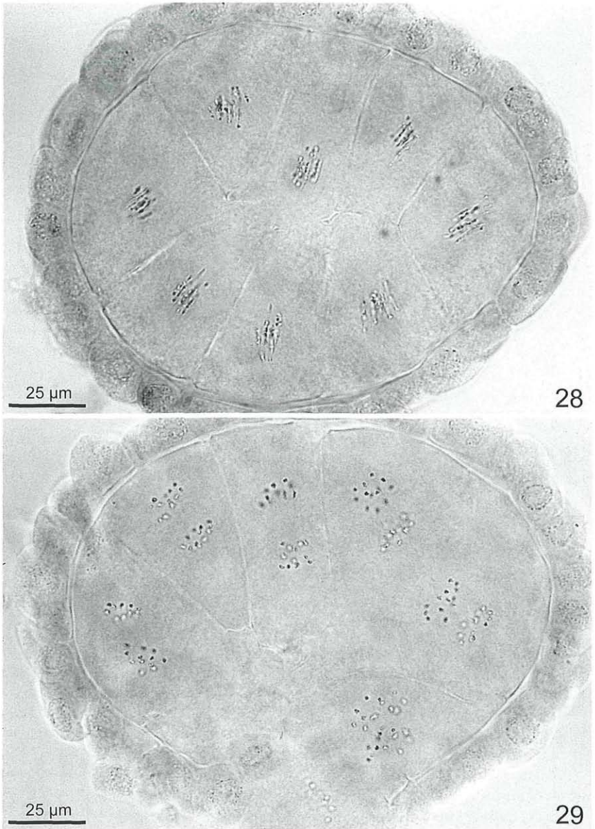
Fig. 28–29. Inga feuillei . Meiosis I. Prepolysads with 8 PMCs with callose in the tapetum-sac, squashed out from the locule-halves. – Fig. 28. PMCs at metaphase I, all spindles more or less parallel to the plane of the prepolysad and radially oriented. – Fig. 29. PMCs at anaphase I, prepolysad a little damaged at the bottom due to squashing. Orientation of the spindles similar to those in Fig. 28, a few a little more oblique (above right).
