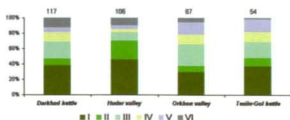
Fig. 3: Species Groups of: I – mires; II – meadow and forest; III – meadow-steppe; IV – dry steppe; V – salt marshes; VI – high mountains and gravel. The figures above the graphs represent the total number of vascular plant species recorded in mires at that site.
