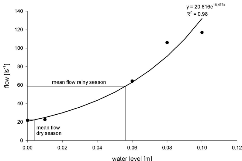
Fig. 12: Measured flow [ \text{ls}^{-1} ] of five different water levels [m] and accounted mean flow [ \text{ls}^{-1} ] of the Q. Negra during the dry and rainy season (based on mean water level for three-month periods).
