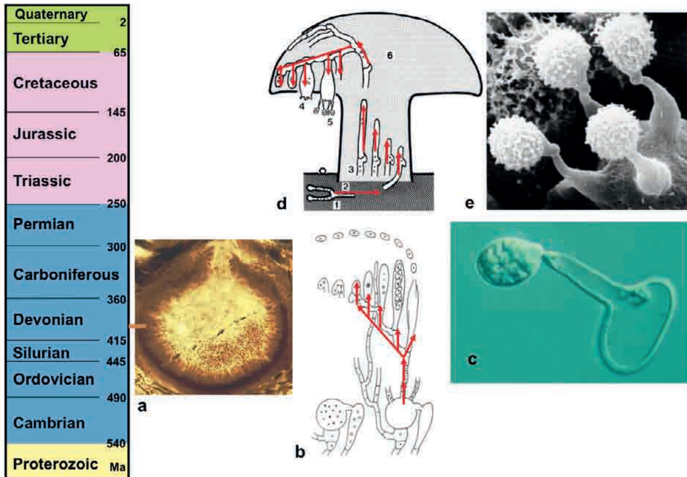
Fig. 4: The dikaryomycotic fungi, Ascomycota and Basidiomycota. a: Fossils of Ascomycota are known from the Devonian. The perithecium is approximately 400 \mu\text{m} in diameter and develops in the stomatal chamber of Asteroxylon . Their morphology is identical with extant representatives. The dikaryophases of typical Asco- and Basidiomycota are illustrated schematically (red arrows). b: In Ascomycetes the dikaryophase is restricted to short hyphae between the ascogon and the asci. d: In the majority of Basidiomycetes the dikaryophase extends to more or less the whole life cycle. e: Ballistospores ejected from sterigmata are typical for basidiomycetous meiosporangia, the basidia. c: A similar mechanism can occur in ballistosporous yeasts of Basidiomycetes. a from TAYLOR et al. (1999). Orig. F. OBERWINKLER.
