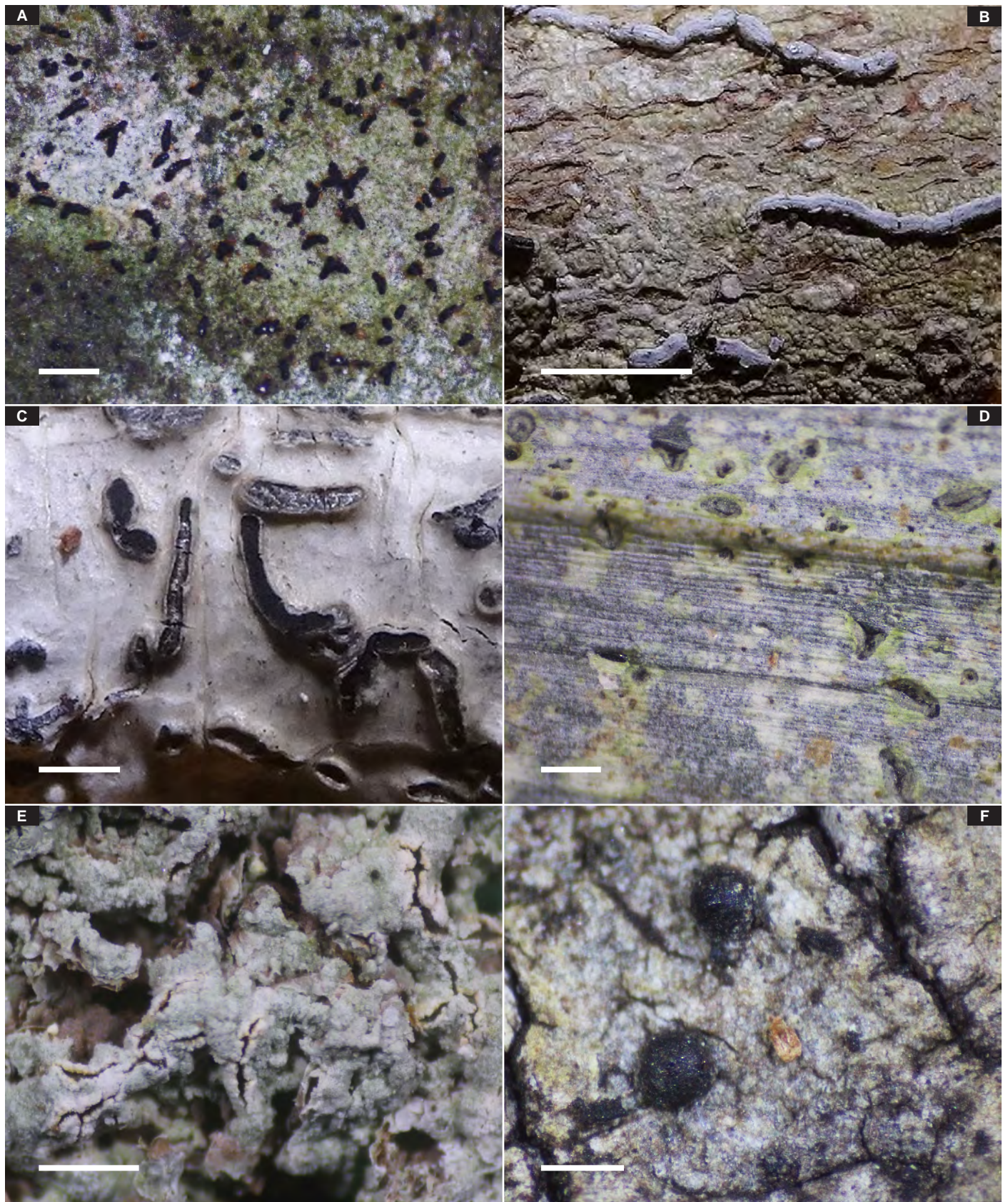
Fig. 1: Habitus and ascomata of species. A – Arthonia orbyniae ; B – Carbacanthographis marcescens ; C – Leiorreuma hypomelae-num ; D – Fouragea viridistellata ; E – Thalloloma janeirense ; F – Bogoriella miculiformis . Scale bars: A=0.5 mm, B=3 mm, C=2 mm, D=0.2 mm, E=2 mm, F=0.3 mm.
