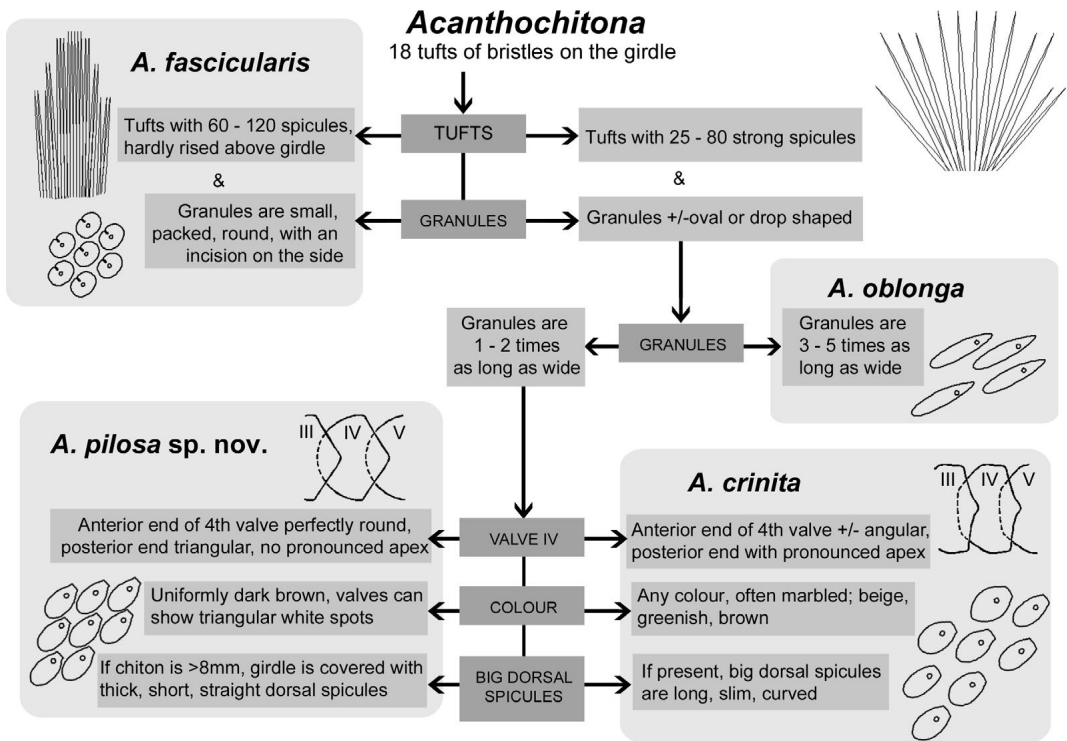
Fig. 6. Illustrated key to the Acanthochitona of the Mediterranean Sea. Key is based on external, macroscopic morphological features.
