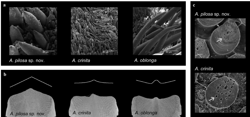
Fig. 5. Morphological differences between A. pilosa spec. nov., A. crinita and A. oblonga (SEM). a. Section of the dorsal part of the girdle (perinotum), scale bar: 50 µm. b. Posterior shape of valve IV. c. Granule with macro- and microaesthetes.
