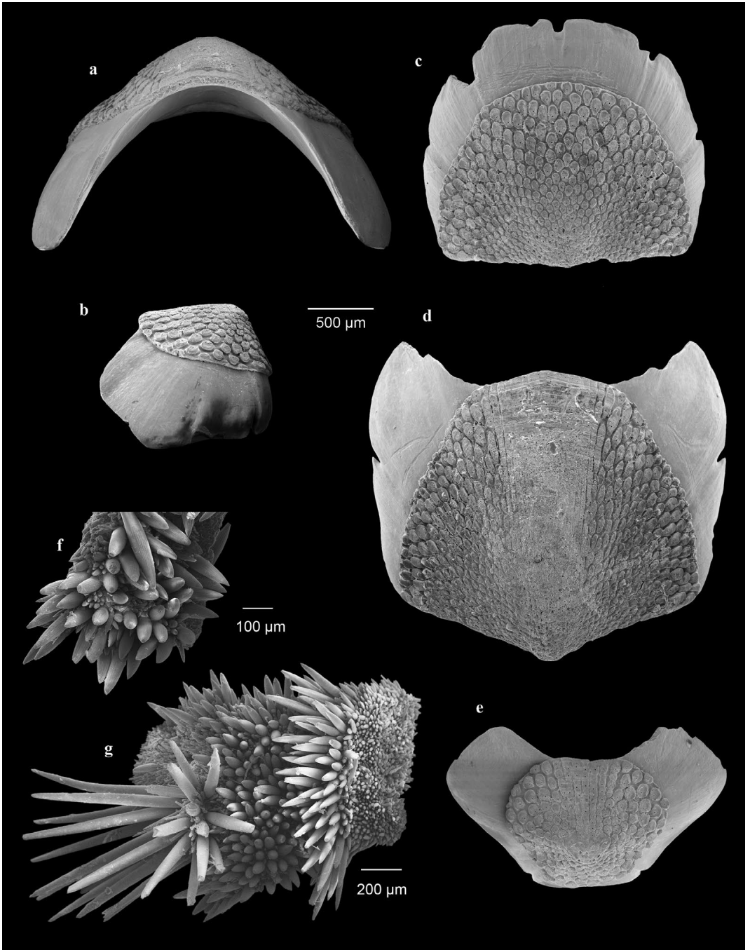
Fig. 2. Valves and girdle elements of the holotype of Acanthochitona pilosa spec. nov. (ZSM Mol 20070223) body length 13 mm (SEM). a. Frontal view of valve II. b. Lateral view of tail valve. c. Dorsal view of head valve. d. Dorsal view of valve II. e. Dorsal view of tail valve. f. In situ spicules of the perinotum. g. Section through the girdle showing from left to right a tuft, mid-girdle (perinotum) spicules, marginal fringe, and hyponotum spicules. Scale bar: 50 µm for a-e.
