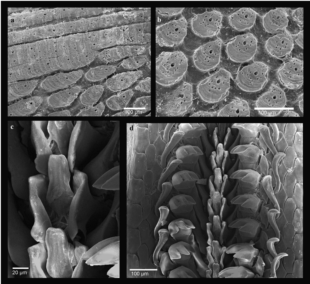
Fig. 3. Radula and tegmentum sculpture of the holotype of Acanthochitona pilosa spec. nov. (SEM) (ZSM Mol 20070223). a. Dorsal view of valve II junction of jugal area and pleurolateral area. b. Detail of pleurolateral area of valve II, showing the aesthete arrangement. c. Detail of central tooth and first lateral teeth. d. Anterior portion of radula.
