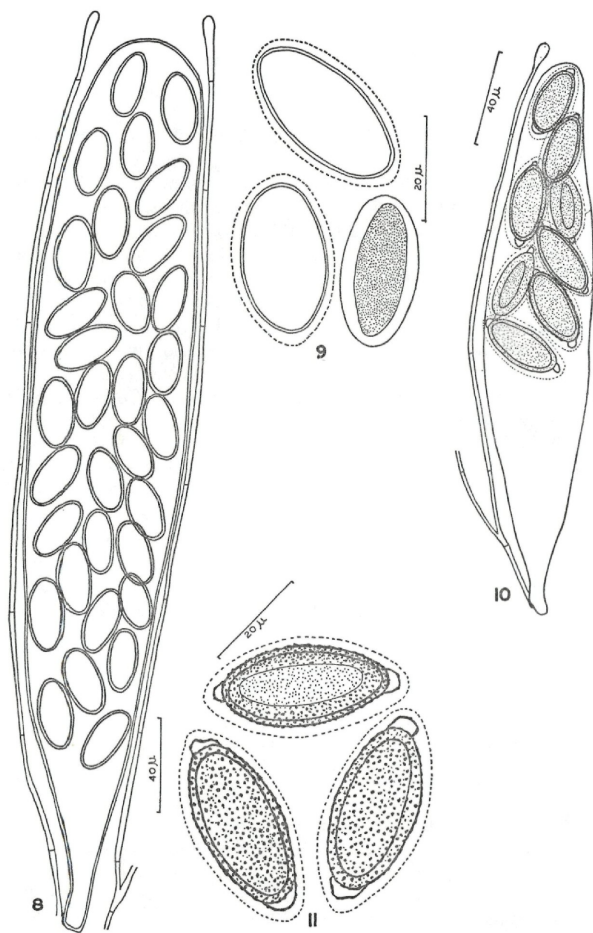
Figs. 8—11. Thecotheus pelletieri . 8. Cylindric-clavate and 32-spored ascus and paraphyses. 9. Large-sized ascospores covered with a mucilaginous perisporic covering. T. holmskjoldii . 10. Broad-clavate and 8-spored ascus, and filiform paraphysis with capitate tip. 11. Large-sized apiculate ascospores with fine granules and covered on the outside with mucilaginous perisporic sheath.
