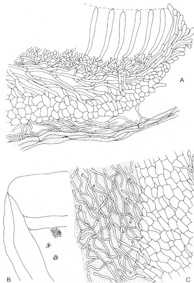
Fig. 7: Rodwayella citrinula . A. Vertical section of margin and upper receptacle, \times 700 . - Skyatheia hederarum : B. Diagrammatic vertical section of margin to show arrangement of tissues, \times 120 . - C. Ectal excipulum near margin, \times 700 .
