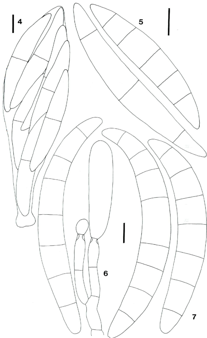
Figs. 4-7. - Nectria fusispora . - 4. Ascus with developing ascospores. - 5. Two discharged ascospores. - 6, 7. Cyliandrocarpon fusisporum anamorph. - 6. Conidiogenous cells. - 7. Macroconidia. - Figs. 4 from KPD-CO 5297, 5 from KPD-2101. - Scale bars = 10 \mu m.
