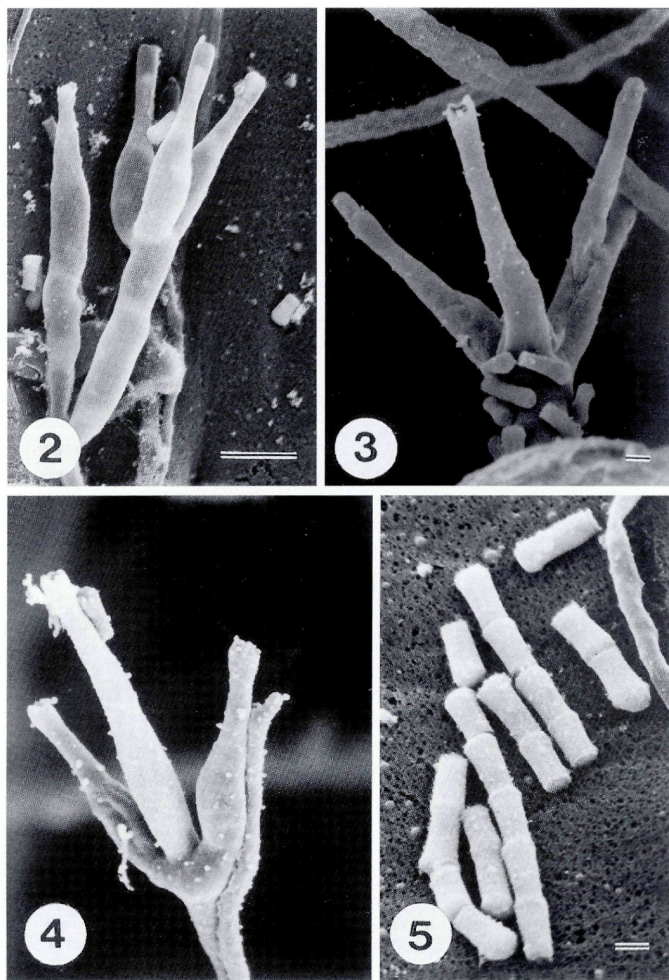
Figs. 2-5. - Scanning electron micrographs of Sporendocladia fumosa . - 2. conidiophore with phialides showing apical wall conidial development (bar = 5 μm). - 3, 4. conidiophores with phialides showing tubular collarettes and cuneiform conidia (bar = 1 μm). - 5. cuneiform conidia in false chains with thickened basal hila, indicating basal dehiscence scars (bar = 1 μm).
