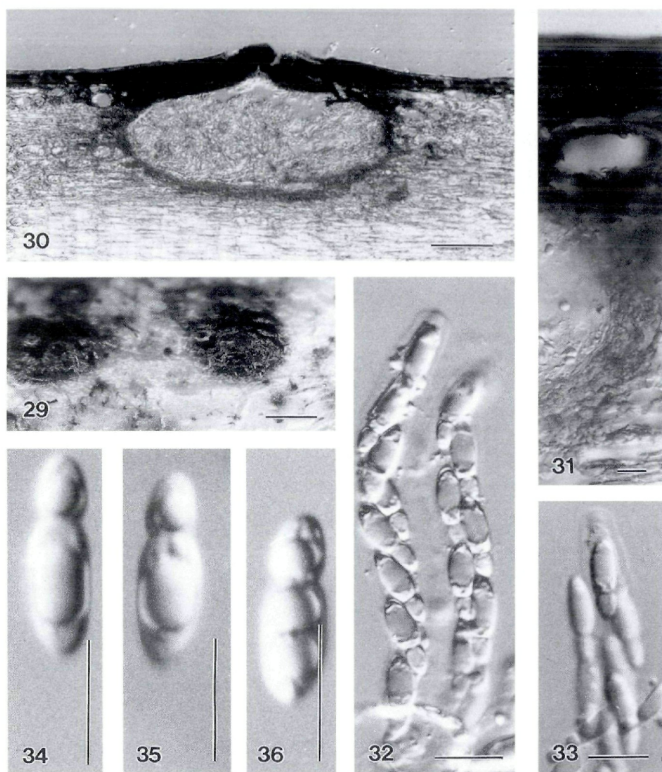
Figs. 29–36. Apioctypha indica [from HKU(M) JF509]. – 29. Appearance on host surface. – 30. Section of ascoma. – 31. Peridium. – 32, 33. Asci. – 34–36. Ascospores. – Bars: 29 = 500 \mu\text{m} , 30 = 100 \mu\text{m} , 31–36 = 10 \mu\text{m} .
