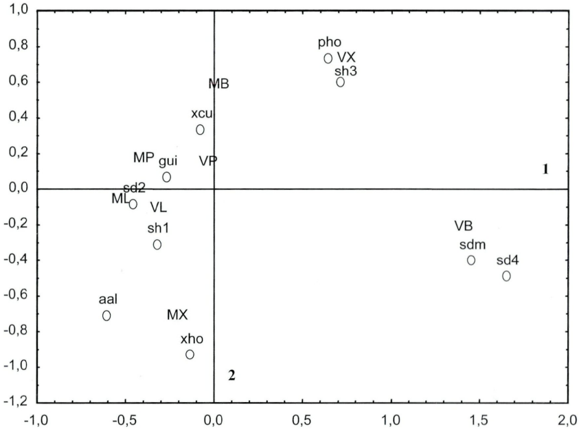
Fig. 1. – Simple correspondence analysis. Ordination of twigs and leaves from Mato Leitão and Veranópolis on the two first axes. Total inertia explained by the first three co-ordinates: 82 %. Variables are the relative frequencies of isolation of species with frequency equal or higher than 5%.—Symbols for the species are indicated in Table 1; M, Mato Leitão; V, Veranópolis; P, main vein and petiole; B, bark; X, xylem.
