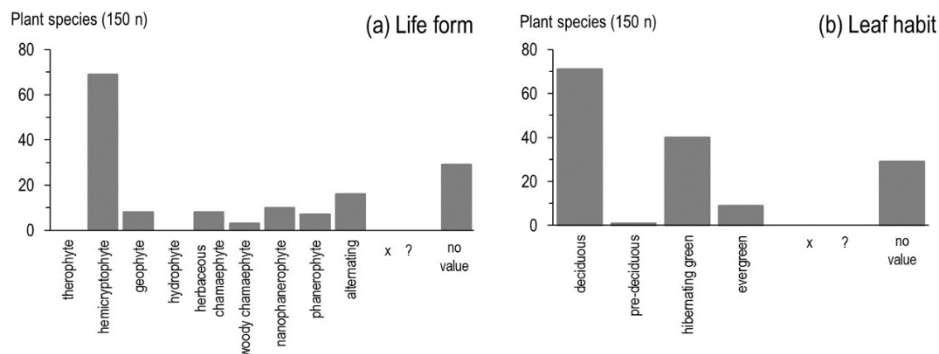
Fig. 4. a) Life form and b) leaf habit according to ELLENBERG et al. (2001) for the 150 plant species from the Kazbegi-Bakuriani database which have at least ten German suppliers in the PPP-Index. 'alternating' = alternating life form with site conditions, x = indifferent, ? = unclear, 'no value' = species not listed in ELLENBERG et al. (2001).
