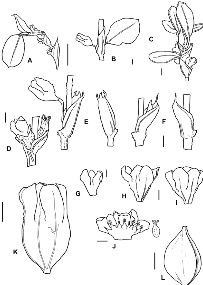
Figure 7. Morphological characteristics of P. cognatum (A, B, G, J, K), P. serpyllaceum (C, D, H, L) and P. myrtillofolium (E, F, I). A – fragment of the shoot; B – leaf with ochrea; C – fragment of the shoot; D – ochrea with axillary flower; E, F – ochrea with axillary flower; G – flower bud; H, I – flower; J – flower, cut open; K – perianth in fruiting stage; L – mature achene. Scale bars: A = 10 mm; B–L = 1 mm.
