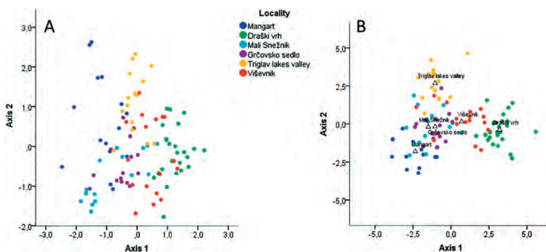
Figure 3. A – Principal components analysis of Nigritella miniata localities from the Julian and Dinaric Alps based on 18 morphological characters (Table 1). Axes 1 and 2 explain 50.79% and 12.13% respectively of the total variation. B – Discriminant function analysis of Nigritella miniata localities from the Julian and Dinaric Alps based on 18 morphological characters (Table 4). Axes 1 and 2 explain 55.70% and 22.30% respectively of the total variation.
