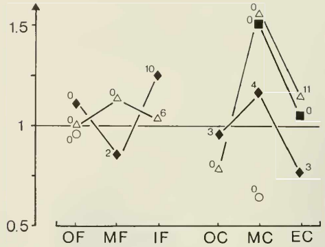
Fig. 17: Right-left valve ratio among shells of the target genera Dosima (○), Chione (◆), Tagelus (△), and Protothaca (■). Figures refer to percentage of articulated shells. For remaining key see Fig. 3.
