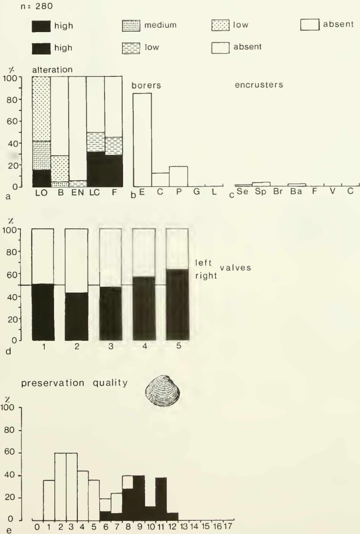
Fig. 23: Taphonomic features of shells of target genera from the beachrock. For key see Fig. 22. a: degree of alteration of shells; b: percentage of shells bored; c: percentage of shells encrusted; d: right-left valve ratio; 1 = Dosinia ponderosa ; 2 = Protothaca grata ; 3 = Chione fluctifraga ; 4 = Chione californiensis (Recent); 5 = Chione californiensis (Pleistocene). e: preservation quality of Chione . White: all Chione ; black: Pleistocene Chione .
