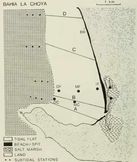
Fig. 2: Map of Bahía la Choya showing sampling stations for the target genera and location of the four transects (A–D). Dotted: desert; stippled: salt marsh; black: spit; stippled line: spring low tide mark. OF: outer flat; MF: mild flat; IF: inner flat; OC: outer channel; MC: mid channel; EC: estero channel; P: Pleistocene locality discussed in the text; BR: beachrock.
