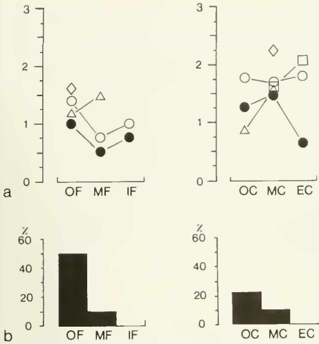
Fig. 4. a: Index of loss of ornament of various target genera in the sub-environments; b: percentage of Cerithium shells inhabited by hermit crabs. ○ = Chione ; ● = Tagelus ; ◇ = Dosinia ; △ = Cerithium ; □ = Protothaca . For additional key see Fig. 3.
