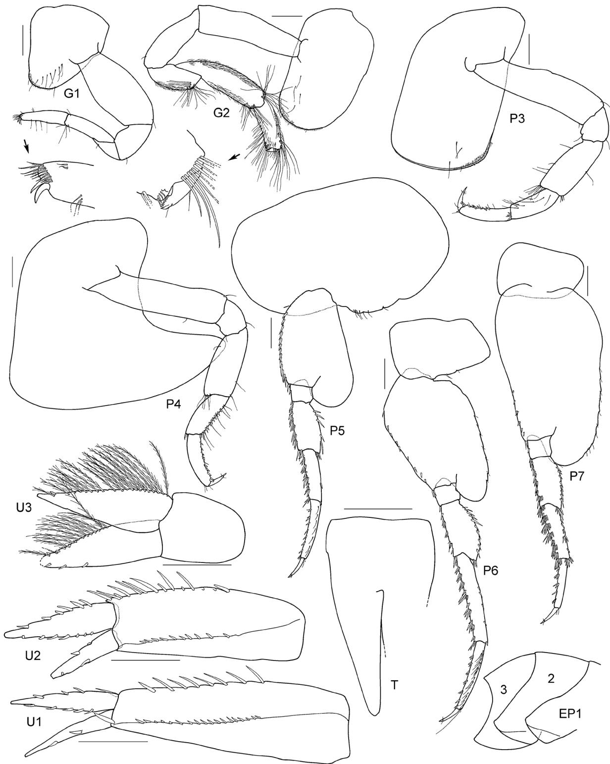
Figure 16. Austrocallisoma jerryi sp. n., holotype, female, 32.0 mm, AM P.69087, from east of Sydney, New South Wales, Australia. Scales represent 0.5 mm.
