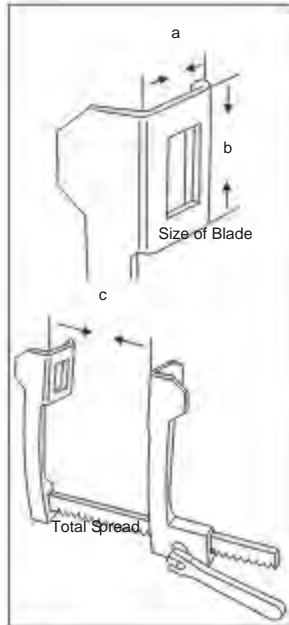
Scheme of Dimension
