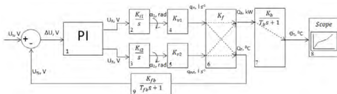
Figure 2. Block diagram of an automatic control system: 1) PI controller; 2) electric motor for furnace flue gasses valve; 3) electric motor for air inlet valve; 4) furnace flue gasses control valve; 5) air inlet control valve; 6) furnace; 7) boiler; 8) monitoring unit; 9) flue gasses measuring unit.
