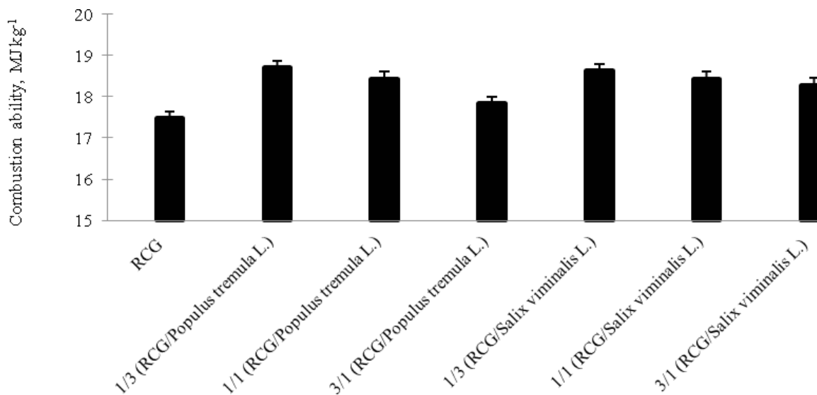
Figure 3. Combustion ability in pellets with different component proportions.
