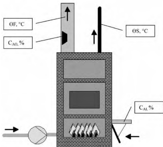
Figure 1. Tests monitoring setup.
