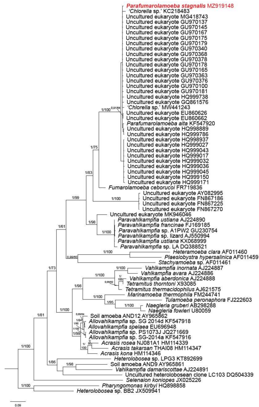
Figure 4. Bayesian phylogeny of the SSU rRNA gene. Bayesian posterior probabilities and Maximum Likelihood (TIM2+F+R4 model) bootstrap values are indicated at branches (values >0.9/>60 are shown; dt—different topology). Pharyngomonas kirbyi HQ898858 SD1A and Heterolobosea sp. BB2 JX509941 were used as the outgroup.
