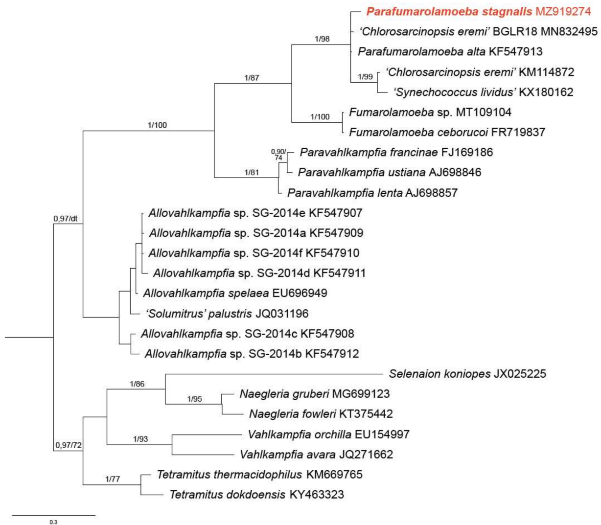
Figure 5. Bayesian phylogeny of the internal transcribed spacer (ITS) region. Bayesian posterior probabilities and Maximum Likelihood (TN+F+G4 model) bootstrap values are indicated at branches (values >0.9/>70 are shown; dt—different topology).
