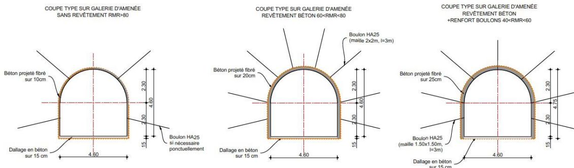
Figure 6 - Typical sections of the feeder tunnel for certain types of land
