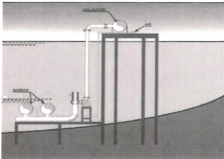
Figure 6 – Wedgewire Screen Intake of Beckton Desalination Plant
