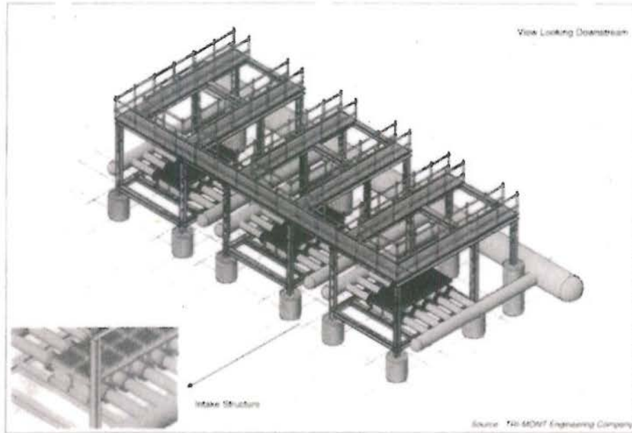
Figure 14 – Taunton River Desalination Plant Intake
