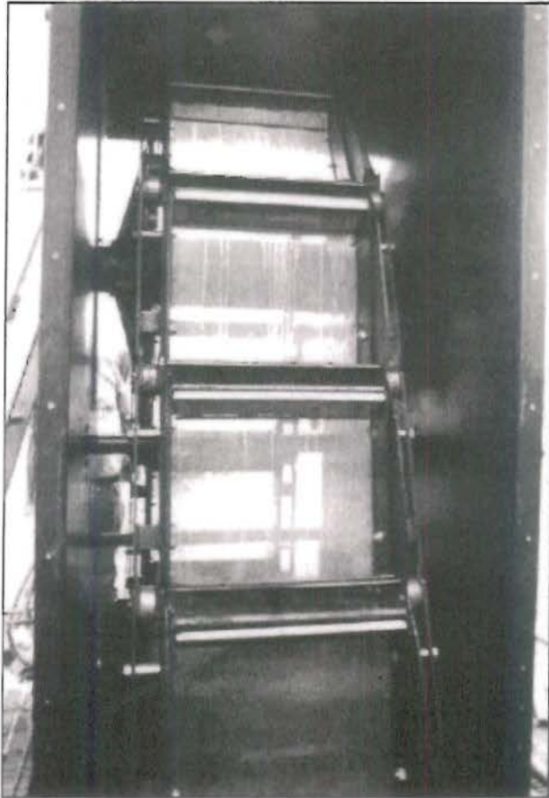
Figure 13 – 0.5 mm Fine Mesh Screens of the Tampa Bay Power Plant Intake
