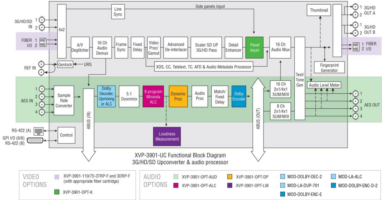
Figure 1.5 Functional block diagram XVP-3901-UC
