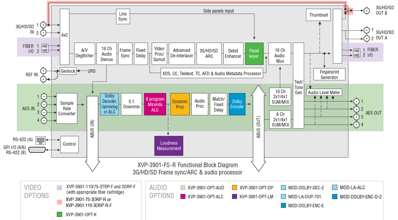
Figure 1.3 Functional block diagram XVP-3901-FS-R
