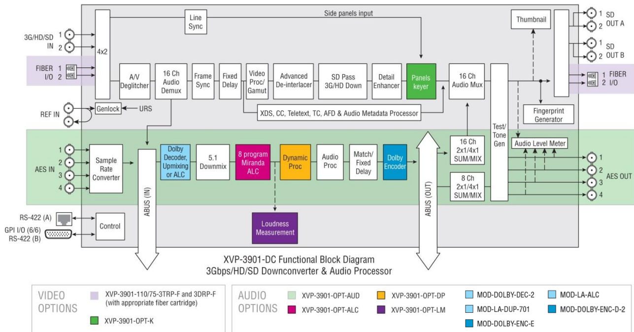
Figure 1.4 Functional block diagram XVP-3901-DC
