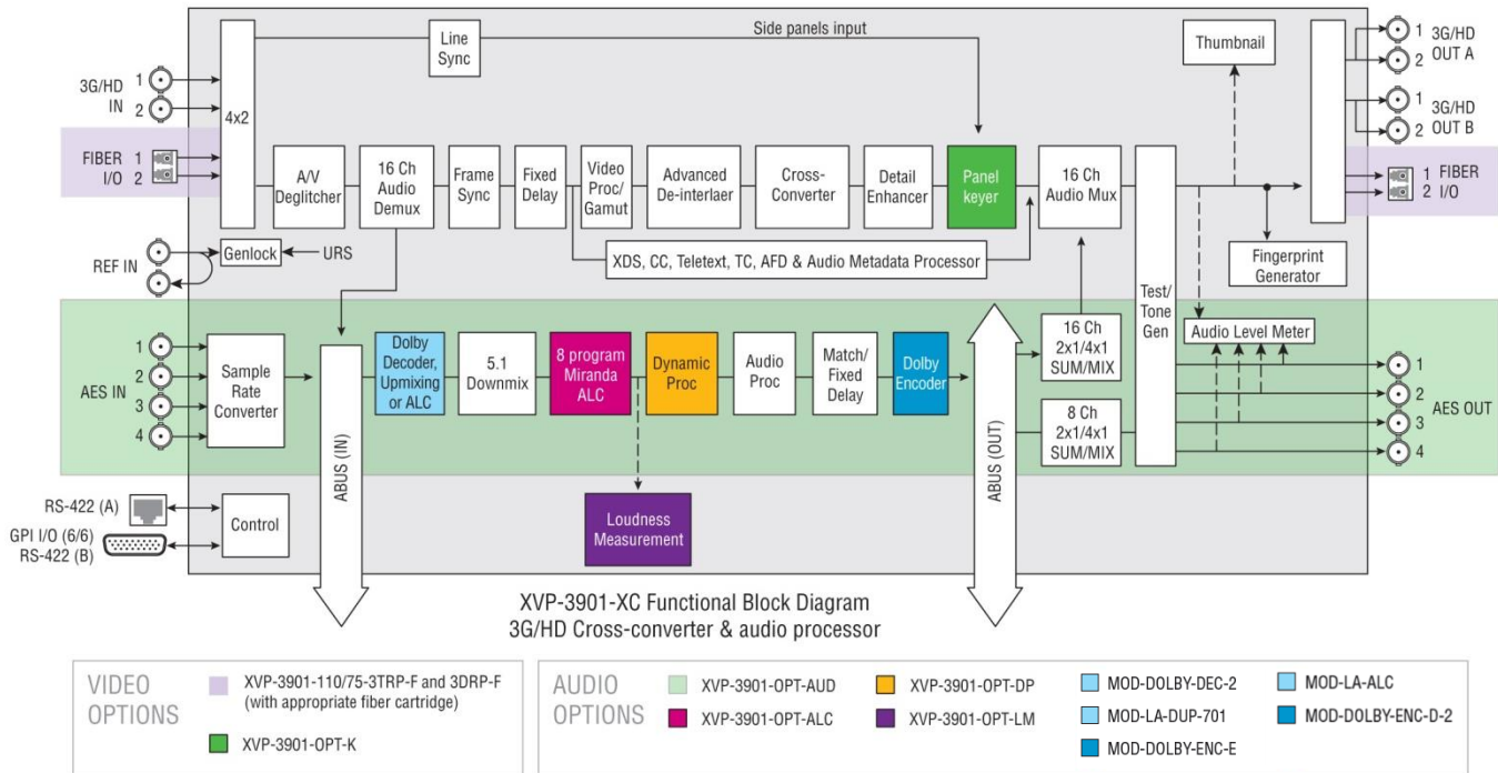
Figure 1.6 Functional block diagram XVP-3901-XC
