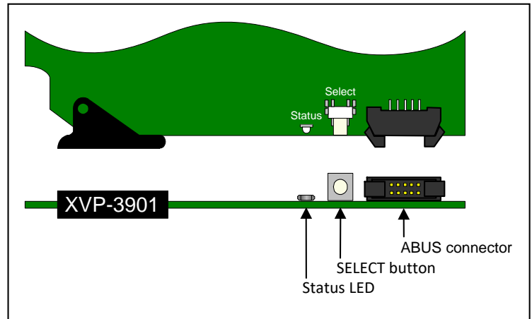
Figure 1.7 Front card-edge layout
