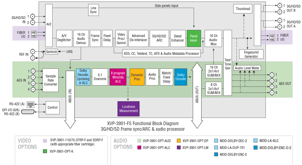
Figure 1.2 Functional block diagram XVP-3901-FS
