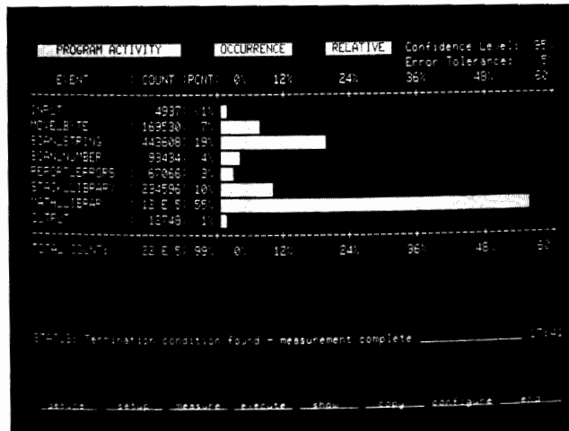
HP 64310A Software Performance Analyzer brings performance analysis measurements to design applications for microprocessor-based products. Six measurements quickly characterize total system performance, allowing the software designer to allocate available resources optimally.
