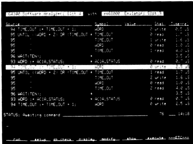
The HP 64340 Real-time, High-level Analyzer Trace Statements Measurement displays executed source lines along with the values of all variables referenced. A hierarchy of measurements streamline troubleshooting from a global view of module execution down to the detail of variable values.
